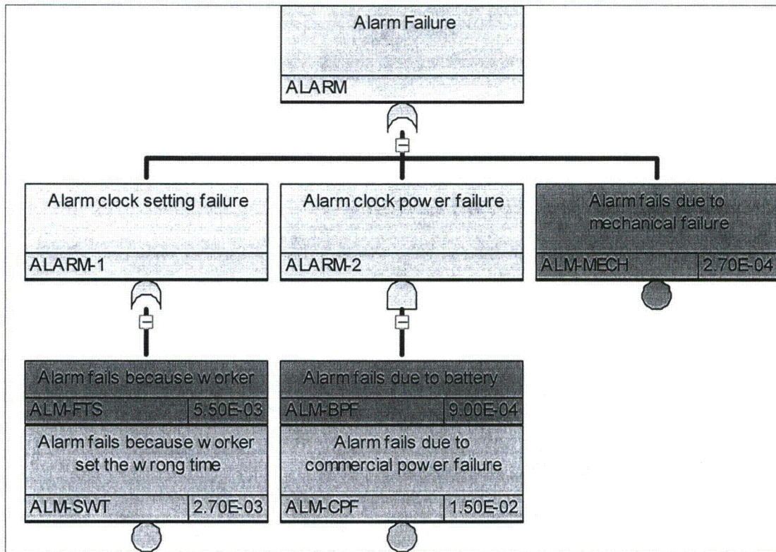
Figure 2. Alarm clock failure fault tree
