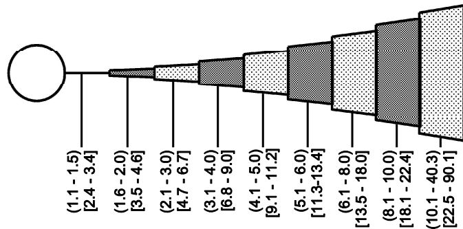
Figure 3.6-16 Rev. 2 EBR September Wind Rose (10 Meters/33 Feet) EAGLE ROCK ENRICHMENT FACILITY ENVIRONMENTAL REPORT
