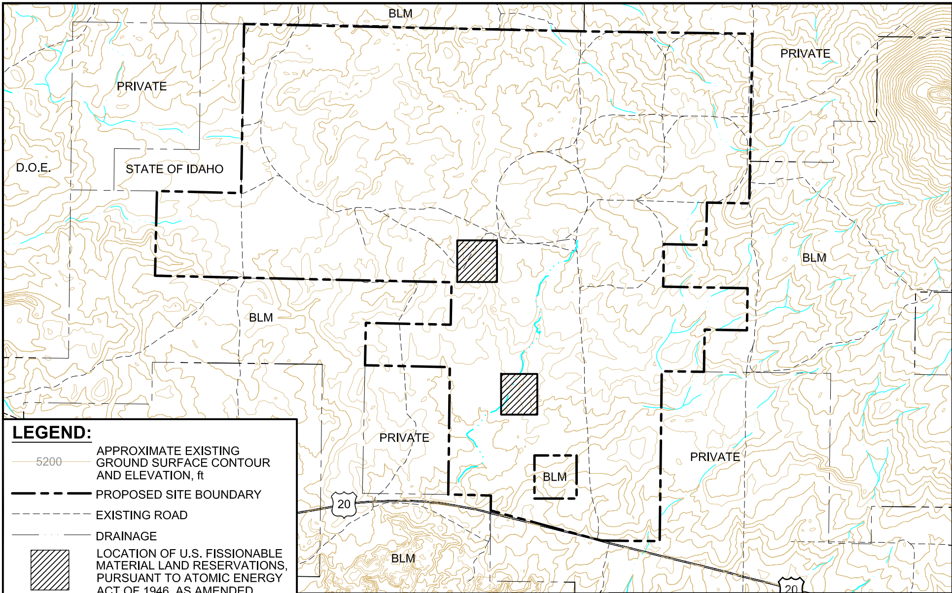
Figure 3.1-2 Rev. 2 Location of U.S. Fissionable Material Land Reservations, Pursuant to Atomic Energy Act of 1946, as Amended EAGLE ROCK ENRICHMENT FACILITY ENVIRONMENTAL REPORT
