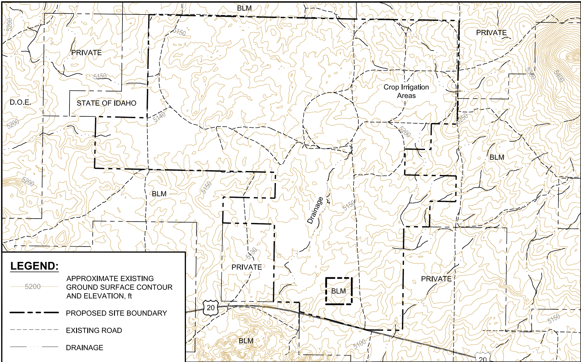
Figure 3.3-8 Rev. 2 Topography, Roads and Drainage EAGLE ROCK ENRICHMENT FACILITY ENVIRONMENTAL REPORT
