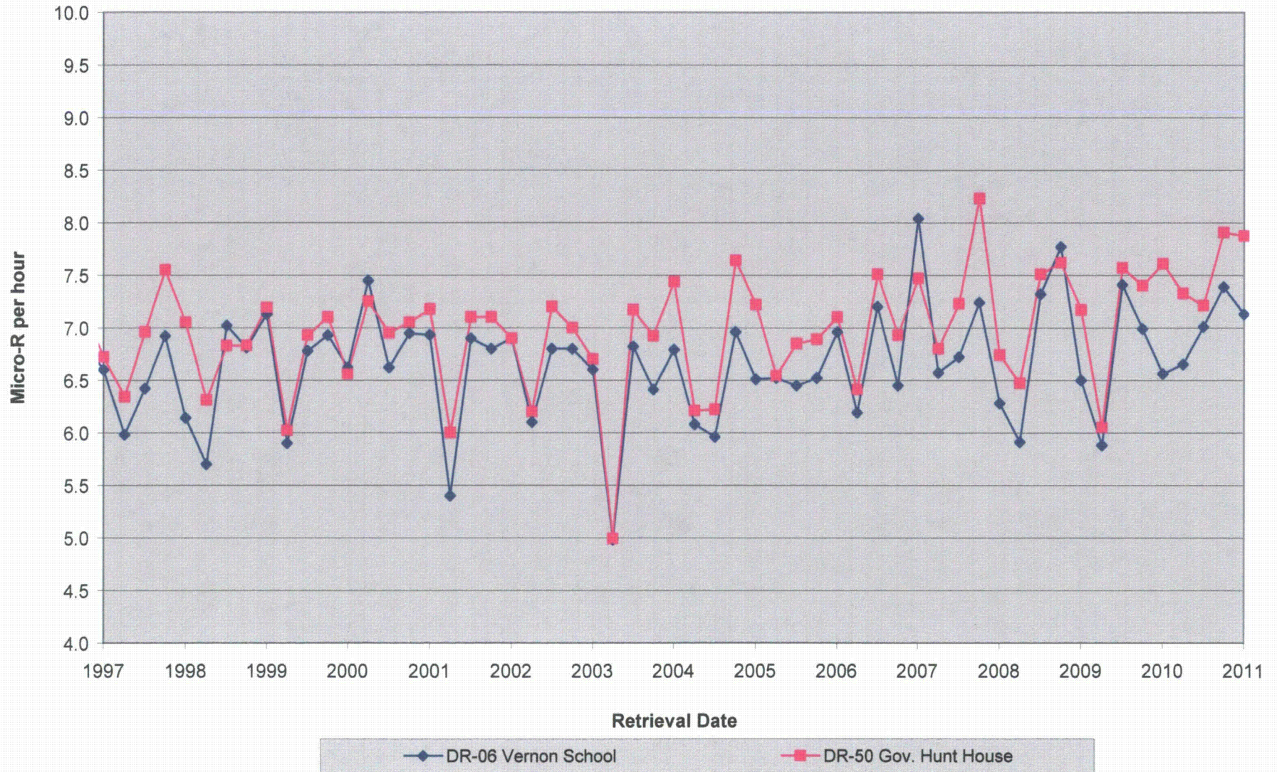
Figure 6.15 - Exposure Rate at Indicator TLDs, DR06 & DR-50
