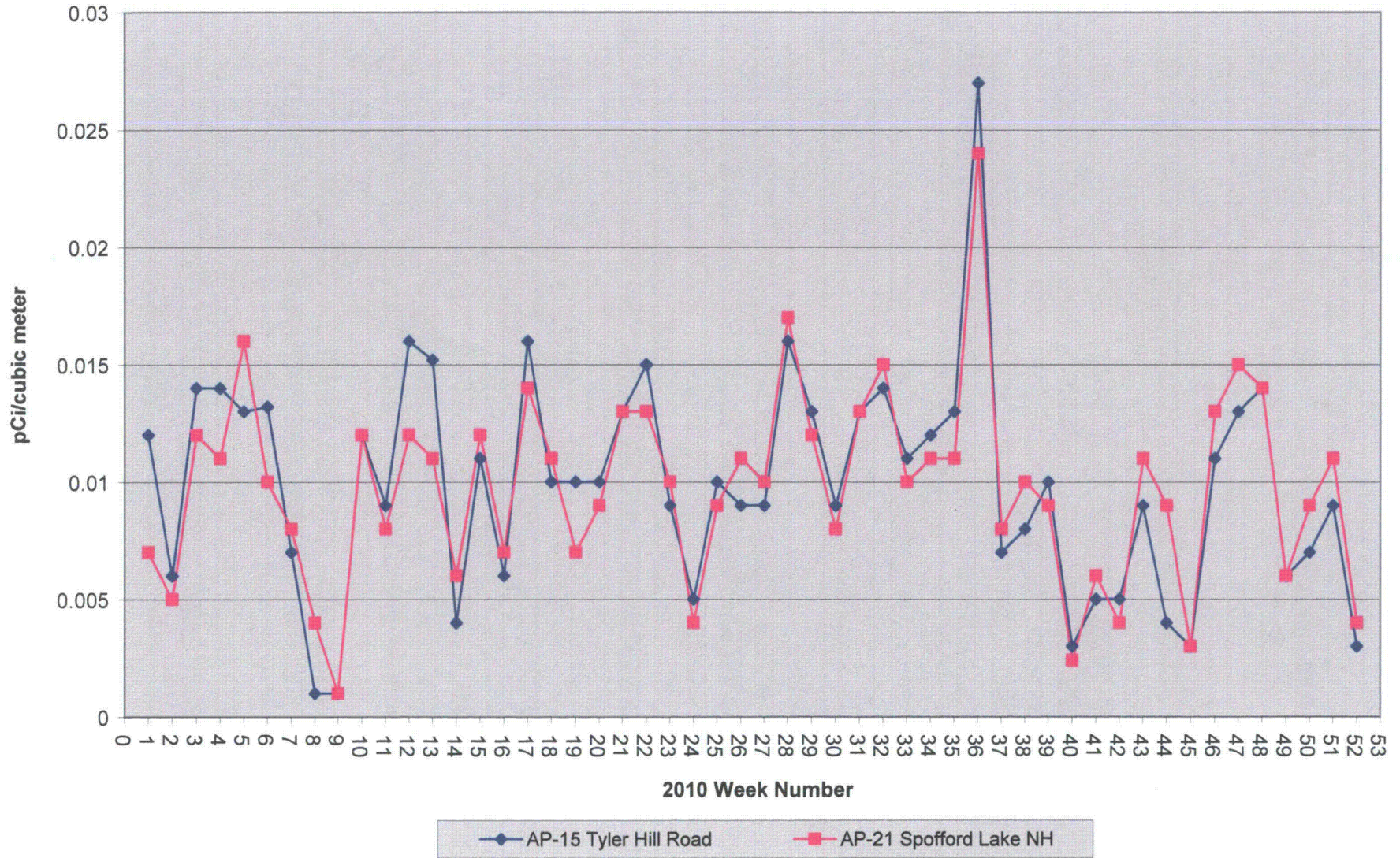
Figure 6.6 - Gross Beta Measurements on Air Particulate Filters
