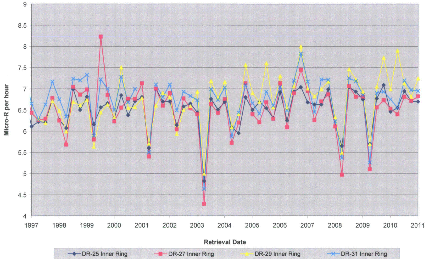
Figure 6.21 - Exposure Rate at Inner Ring TLDs DR25, 27, 29 & 31
