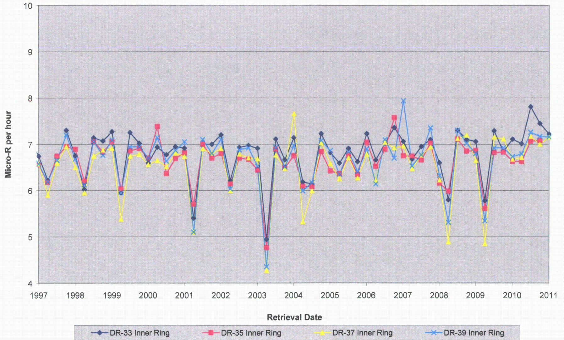
Figure 6.22 - Exposure Rate at Inner Ring TLDs DR33, 35, 37 & 39
