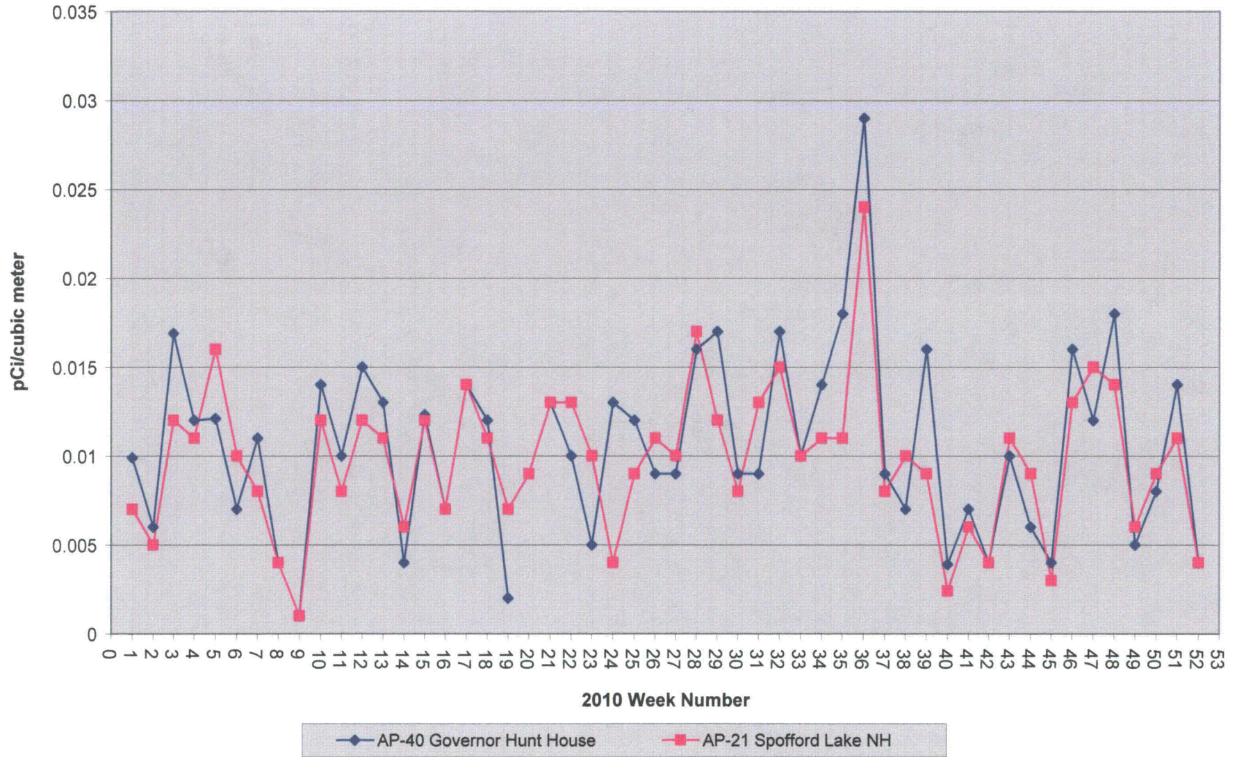
Figure 6.7 - Gross Beta Measurements of Air Particulate Filters
