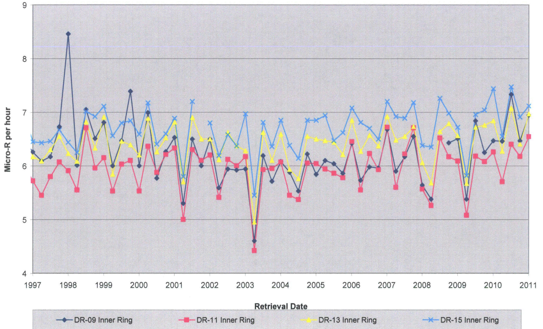
Figure 6.19 - Exposure Rate at Inner Ring TLDs DR09, 11, 13 & 15
