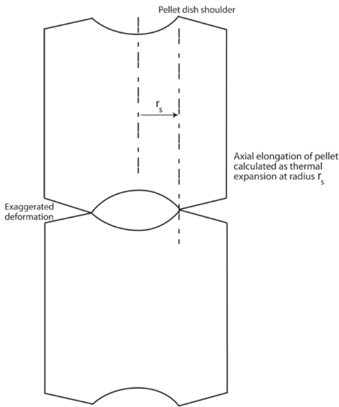
Figure 2.16 Axial thermal expansion using FRACAS-I
