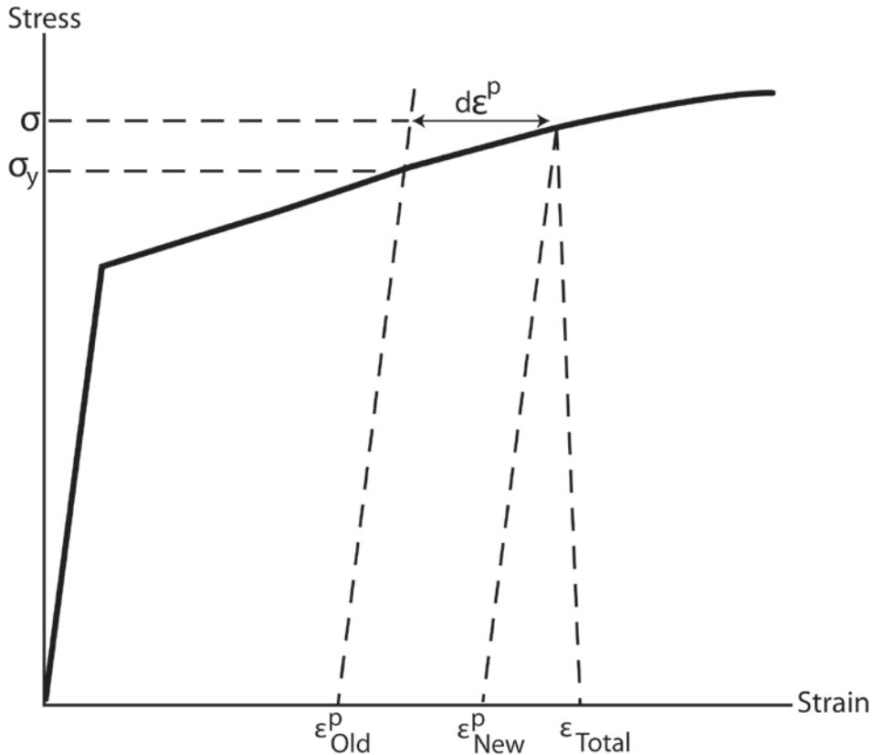
Figure 2.15 Computing stress
