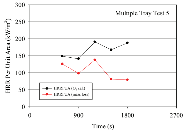
Figure 8-6. Multiple Tray Experiment 5
