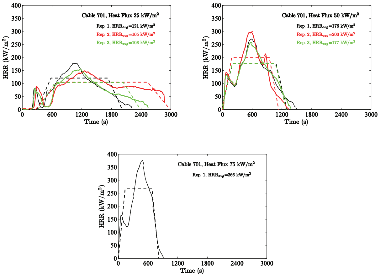
Figure 6-43. Heat Release Rates for Cable #701 in the Cone Calorimeter.
