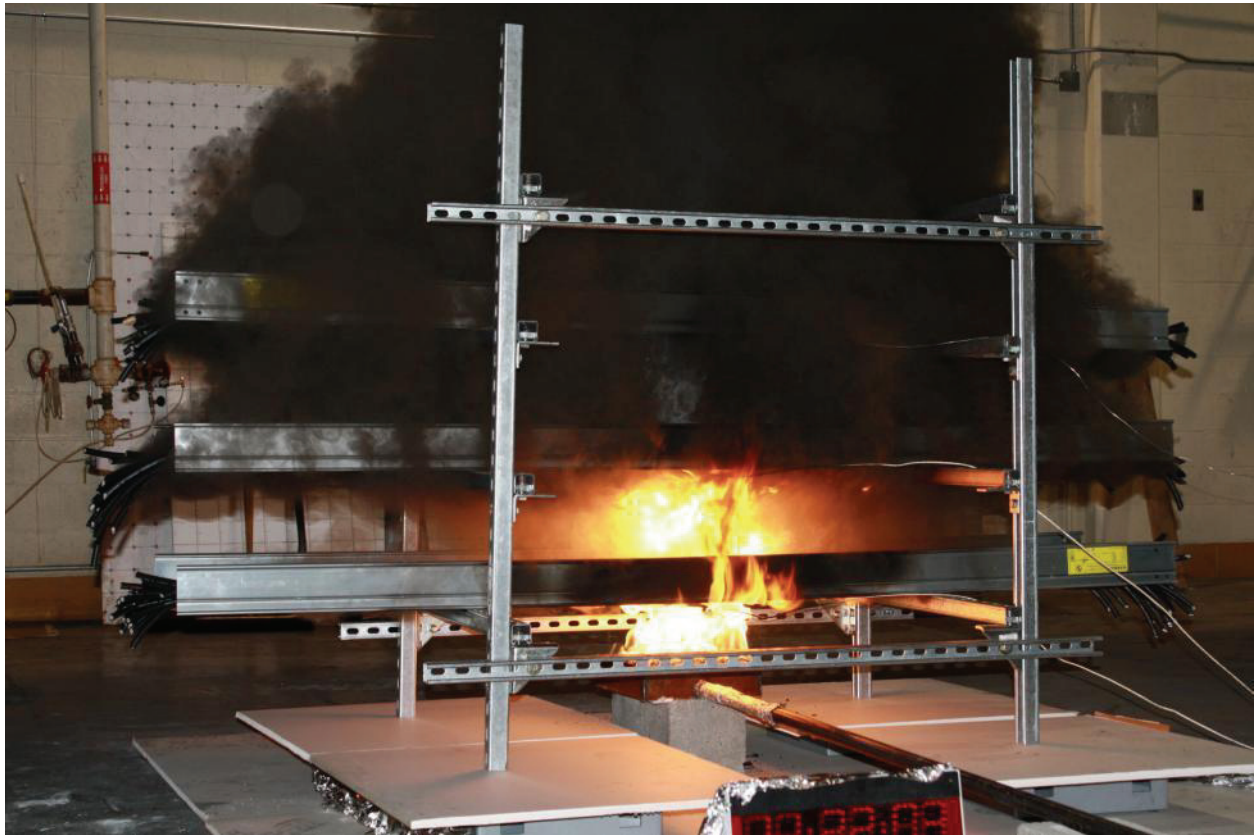
Figure 8-1. Multiple Tray (MT) cable test apparatus.
