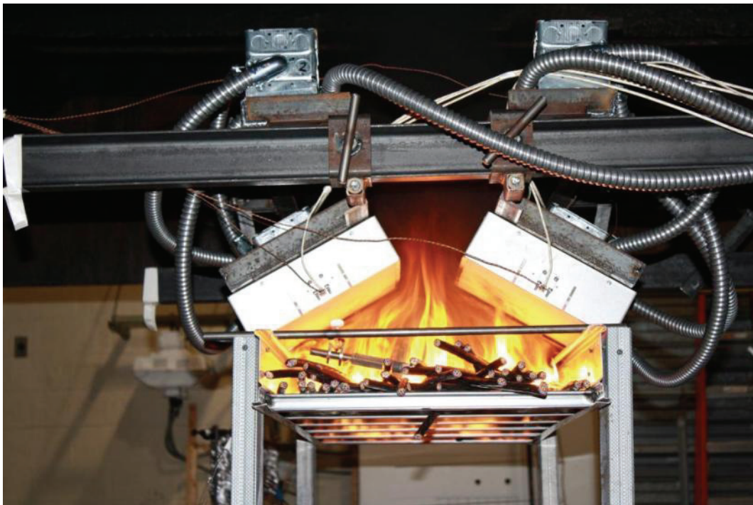
Figure 7-2. End view of Radiant Panel Apparatus.
