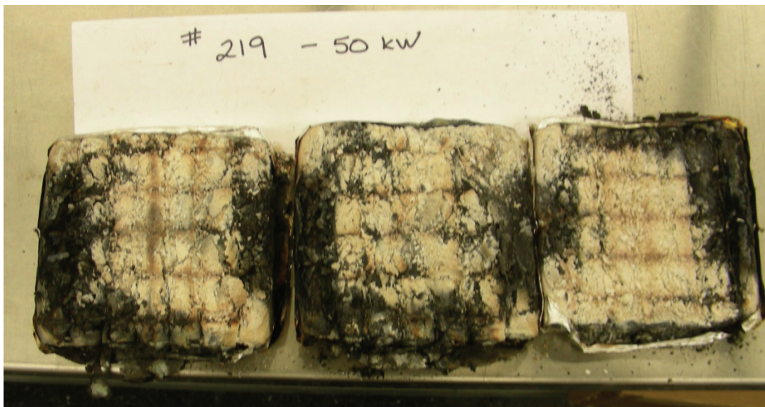
Figure 6-24. Photograph of Cable #219 after Cone Calorimeter test at 50 kW/m 2 .
