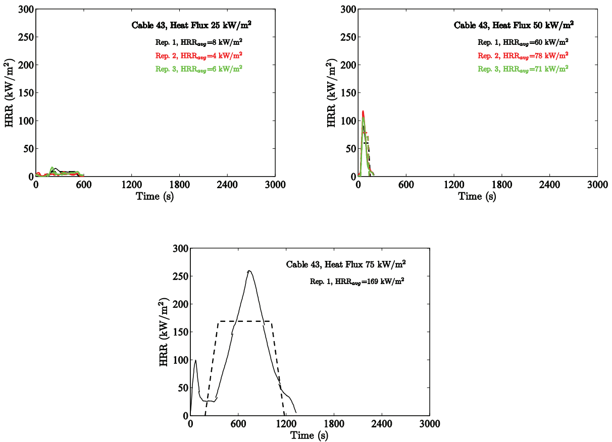
Figure 6-19. Heat Release Rates for Cable #43 in the Cone Calorimeter.
