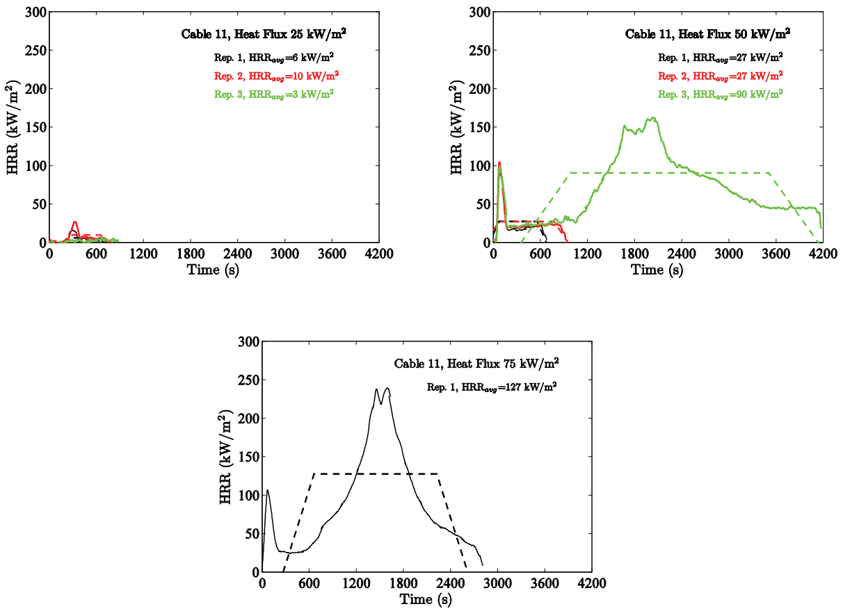
Figure 6-10. Heat Release Rates for Cable #11 in the Cone Calorimeter.
