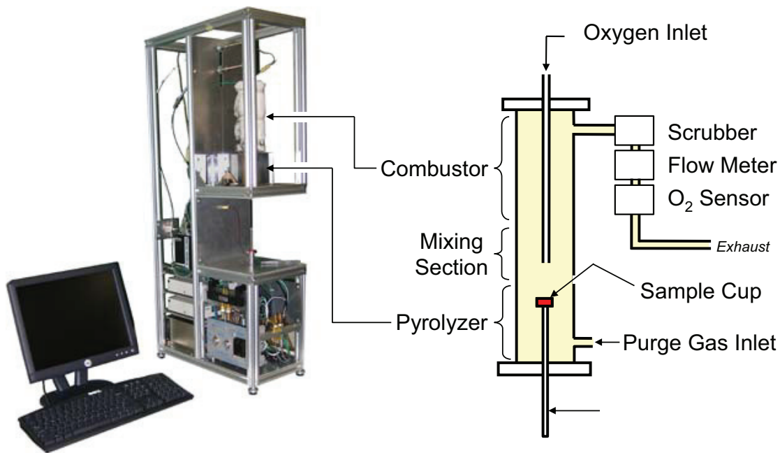
Figure 4-1. Pyrolysis Combustion Flow Calorimeter (PCFC).
