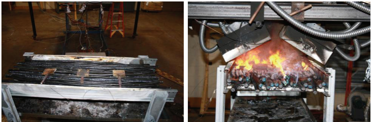
Figure 7-4. Photographs of RP Test 6.
