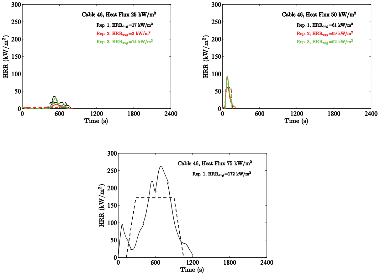
Figure 6-22. Heat Release Rates for Cable #46 in the Cone Calorimeter.
