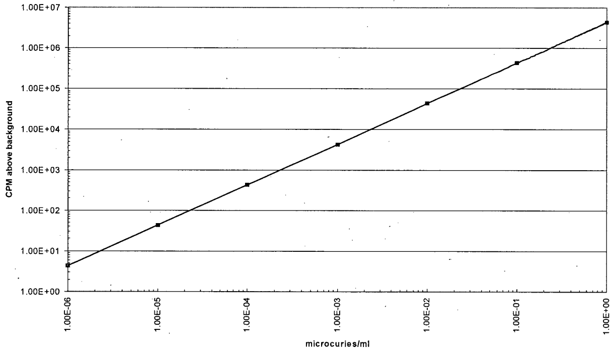
Counting Efficiency Curve for R-20 and R-28 Efficiency Factor = 4.3 E6 cpm/uCi/ml
