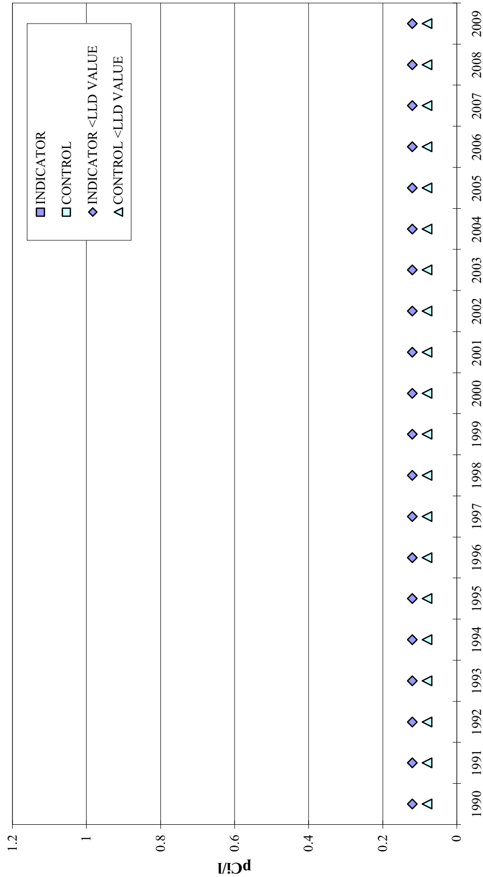
James A. FitzPatrick N.P.P. Milk Cs-137 Figure 9.9
