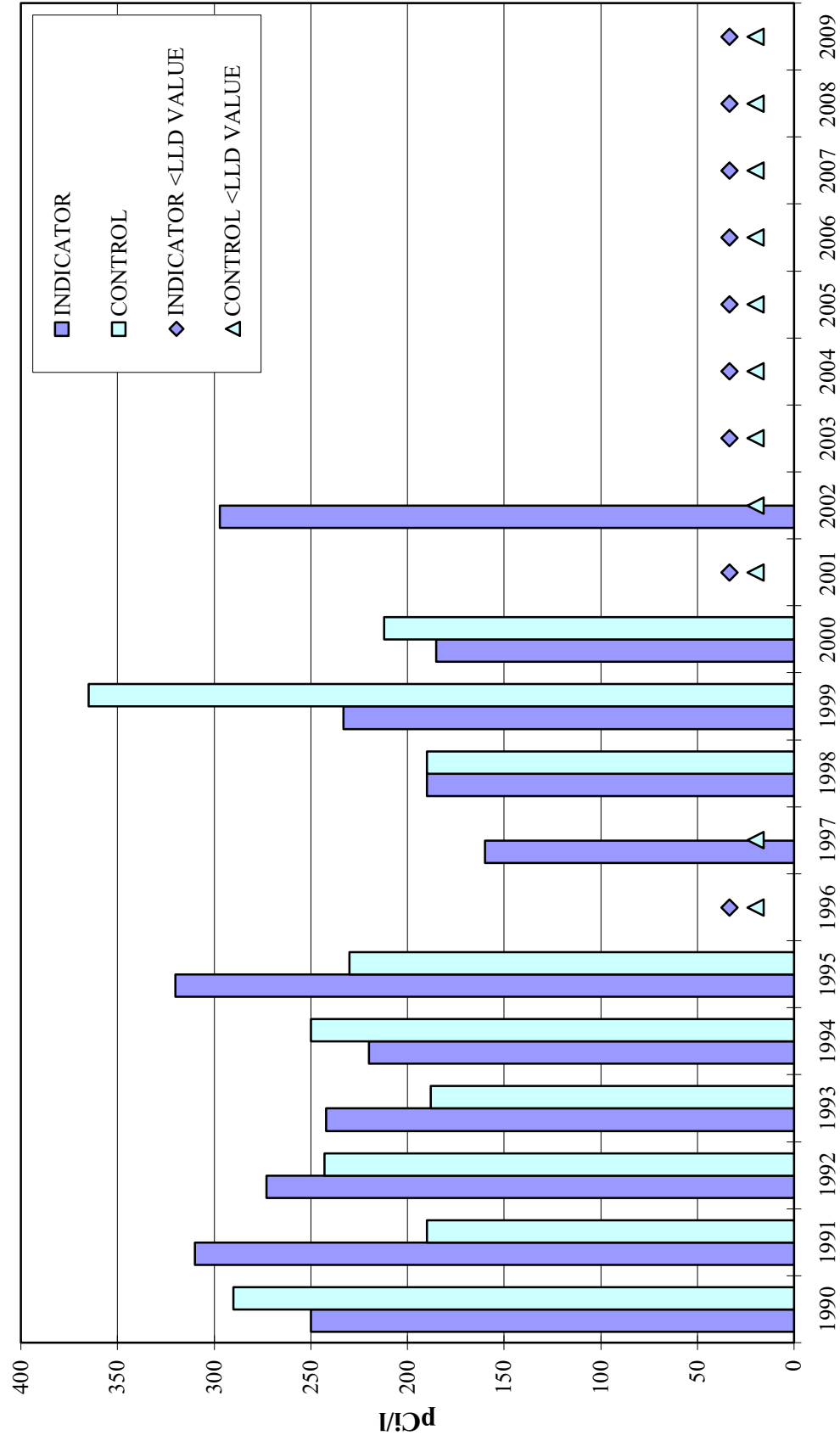
James A. FitzPatrick N.P.P. Surface Water - Tritium Figure 9.2
