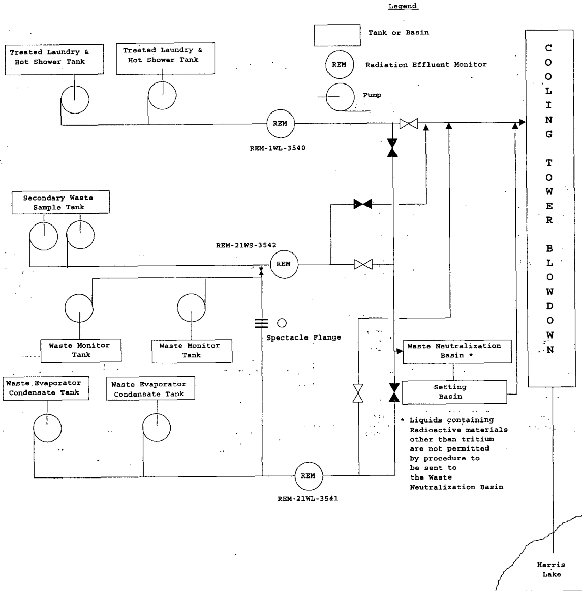
Figure 2.1-2 Liquid Effluent Flow Stream Diagram
