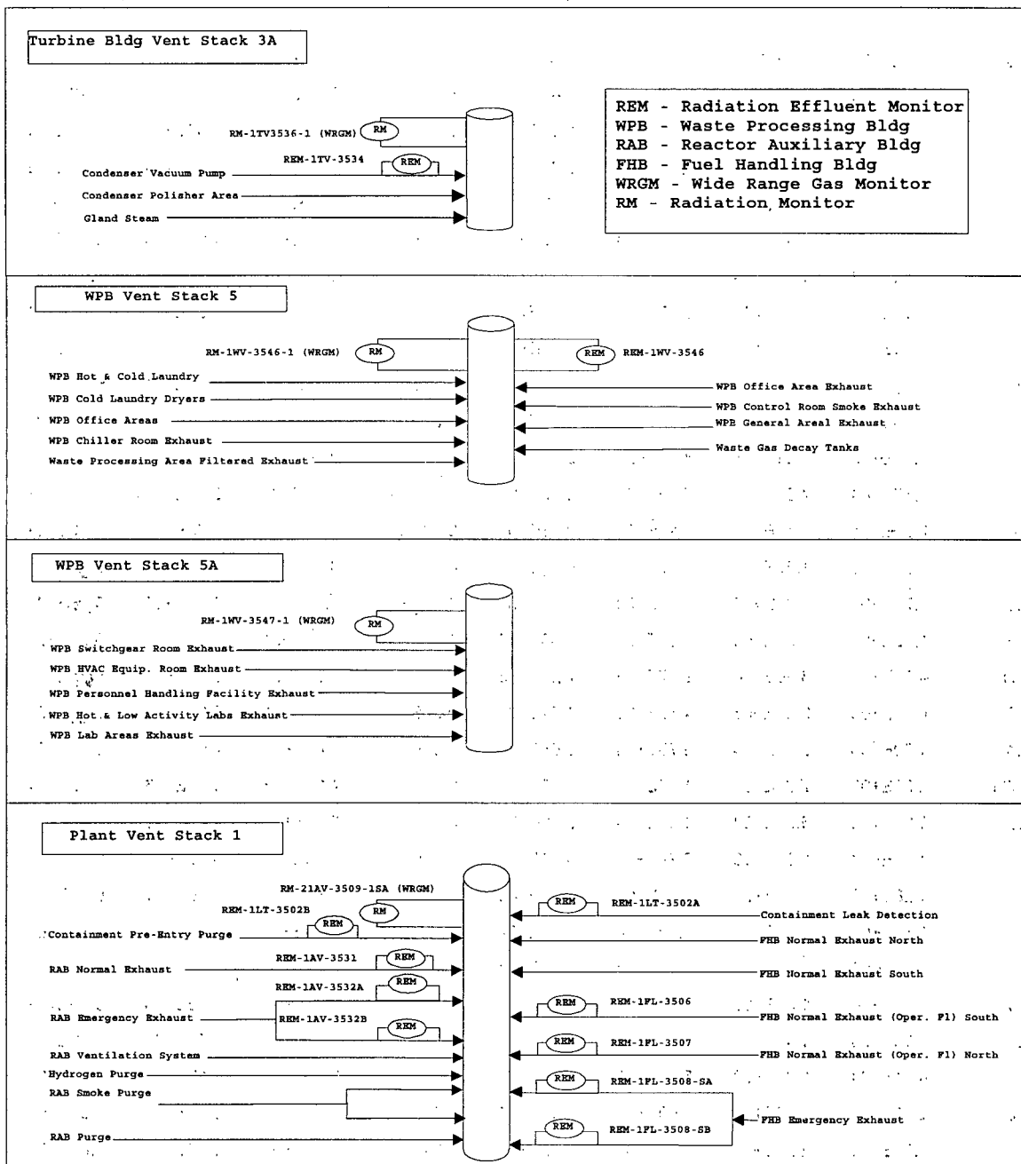
Figure 3.1 SHNPP Gaseous Waste Streams
