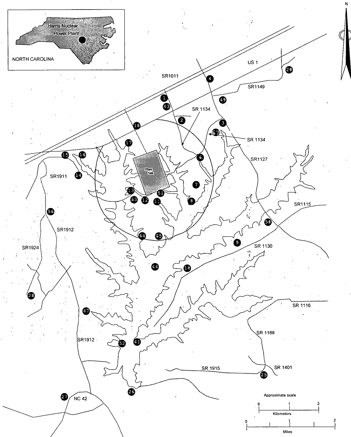
Figure 4.1-4 Environmental Radiological Sampling Points
