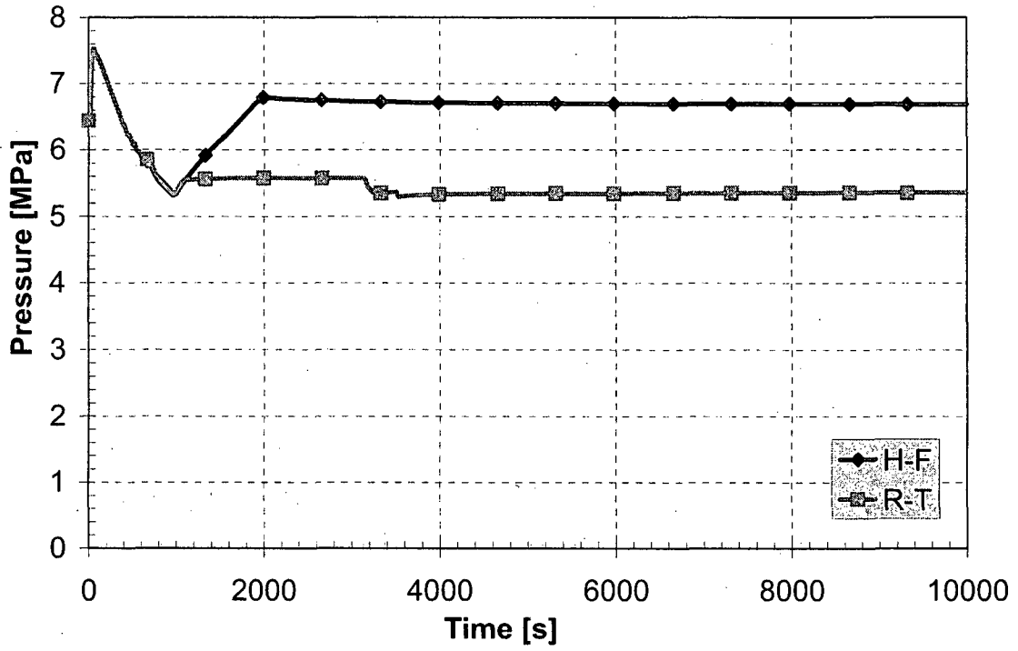
Figure 8 SG 1 pressure
