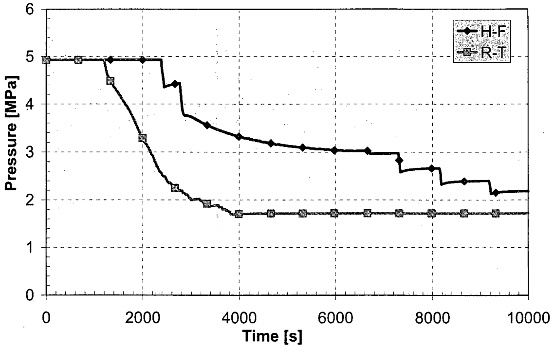
Figure 12 Accumulator No. 1 pressure
