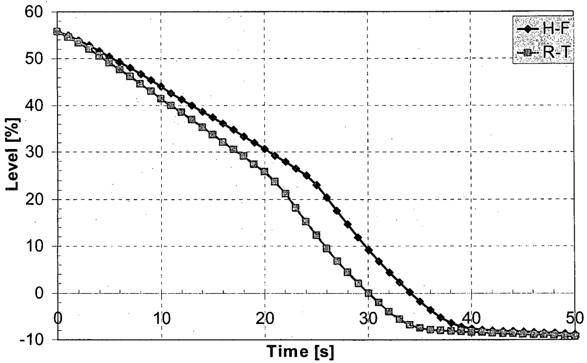
Figure 2 PRZ level
