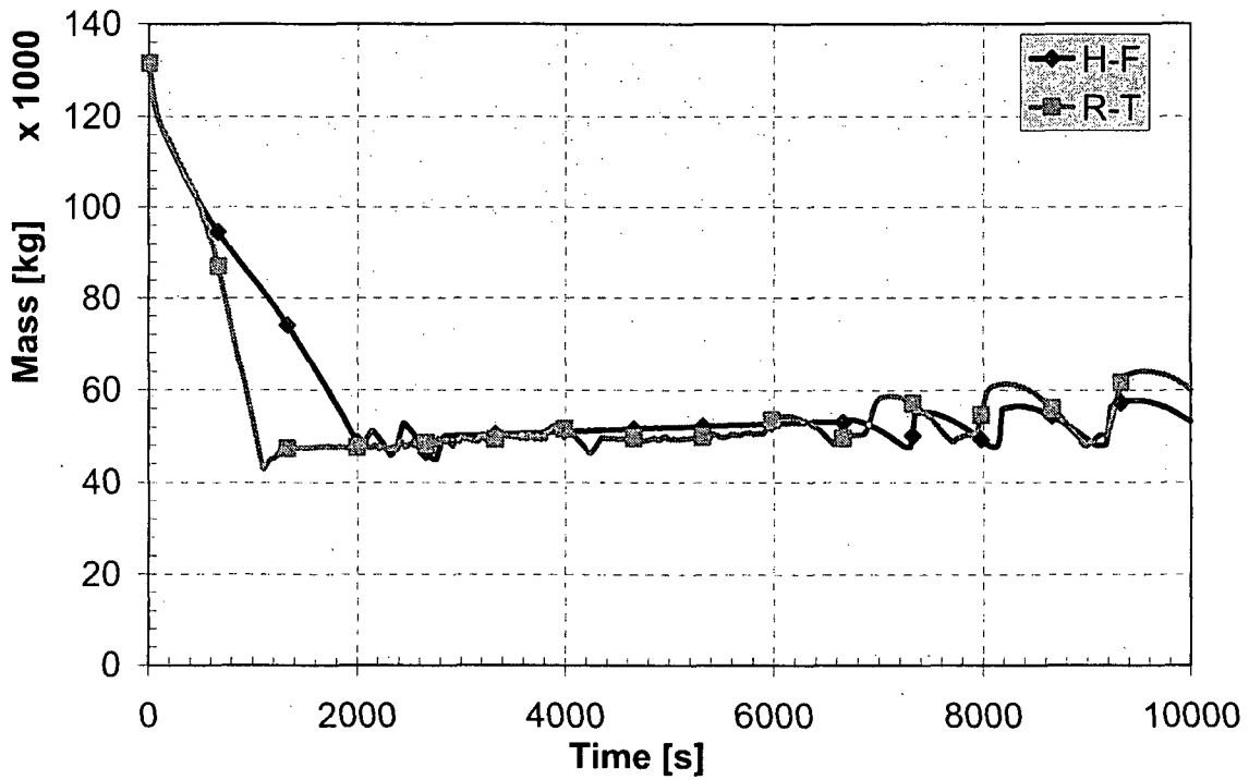
Figure 5 Primary mass
