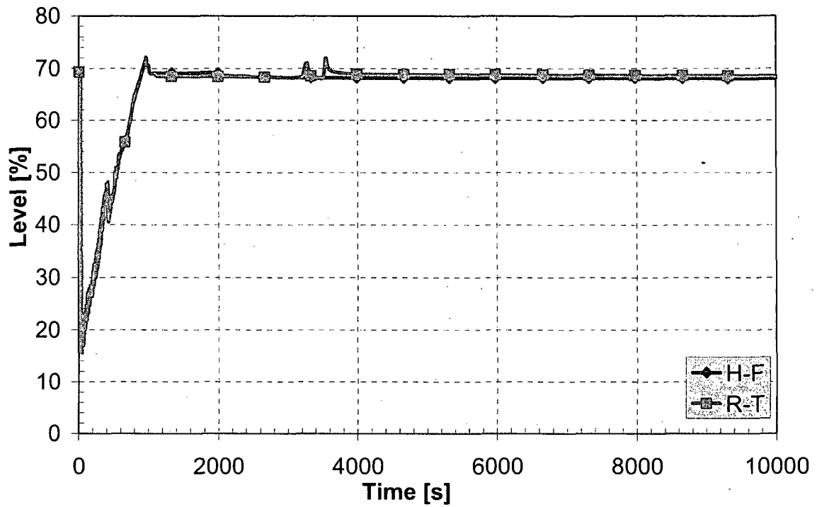
Figure 11 SG 2 level
