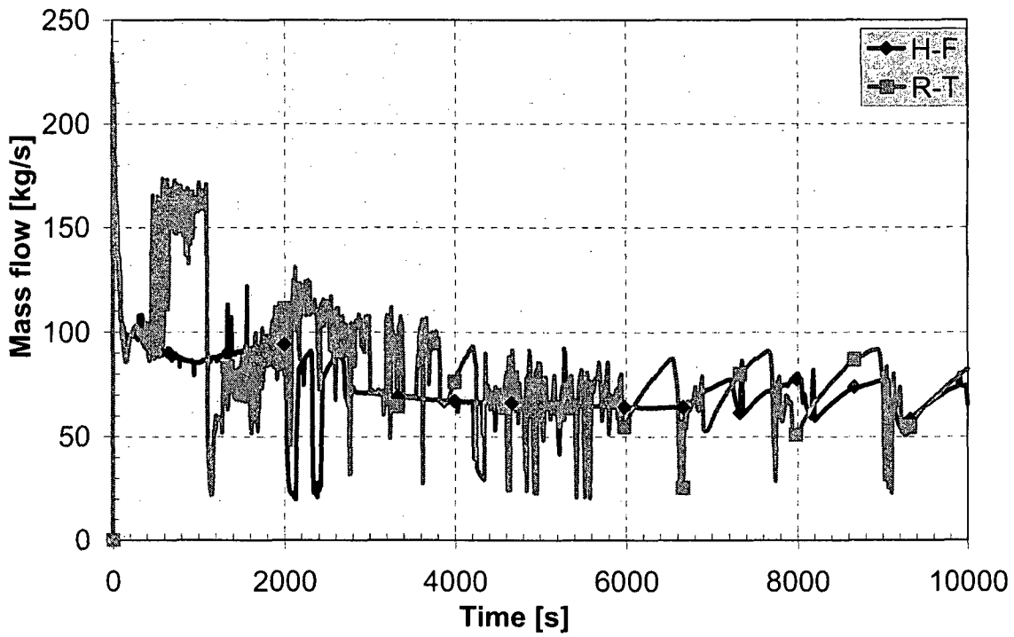
Figure 4 Break flow
