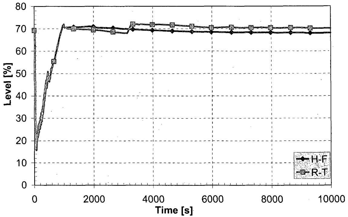
Figure 10 SG 1 level
