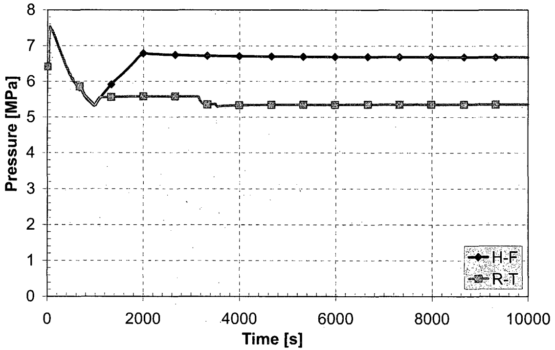
Figure 9 SG 2 pressure
