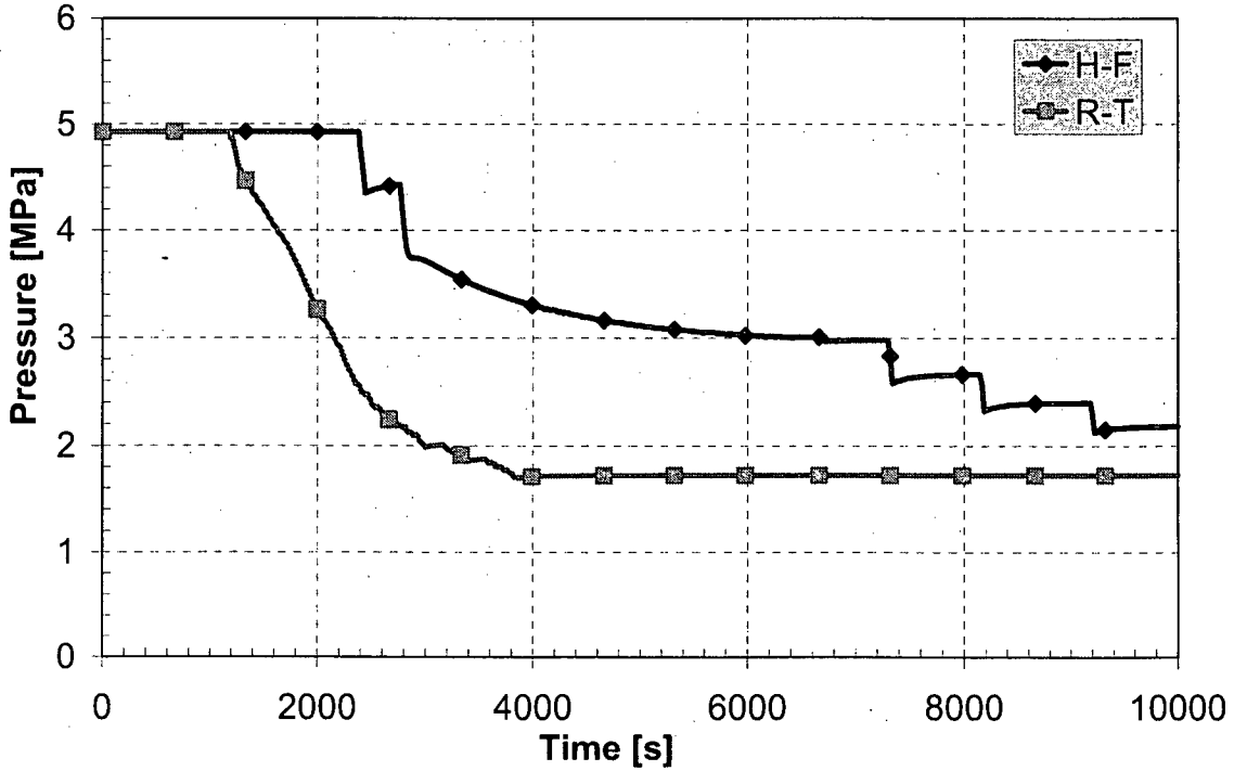
Figure 13 Accumulator No. 2 pressure
