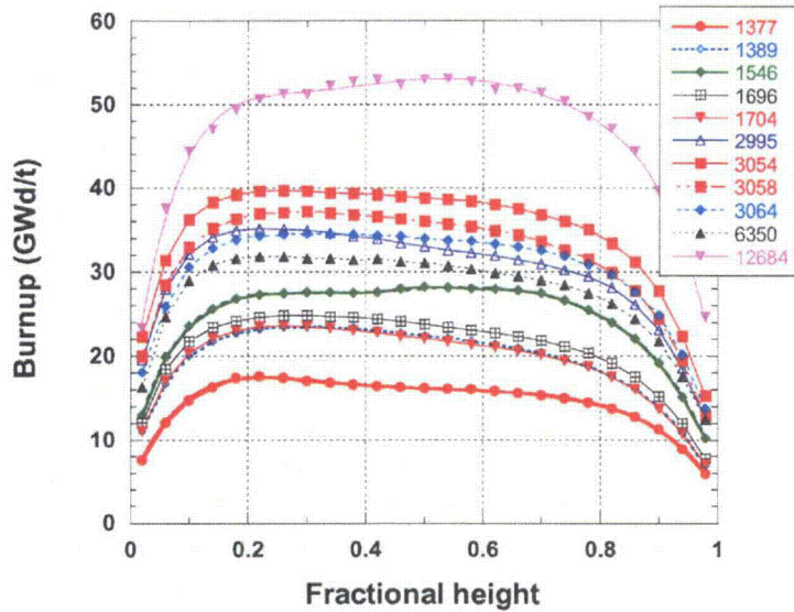
Figure 6 BWR burnup profiles for selected Oskarshamn 2 assemblies (Note: Several assemblies are shown that were not considered in this report.)
