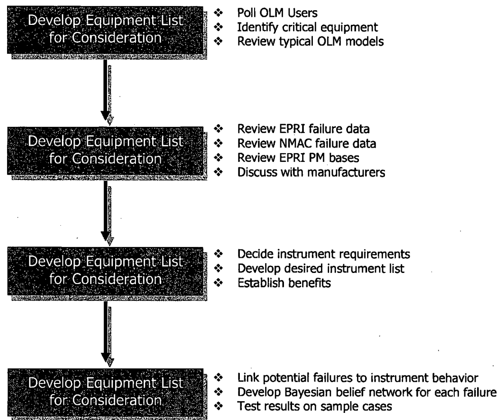
Figure 18. Equipment condition monitoring plan proposed by EPRI. 105
