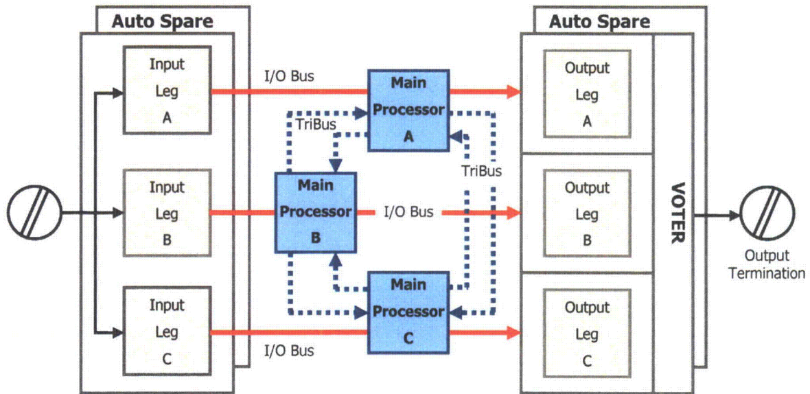
Figure 35. Triple modular redundant architecture of the Tricon PLC system.
