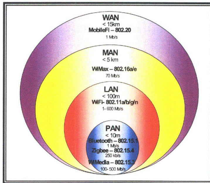
Figure 9. Wireless protocol coverage.
