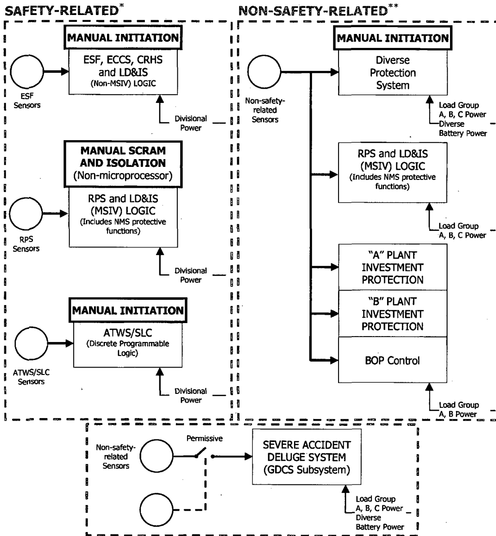
Figure 34. Economic Simplified Boiling Water Reactor sensors and power diversity (Ref. 150).
