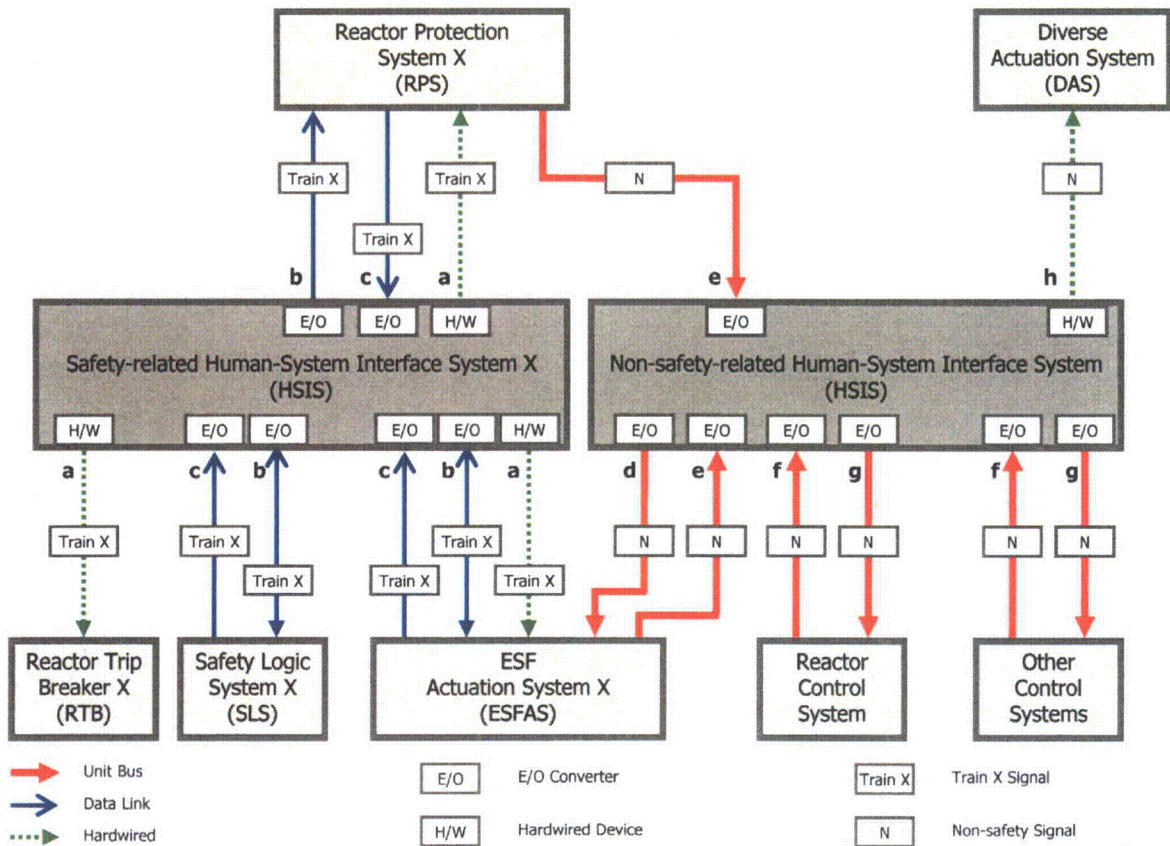
Figure 31. Communication network between the human-system interface system and other systems.
