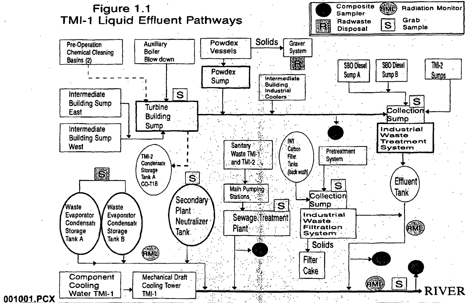
FIGURE 1.1 - TMI-1 Liquid Effluent Pathways -
