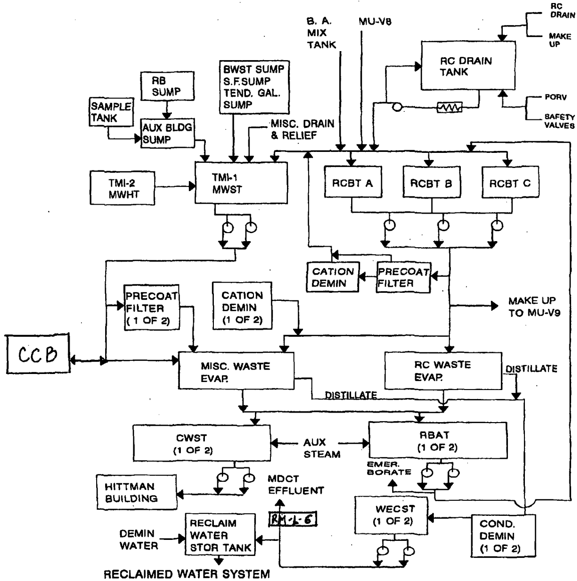
FIGURE 3.1 TMI-1 Liquid Radwaste
