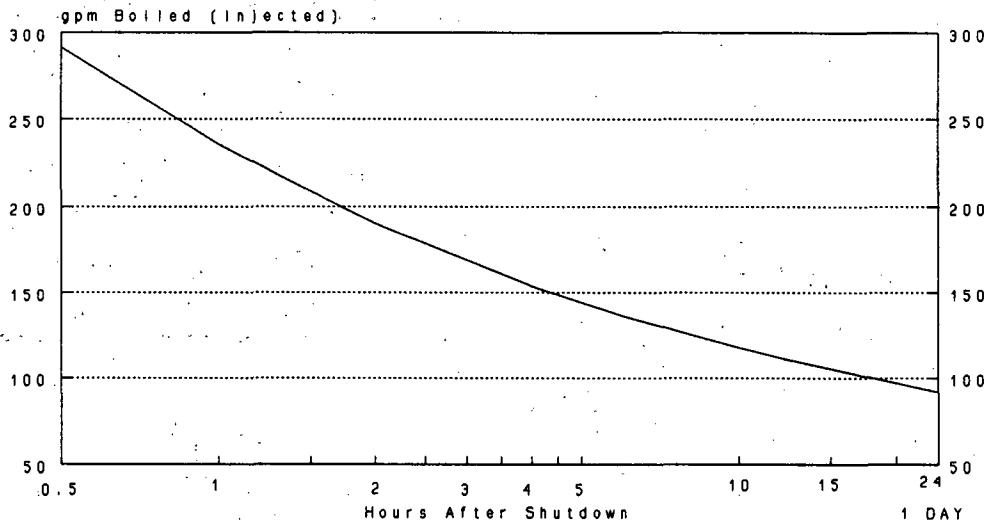
Fig. A-1 Injection required to replace water lost by boiling resulting from decay heat for a 3000 MW(t) plant (0.5–24 h after shutdown).
