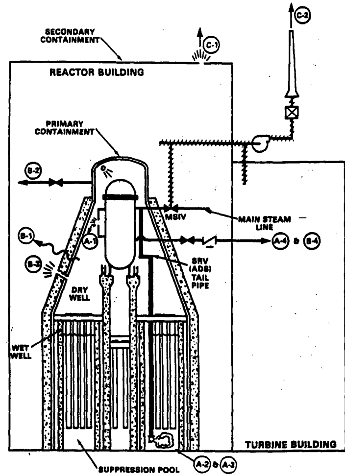
Fig. C-4 BWR Mark II simplified release pathways.
