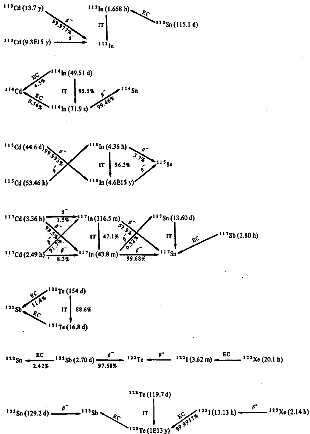
Fig. M-1 Decay diagrams for selected radioisotopes (continued).
