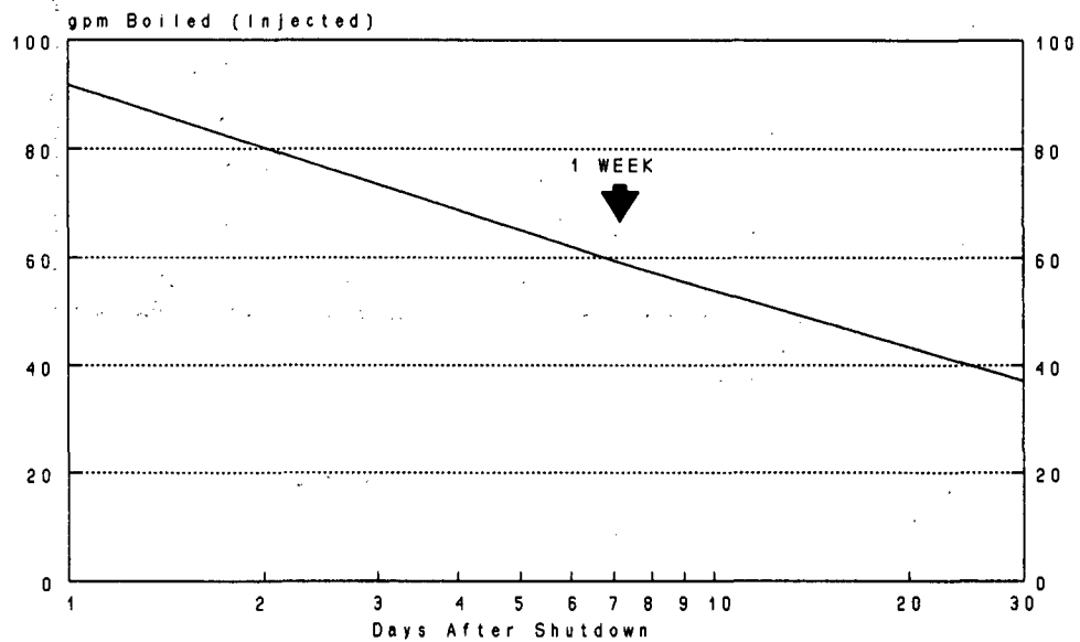
Fig. A-2 Injection required to replace water lost by boiling resulting from decay heat for a 3000 MW(t) plant (1–30 days after shutdown).
