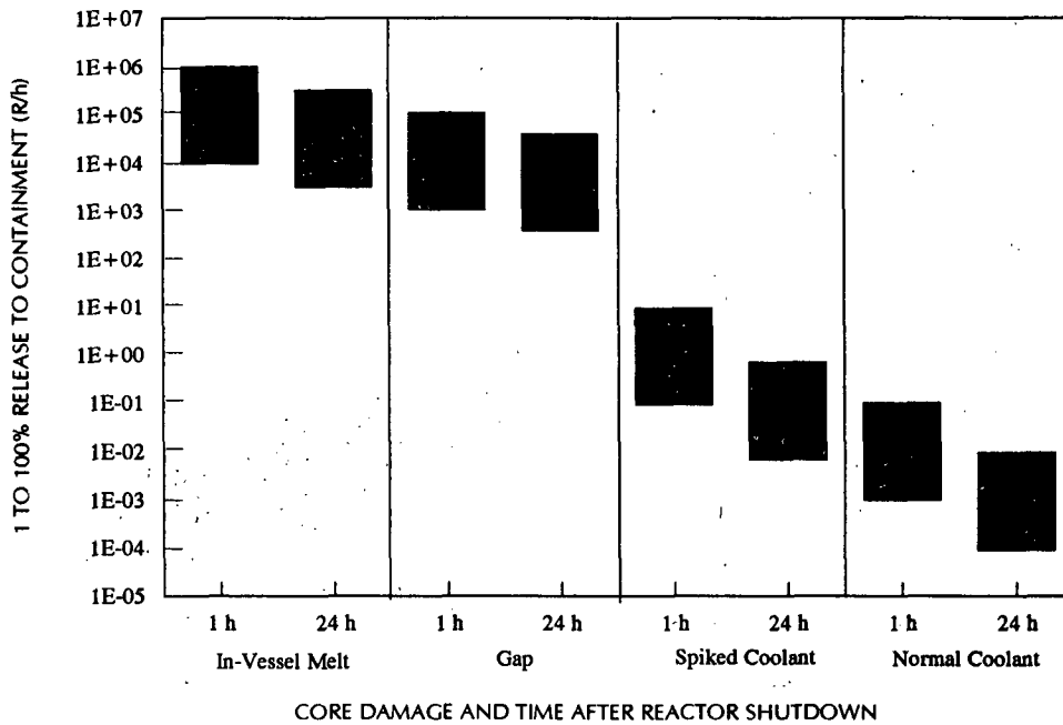
Fig. A-8 BWR Mark I & II drywell containment monitor response (sprays off).
