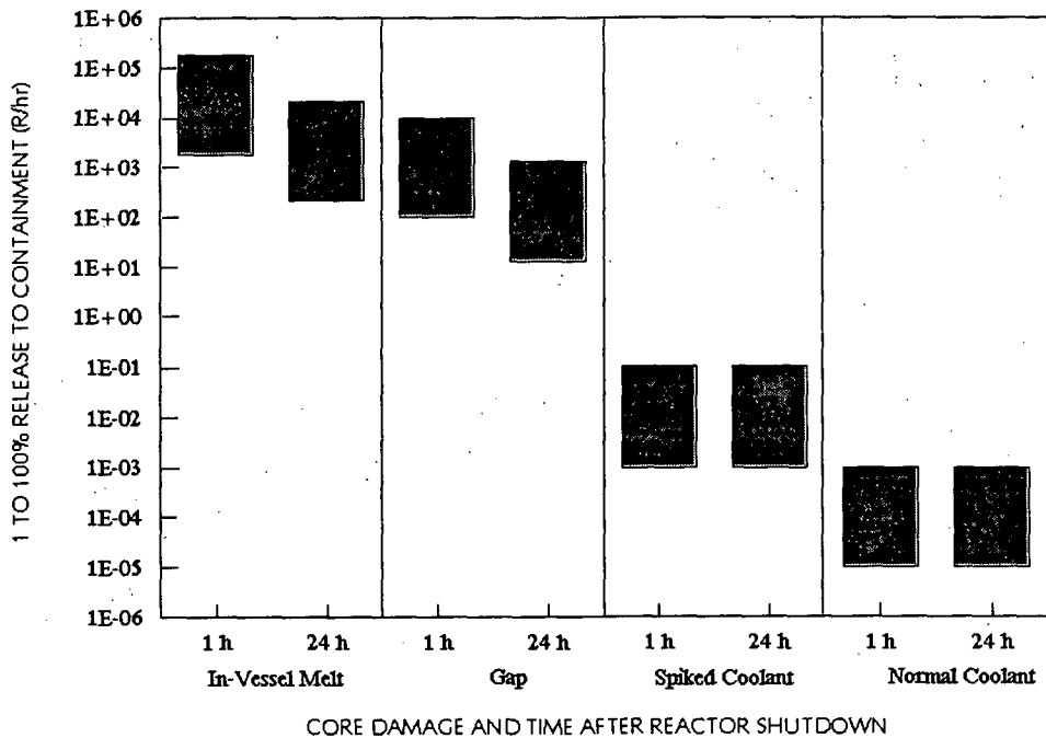
Fig. A-10 BWR Mark III drywell containment monitor response (sprays on).
