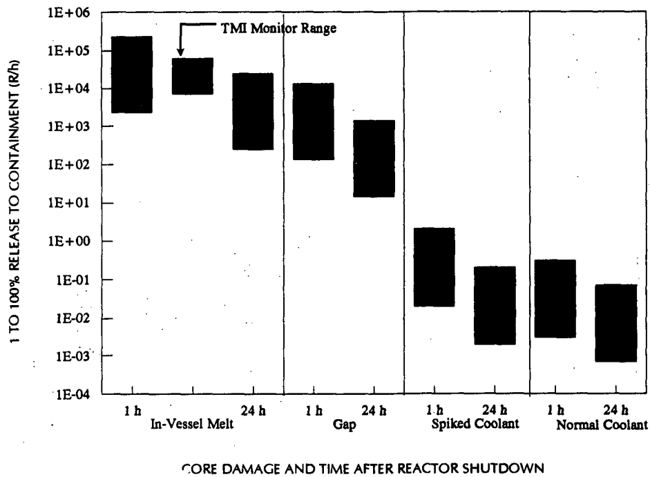
Fig. A-6 PWR containment monitor response (sprays off).
