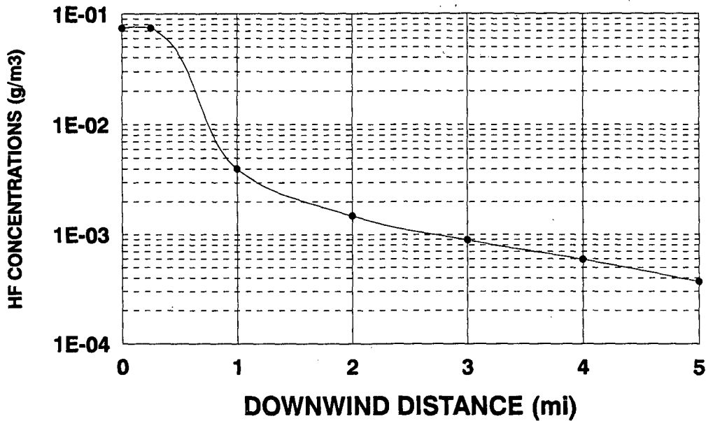
Fig. E-3 Air concentrations of hydrogen fluoride from release of 1 metric ton of liquid UF 6 . a
