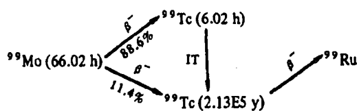
Fig. M-1 Decay diagrams for selected radioisotopes (continued).
