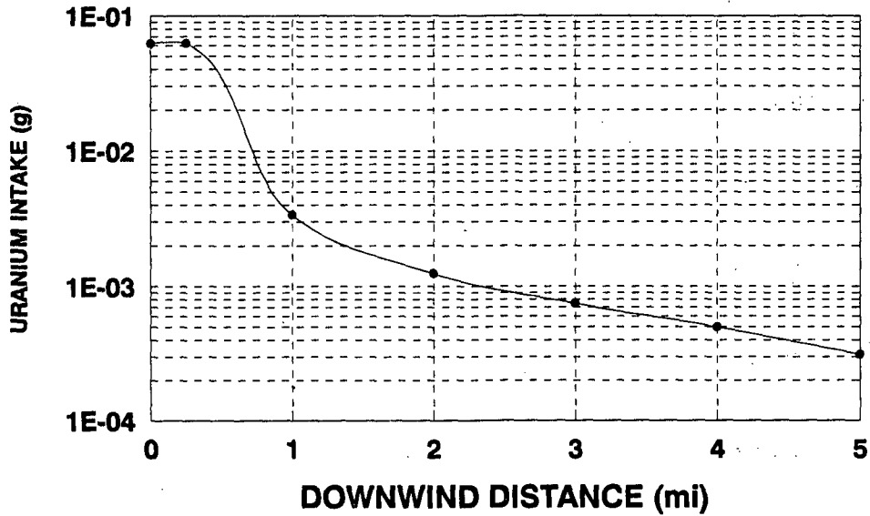
Fig. E-2 Adult uranium intake resulting from release of 1 metric ton of liquid UF 6 . a
