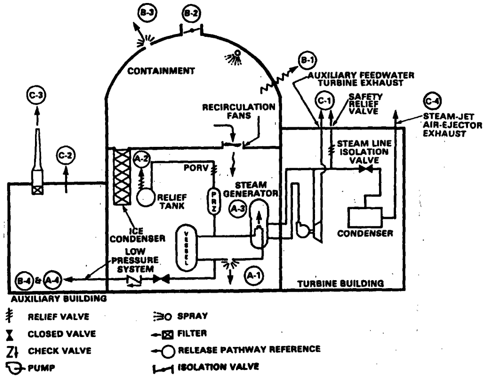
Fig. C-2 PWR ice condenser containment simplified release pathways.
