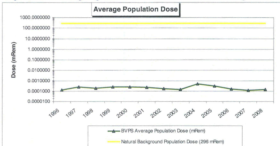
Graph of Annual Average Population Dose: BVPS Dose and Natural Background Dose
