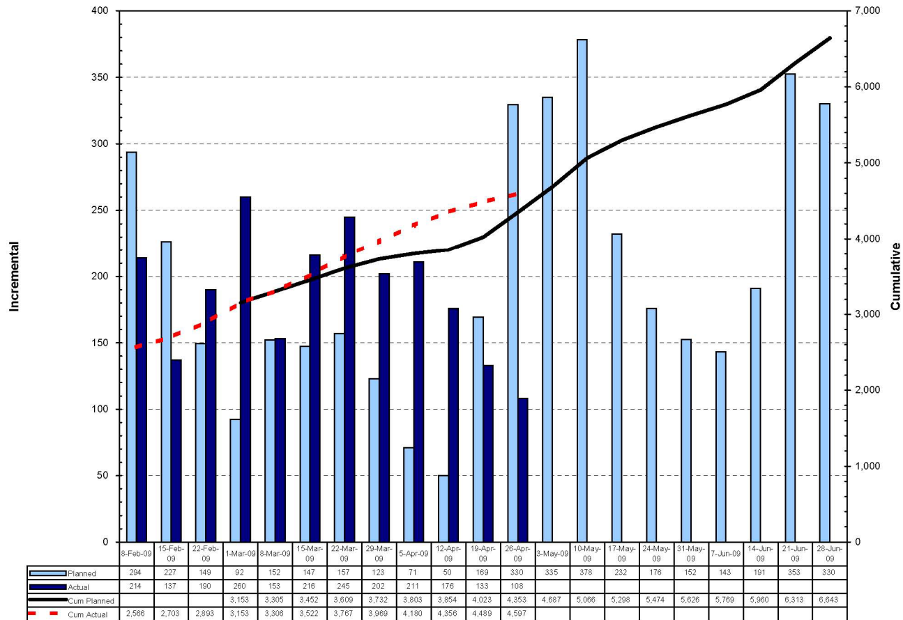
BAKER CONCRETE CONSTRUCTION, INC. Total Release 2 Quantity (ea) of Embedded Plates (Planned Values Reflect Current Approved Schedule of Feb 26, 2009)
