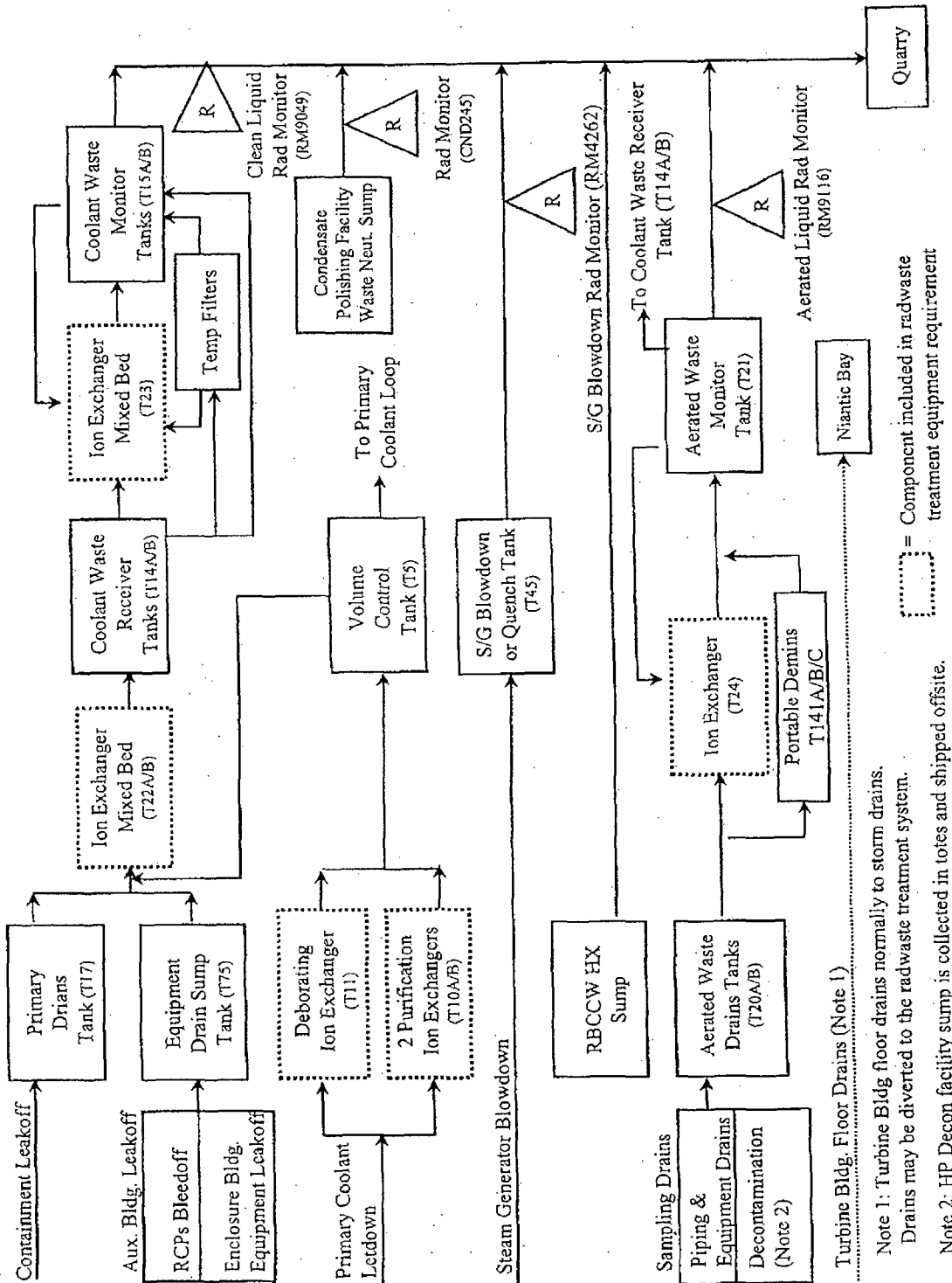
Figure I.C.-2, "Simplified Liquid Effluent Flow Diagram Millstone Unit 2"
