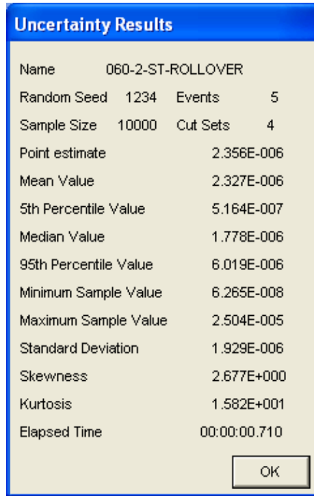
Figure B6.4-20. Uncertainty Results for the Site Transporter Rollover (Tipover) Fault Tree
