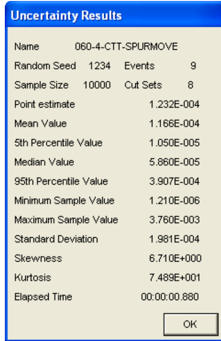
Figure B2.4-5. Uncertainty Results for the “Spurious Movement of the CTT in the Cask Preparation Area During Cask Preparation” Fault Tree
