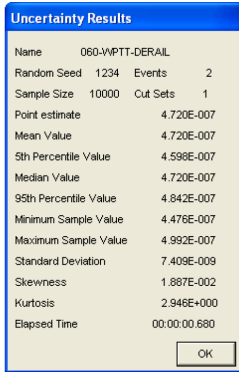
Figure B5.4-11. Uncertainty Results for the Derailment of the WPTT Fault Tree
