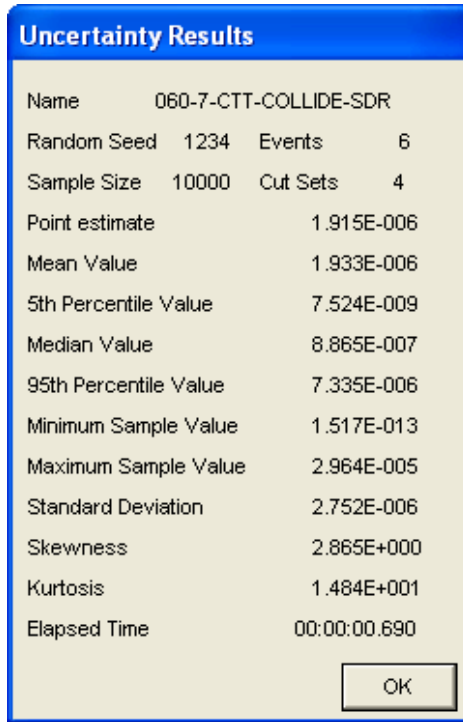
Figure B3.4-7. Uncertainty Results for the Shield Door Closes on Conveyance Fault Tree
