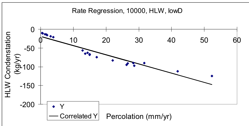
Figure I.2-7. HLW Rate Regression, Low D, 10,000 Years, Unmixed High Invert Transport
