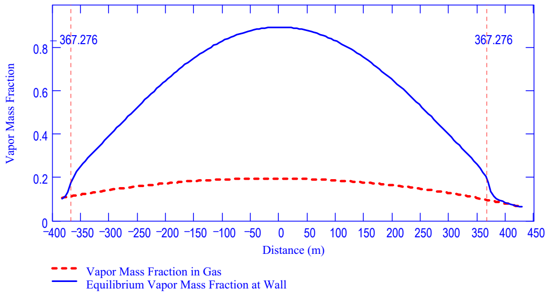
Figure 6.3.7-4. Vapor Mass Fraction in Gas: Choice #7, 1,000 Years, Mean Percolation Rate, Well-Ventilated Drip Shield, Low Invert Transport, High Dispersion Coefficient
