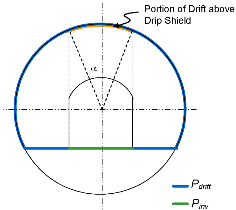
Figure 6-5[a]. Schematic for the Drift Form Factor, f_{drift}
