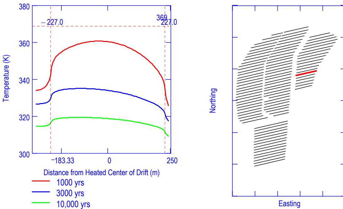
Figure 6.3.5-11. Drift Wall Temperatures for Chosen Drift #5
