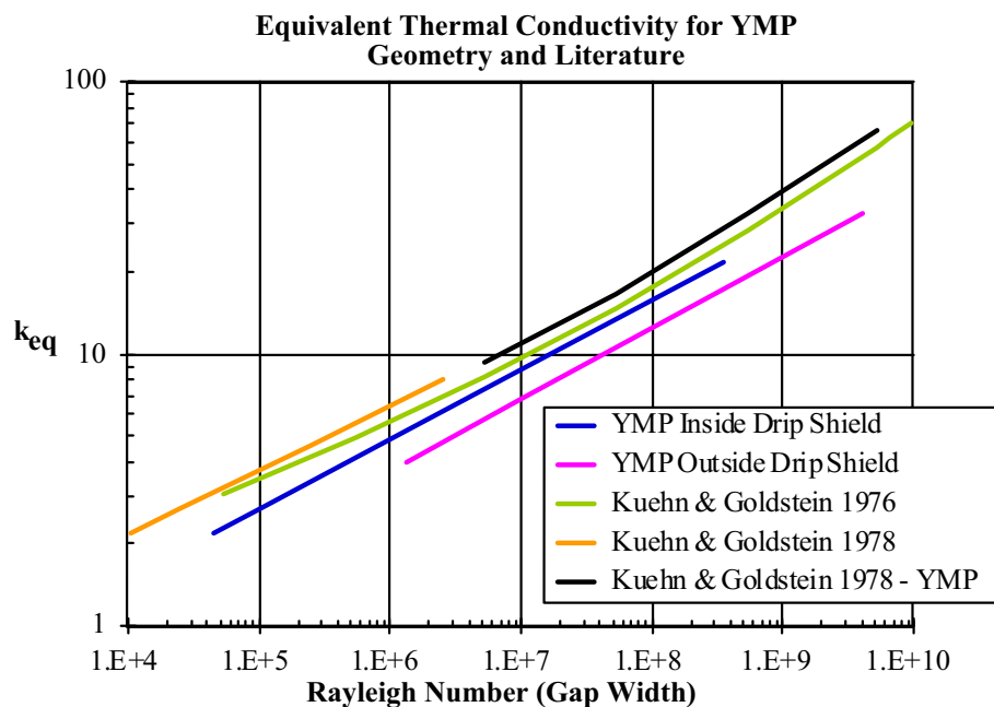
Figure 6.4.7-3. Comparison of Natural Convection Correlation Equations
