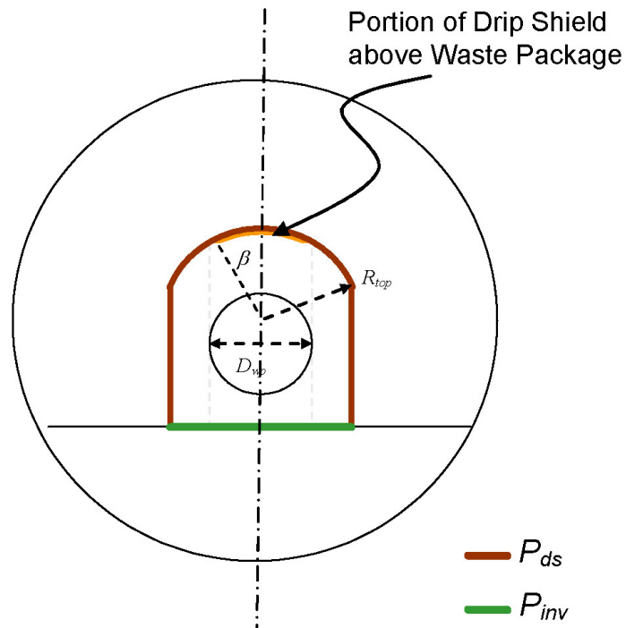
Figure 6-6[a]. Schematic for the Drip Shield to Waste Package Form Factor, f_{wp}
