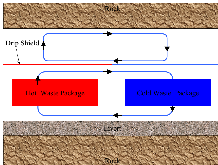
Figure 6.3.3-7. Convective Cells Connecting Hotter and Colder Waste Packages
