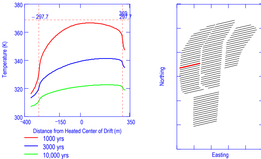
Figure 6.3.5-9. Drift Wall Temperatures for Chosen Drift #3
