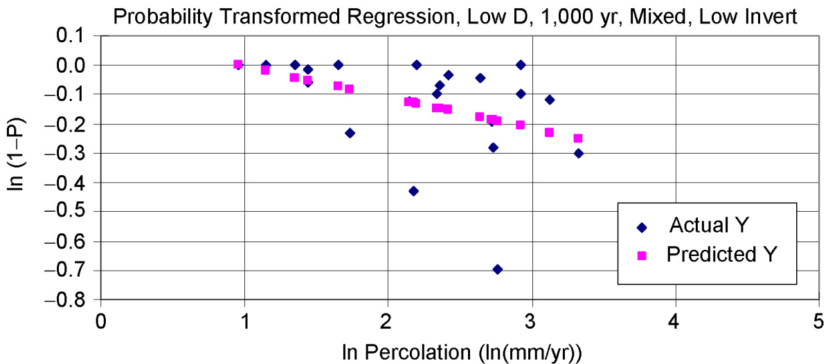
Figure 6-11[a]. Current Probability Regression Analysis (ventilated drip shield (mixed), low invert transport, low dispersivity, 1,000 years)
