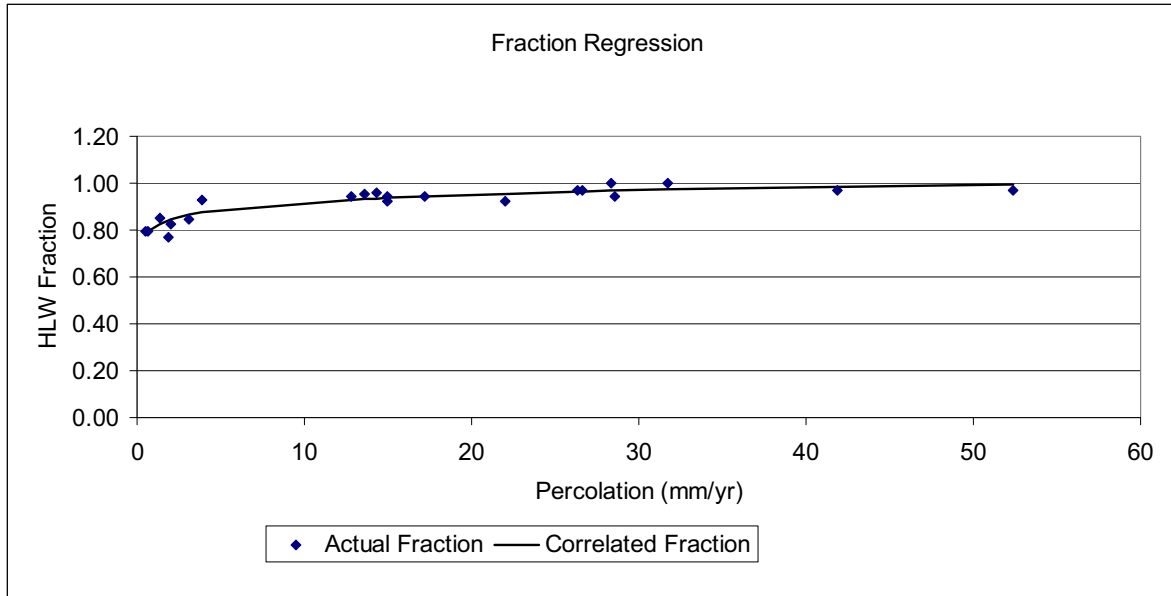
Figure I.2-8. HLW Fraction Regression, Low D, 10,000 Years, Unmixed High Invert Transport
