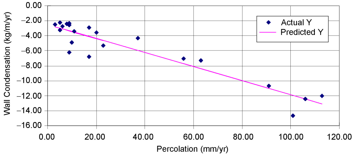
Figure 6-13[a]. Current Regression Analysis with Maximum Percolation ~113 mm/yr (ventilated drip shield (mixed), high invert transport, low dispersivity, 1,000 years)
