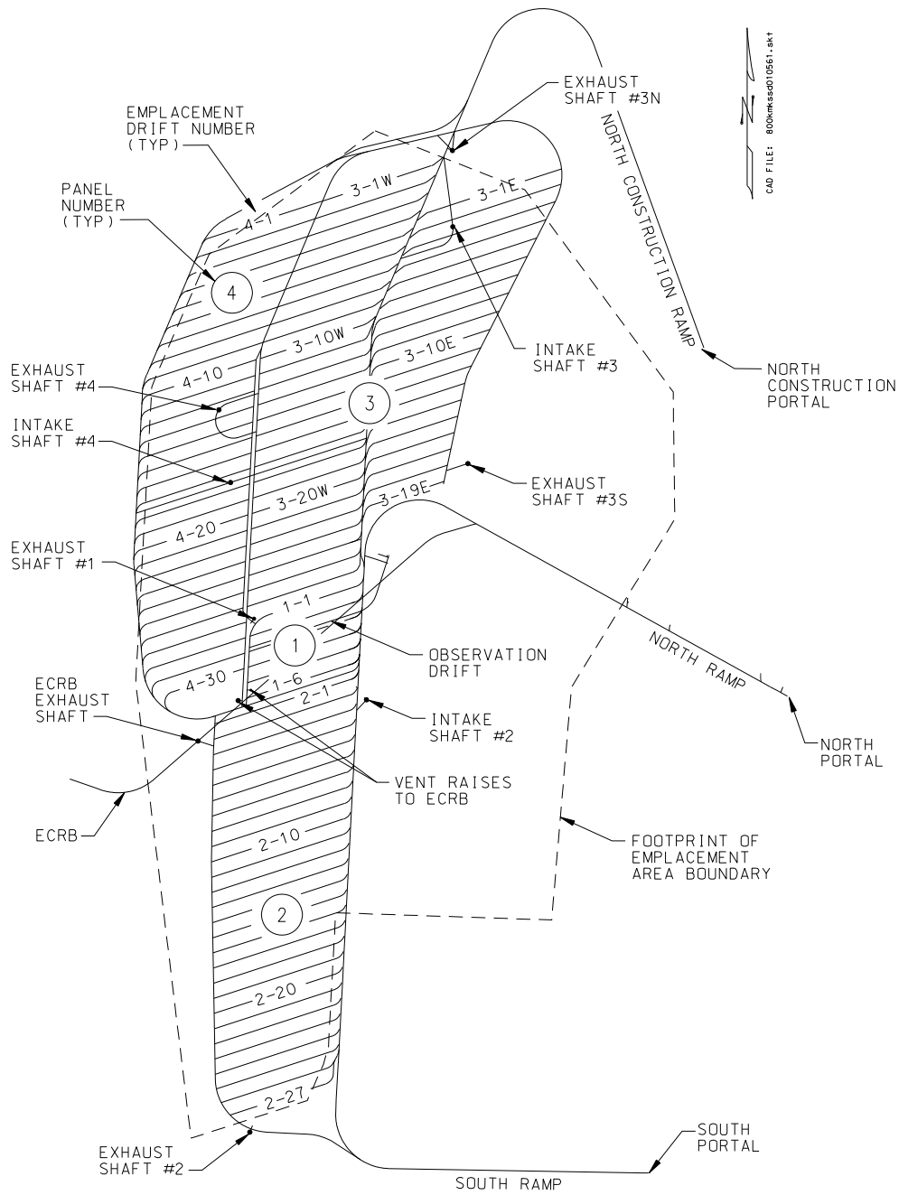
Figure 6-1[a]. Repository Layout
