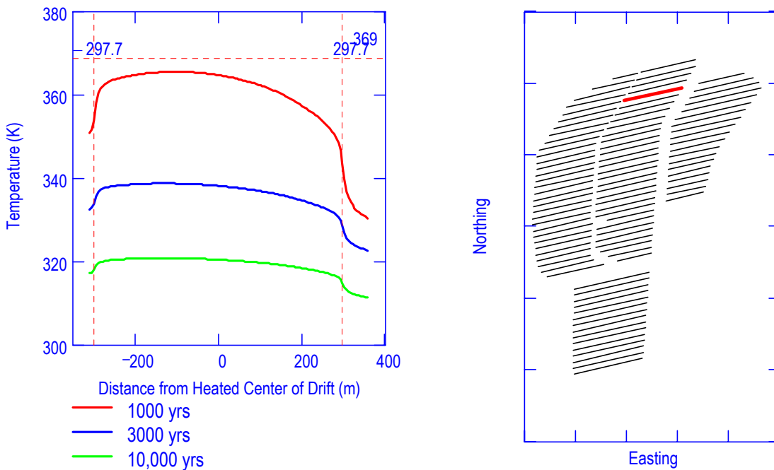
Figure 6.3.5-7. Drift Wall Temperatures for Chosen Drift #1
