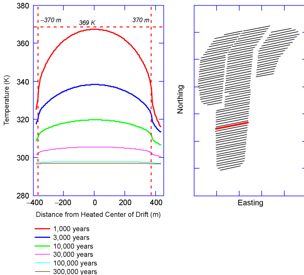
Figure 6-4[a]. Drift Wall Temperatures (Chosen Drift #7)
