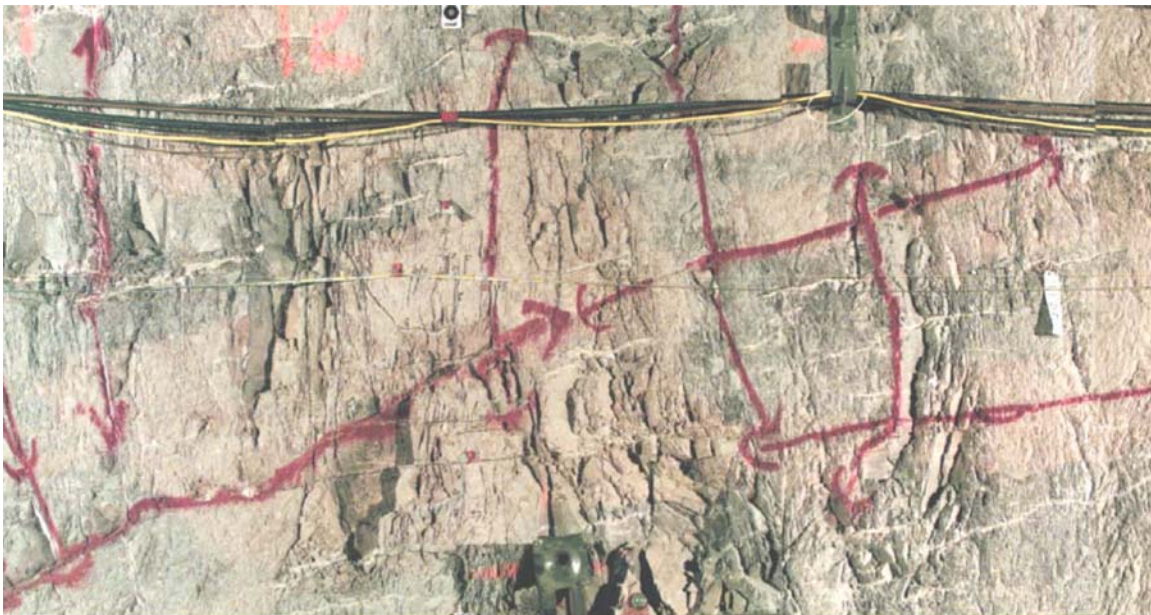
Figure H-2. Fracture Frequency and Lithophysal Abundance Measured in the ECRB Cross-Drift from Stations 0+00 to 27+00
