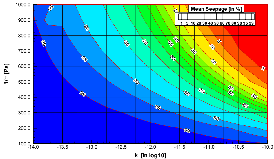
Figure 6.4-10. Mean Seepage Percentage for the Collapsed Drift Scenario as a Function of Capillary-Strength Parameter and Mean Permeability for a Percolation Flux of 200 mm/year
