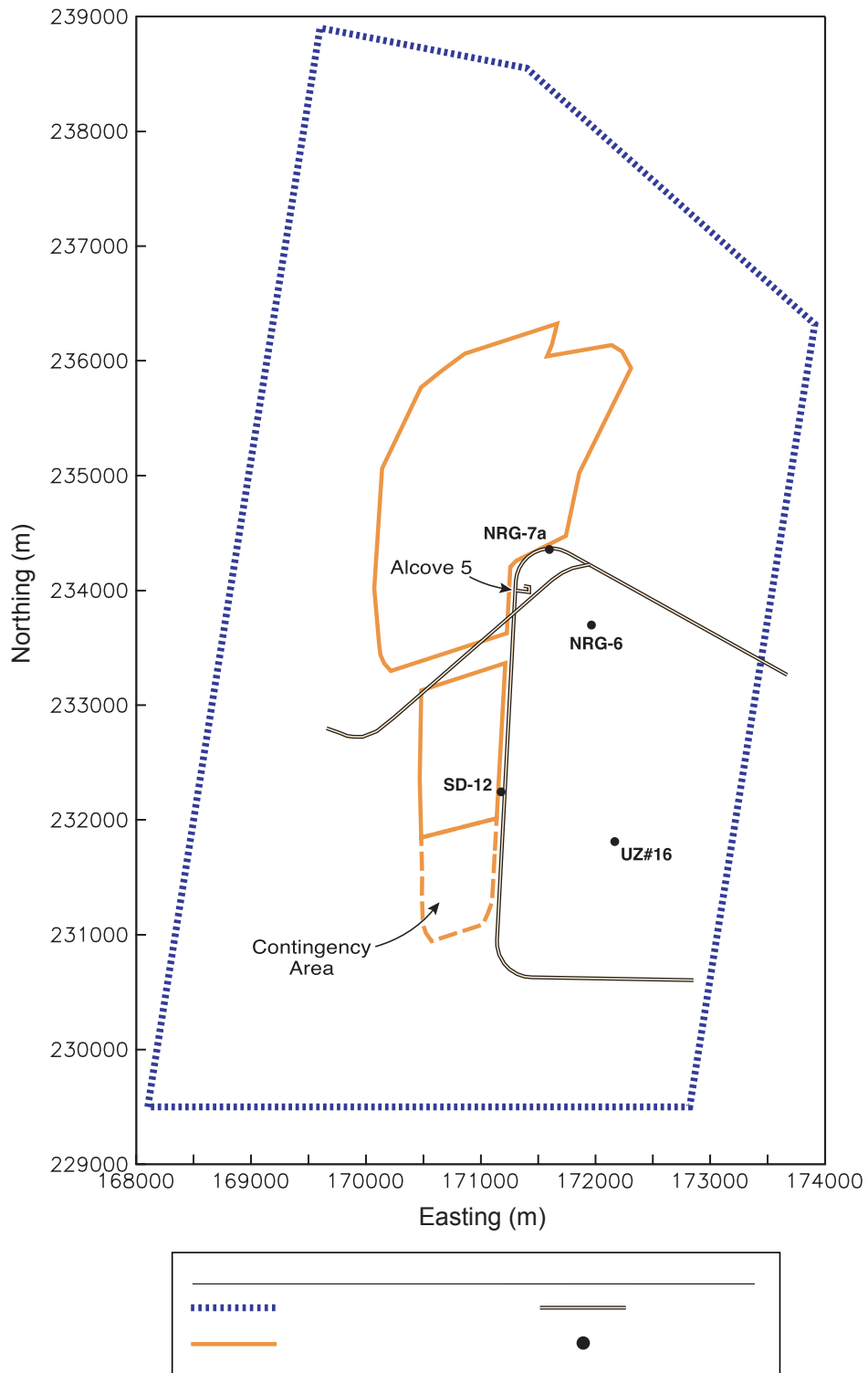
Figure 6.6-5. Map Showing Approximate Location of Surface-B used Boreholes NRG-7a, NRG-6, SD-12, and UZ#16 and SHT/DST Heater Test Area (Alcove 5), together with the 2002 Repository Layout
