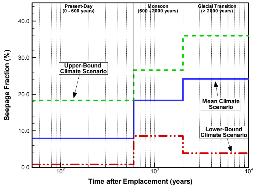
Figure 6.8-4. Mean Seepage Percentage as a F unction of Time after Emplacement for TptII Unit and Different Infiltration Scenarios
