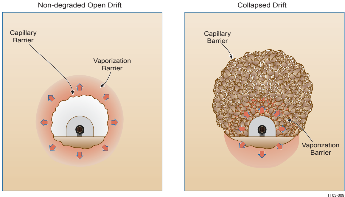
Figure 6.4-16. Schematic of TH Differences between an Open Nondegraded Drift and a Rubble-filled Collapsed Drift
