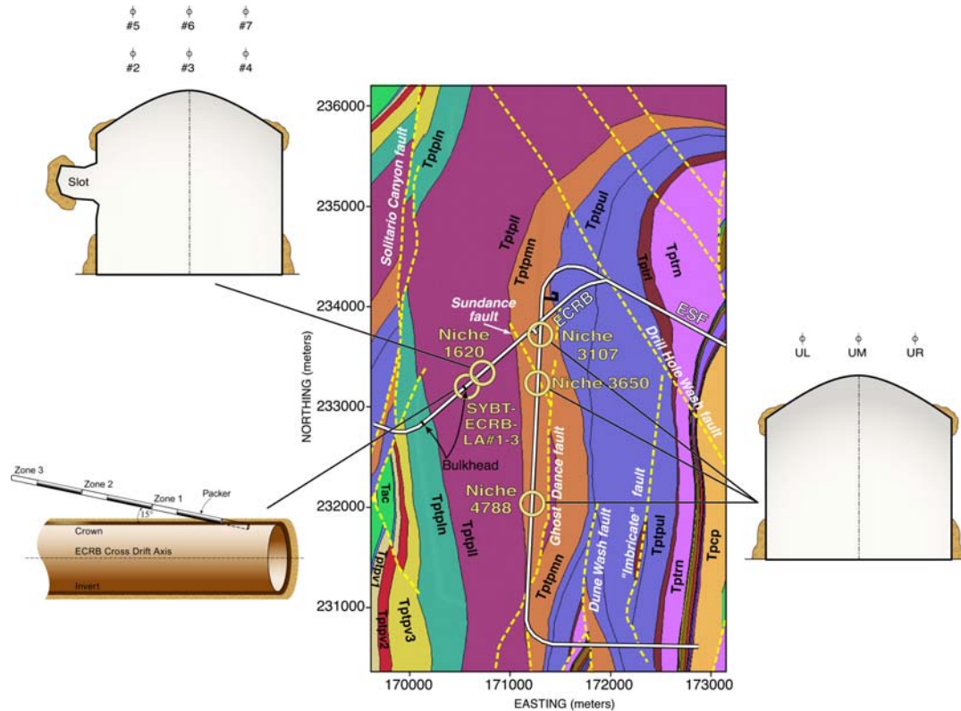
Figure 6.6-1. Schematic Geological Map Showing Approximate Location and Schematic Setup of Niches and Systematic Testing Boreholes SYBT-ECRB-LA#1-3 (Formations Depicted at the Elevation of the ESF)
