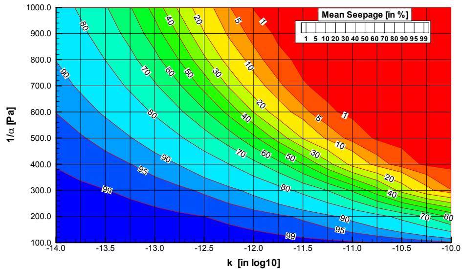
Figure 6.4-8. Mean Seepage Percentage for the Collapsed Drift Scenario as a Function of Capillary-Strength Parameter and Mean Permeability for a Percolation Flux of 5 mm/year
