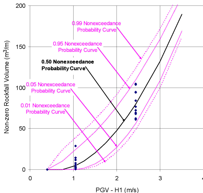
Figure 6-6[a]. Comparison of Percentiles on the Gamma Distributions for Conditional Lithophysal Rock Volumes as a Function of PGV
