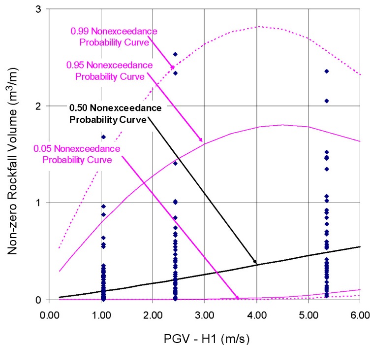
Figure 6-9[a]. Comparison of Percentiles on the Gamma Distributions for Conditional Nonlithophysal Rock Volumes as a Function of PGV
