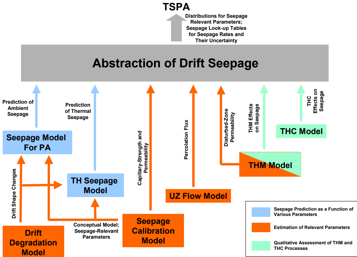
Figure 1-1. Relationship and Information Flow between Primary Process Models and the Seepage Abstraction Model
