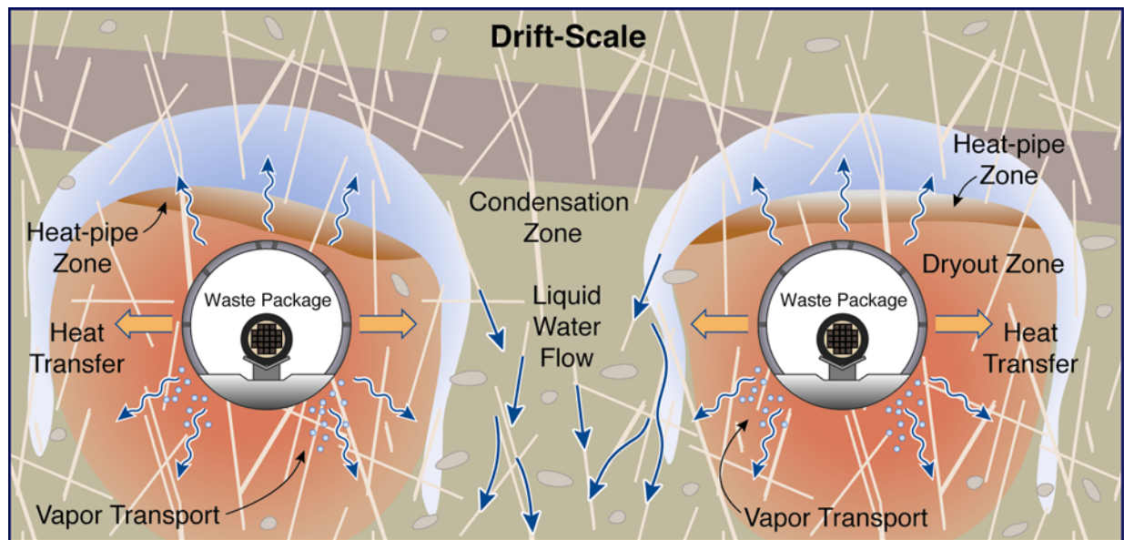
Figure 6.3-2. Schematic of TH Processes Occurring in the Drift Vicinity as a Result of Repository Heating (not to scale)
