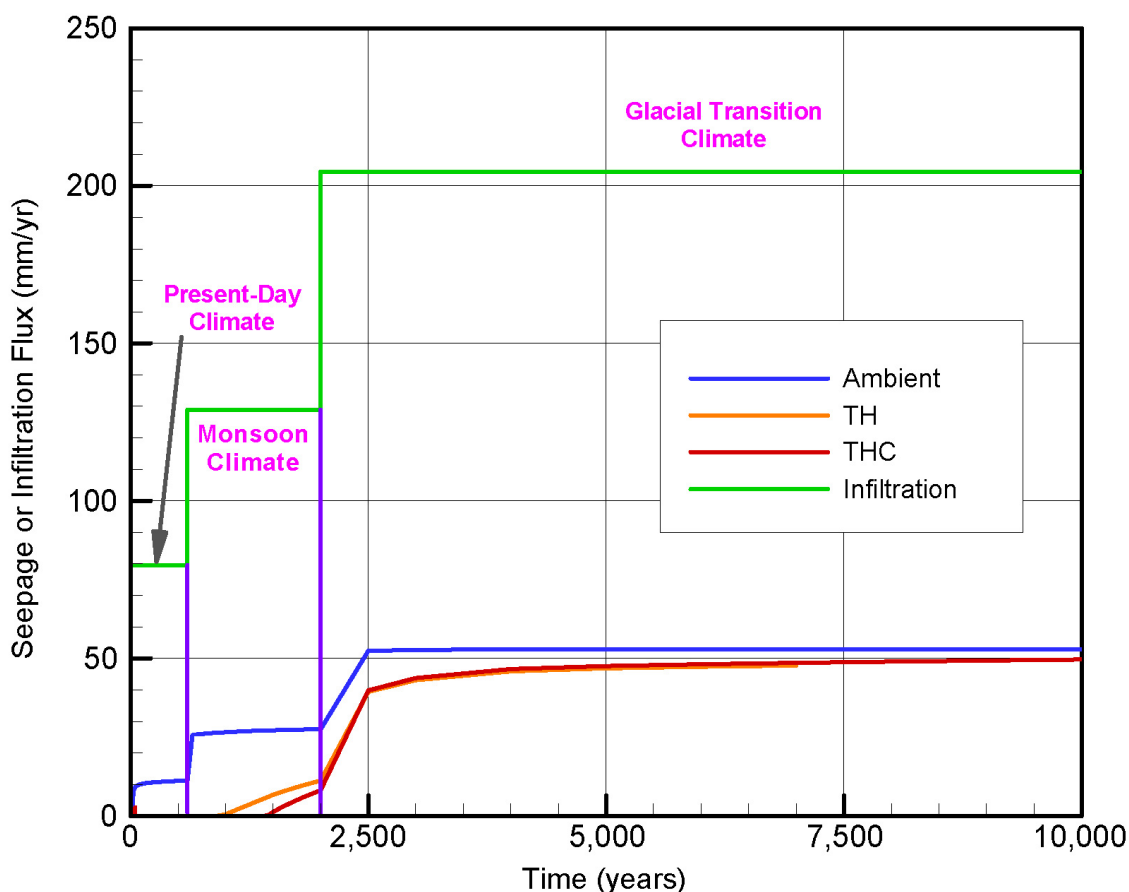
Figure 6-19[a]. Comparison of Seepage Fluxes from Ambient, TH, and THC Simulations for a Ten-Times-Increased Percolation Flux
