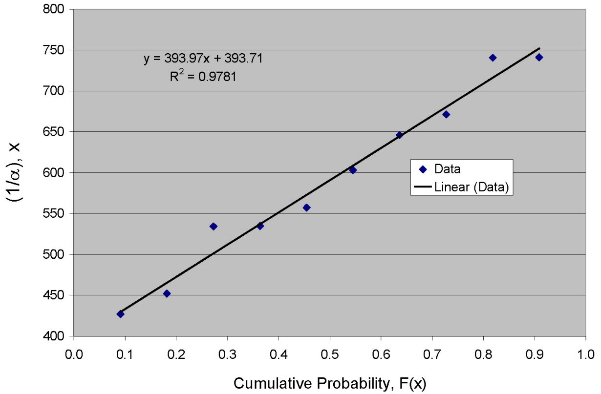
Figure 6-20[a]. Linear Regression Fit to Estimate Uniform Distribution Parameters for the Capillary-Strength Parameter
