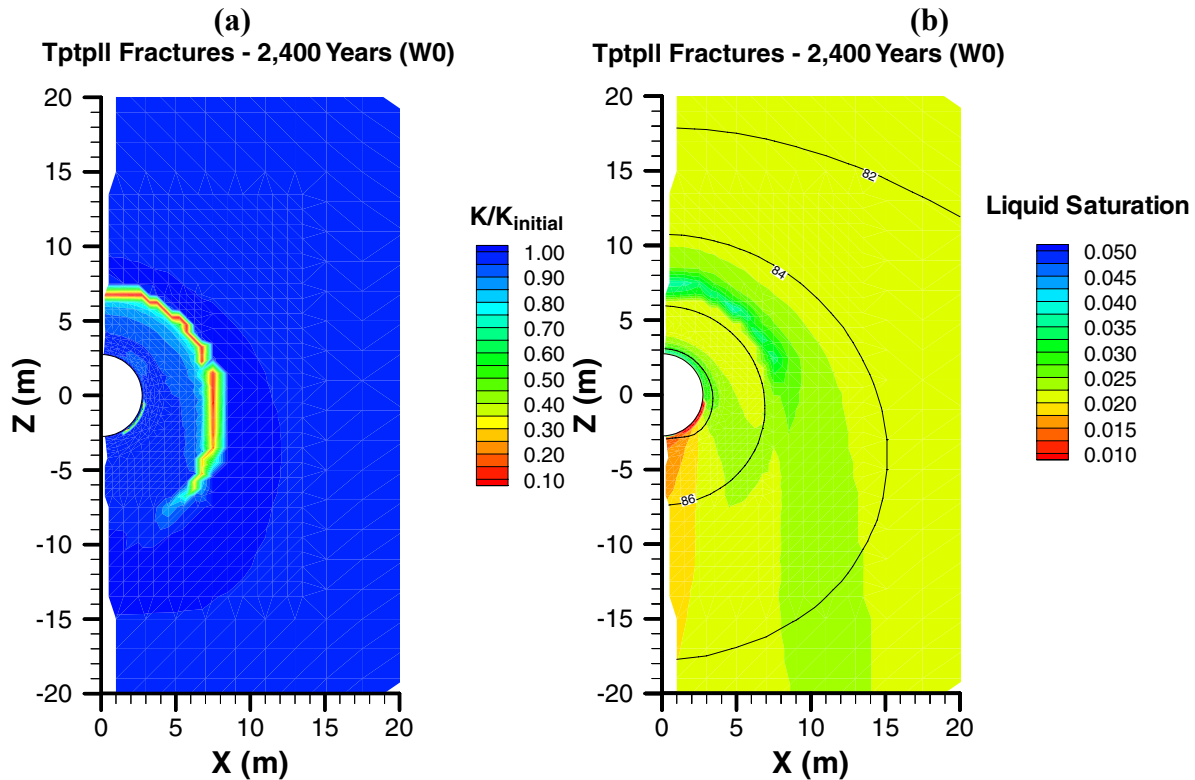
Figure 6.4-35. Example of Effects of Mineral Alteration as Predicted by the TH Seepage Model: Contour Plot of Modeled (a) Permeability Change, and (b) Liquid Saturation and Temperature Contours ( ^{\circ}\text{C} ) at 2,400 Years
