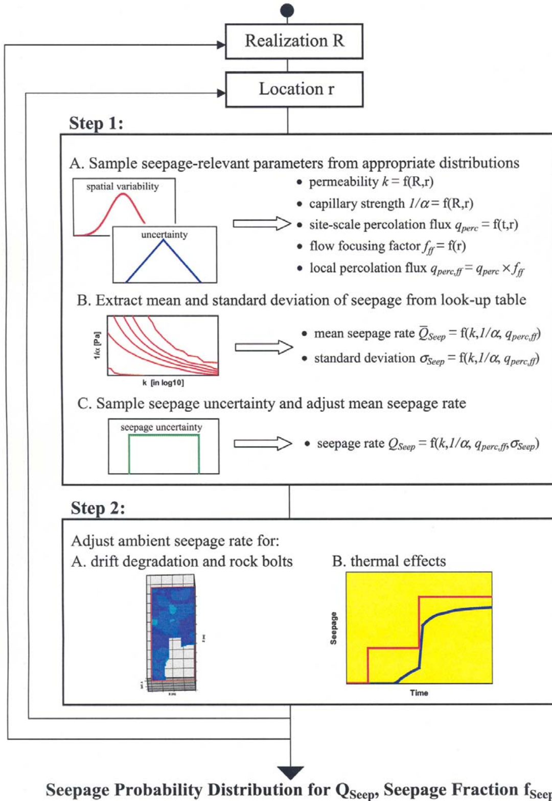
Figure 6.5-1. Schematic of Probabilistic TSPA Procedure for Calculating Seepage
