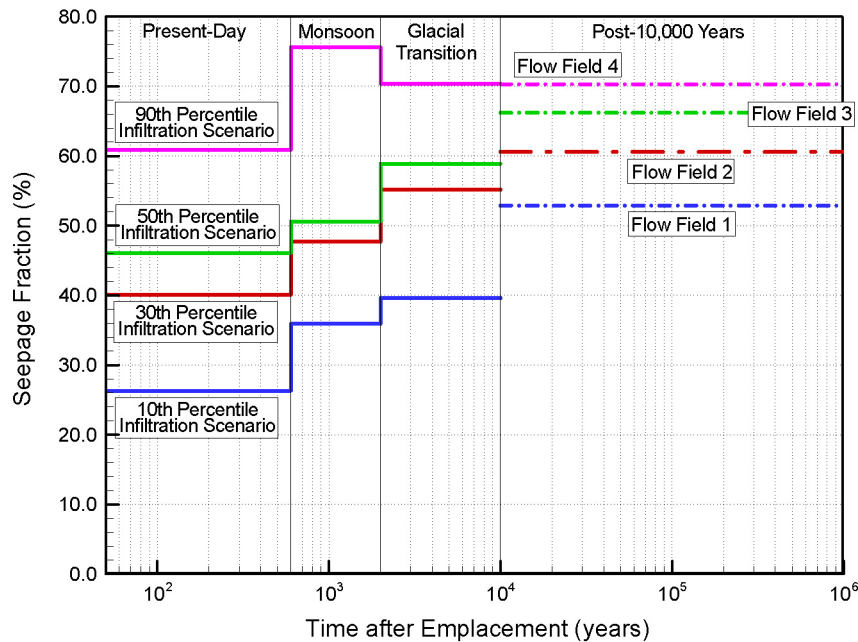
Figure 6-17[a]. Mean Seepage Percentage as a Function of Time after Emplacement for Collapsed Drift in Tptpl Unit and Different Infiltration Scenarios
