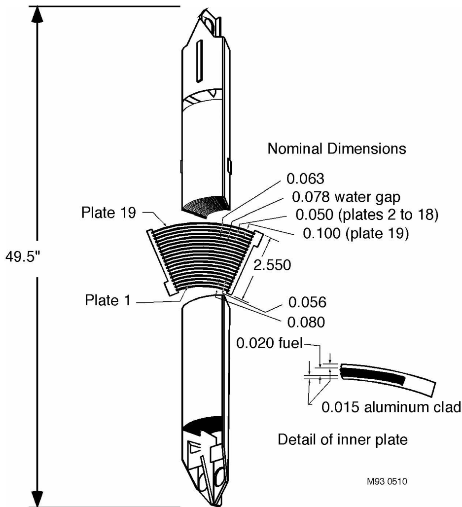
Figure 11. Simplified View of the ATR Fuel Element
