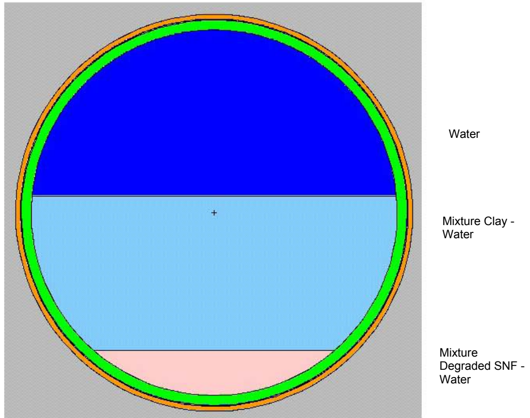
Figure 1010. Cross-sectional View of the Waste Package Containing All Components Degraded Settled in Layers
