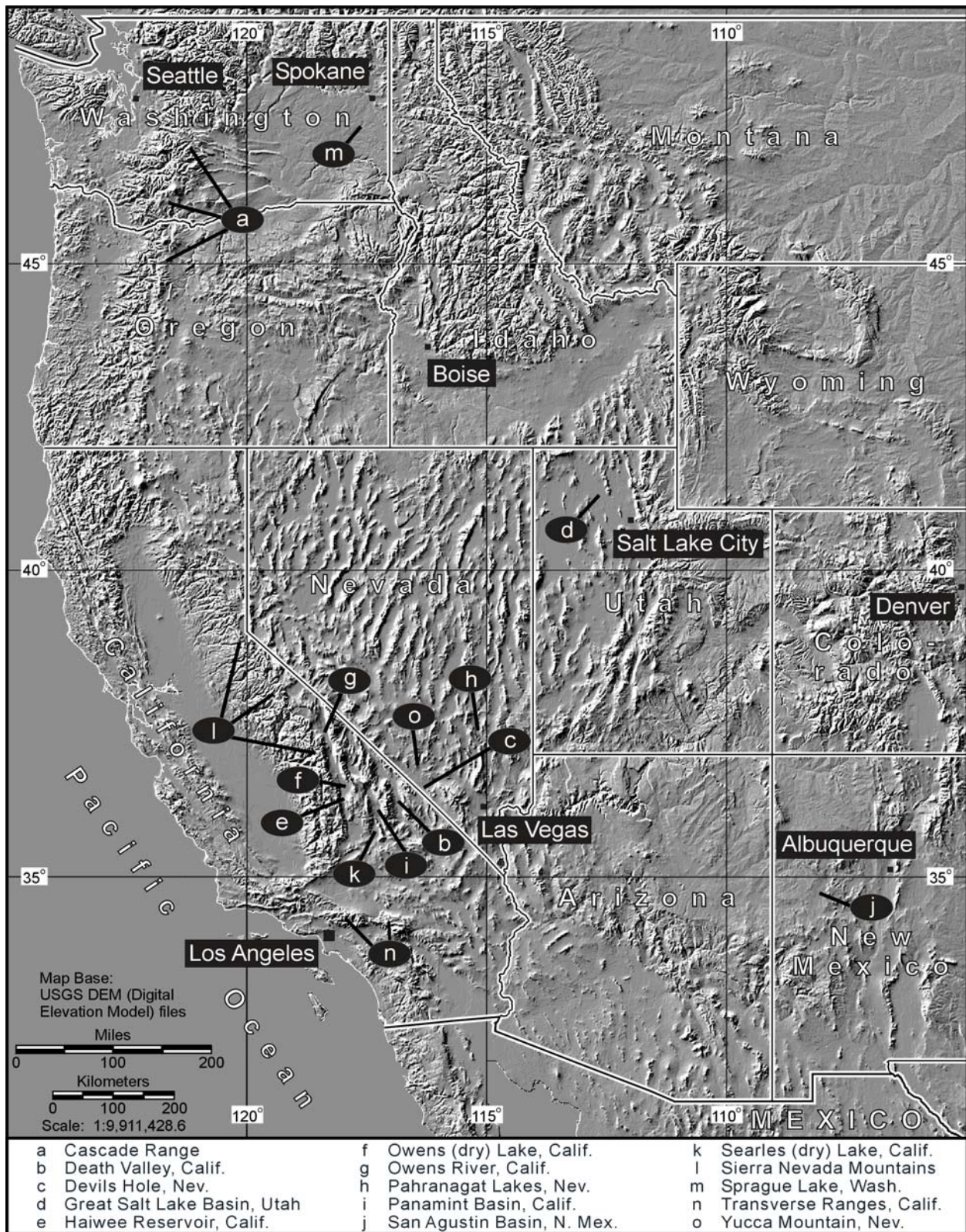
Figure 6-1. Western United States Showing Localities Discussed in the Text
