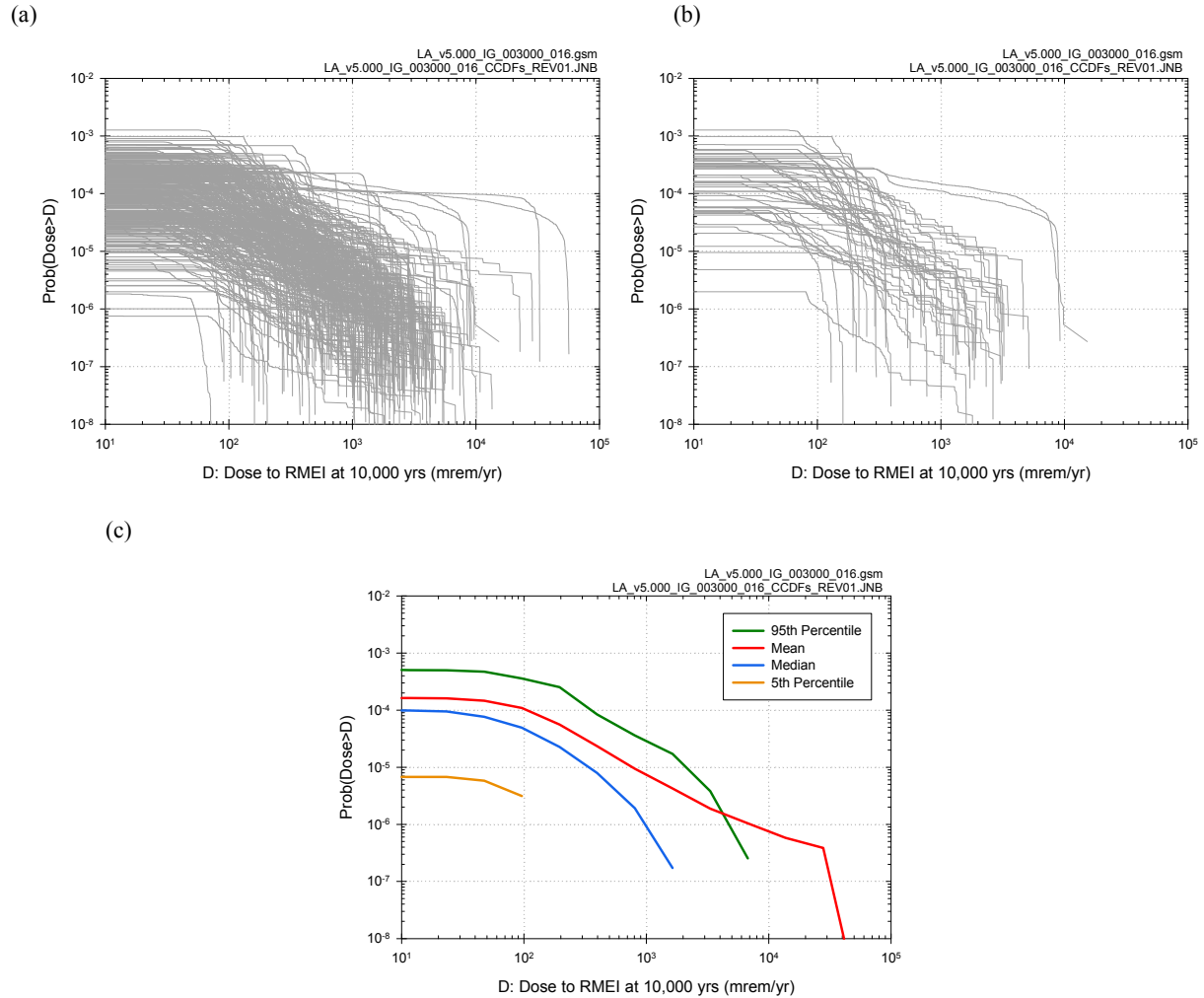
Figure J7.2-9. Results associated with D_{II}(10^4 \text{ yr}|\mathbf{a}_{II}, \mathbf{e}_M) obtained with sampling-based (Monte Carlo) procedures for an LHS of size nLHS = 300 : (a) CCDFs for D_{II}(10^4 \text{ yr}|\mathbf{a}_{II}, \mathbf{e}_{Mi}) with exceedance probabilities p_A[D < D_{II}(10^4 \text{ yr}|\mathbf{a}_{II}, \mathbf{e}_{Mi})|\mathbf{a}_{Ai}] defined in Equation J7.2-23 for i = 1, 2, \dots, nLHS = 300 , (b) CCDFs for D_{II}(10^4 \text{ yr}|\mathbf{a}_{II}, \mathbf{e}_{Mi}) with exceedance probabilities p_A[D < D_{II}(10^4 \text{ yr}|\mathbf{a}_{II}, \mathbf{e}_{Mi})|\mathbf{a}_{Ai}] defined in Equation J7.2-23 for i = 1, 2, \dots, 50 , and (c) expected (mean) CCDF and quantile curves, q = 0.05, 0.5, 0.95 , for CCDFs in (a).
