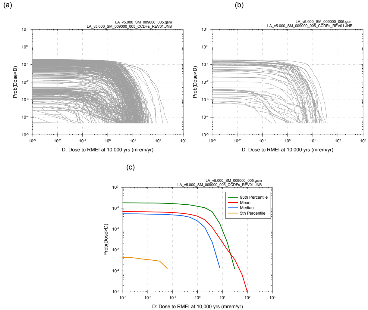
Figure J8.3-10. Results associated with D_{SG}(10^4 \text{ yr} | \mathbf{a}_{SG}, \mathbf{e}_M) obtained with sampling-based (Monte Carlo) procedures for an LHS of size nLHS = 300 : (a) CCDFs for D_{SG}(10^4 \text{ yr} | \mathbf{a}_{SG}, \mathbf{e}_{Mi}) with exceedance probabilities p_A[D < D_{SG}(10^4 \text{ yr} | \mathbf{a}, \mathbf{e}_{Mi}) | \mathbf{e}_{Ai}] defined in Equation J4.5-19 for i = 1, 2, \dots, nLHS = 300 , (b) CCDFs for D_{SG}(10^4 \text{ yr} | \mathbf{a}_{SG}, \mathbf{e}_{Mi}) with exceedance probabilities p_A[D < D_{SG}(10^4 \text{ yr} | \mathbf{a}, \mathbf{e}_{Mi}) | \mathbf{e}_{Ai}] defined in Equation J4.5-19 for i = 1, 2, \dots, 50 , and (c) expected (mean) CCDF and quantile curves, q = 0.05, 0.5, 0.95 , for CCDFs in (a).
