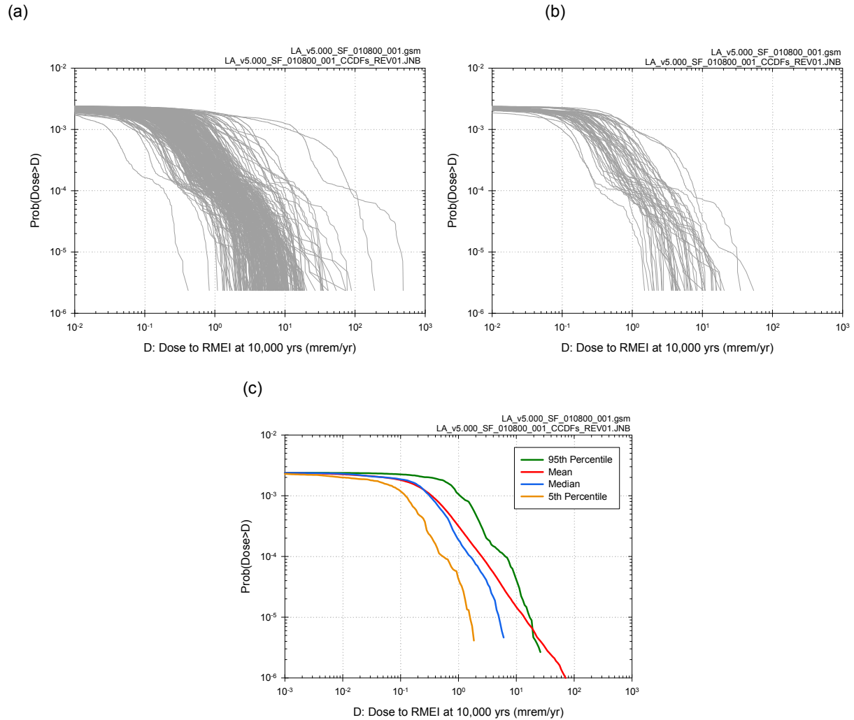
Figure J8.6-10. Results associated with D_{SF}(10^4 \text{ yr} | \mathbf{a}_{SF}, \mathbf{e}_M) obtained with sampling-based (Monte Carlo) procedures for an LHS of size n_{LHS} = 300 : (a) CCDFs for D_{SF}(10^4 \text{ yr} | \mathbf{a}_{SF}, \mathbf{e}_{Mi}) with exceedance probabilities p_A[D < D_{SF}(10^4 \text{ yr} | \mathbf{a}, \mathbf{e}_{Mi}) | \mathbf{e}_{Ai}] defined in Equation J4.5-19 for i = 1, 2, \dots, n_{LHS} = 300 , (b) CCDFs for D_{SF}(10^4 \text{ yr} | \mathbf{a}_{SF}, \mathbf{e}_{Mi}) with exceedance probabilities p_A[D < D_{SF}(10^4 \text{ yr} | \mathbf{a}, \mathbf{e}_{Mi}) | \mathbf{e}_{Ai}] defined in Equation J4.5-19 for i = 1, 2, \dots, 50 , and (c) expected (mean) CCDF and quantile curves, q = 0.05, 0.5, 0.95 , for CCDFs in (a).
