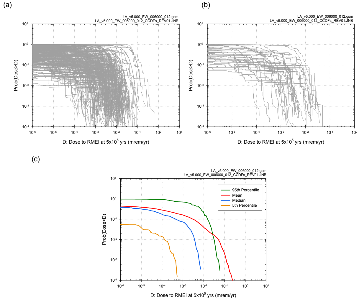
Figure J6.2-20. Results associated with D_{EW}(5 \times 10^5 \text{ yr} | \mathbf{a}_{EW}, \mathbf{e}_M) obtained with sampling-based (Monte Carlo) procedures for an LHS of size n_{LHS} = 300 : (a) CCDFs for D_{EW}(5 \times 10^5 \text{ yr} | \mathbf{a}_{EW}, \mathbf{e}_{Mi}) with exceedance probabilities p_A[D < D_{EW}(5 \times 10^5 \text{ yr} | \mathbf{a}_{EW}, \mathbf{e}_{Mi}) | \mathbf{e}_{Ai}] defined in Equation J66.2-12 for i = 1, 2, \dots, n_{LHS} = 300 , (b) CCDFs for D_{EW}(10^4 \text{ yr} | \mathbf{a}_{EW}, \mathbf{e}_{Mi}) with exceedance probabilities p_A[D < D_{EW}(5 \times 10^5 \text{ yr} | \mathbf{a}_{EW}, \mathbf{e}_{Mi}) | \mathbf{e}_{Ai}] defined in Equation J6.2-20 for i = 1, 2, \dots, 50 , and (c) expected (mean) CCDF and quantile curves, q = 0.05, 0.5, 0.95 , for CCDFs in (a).
