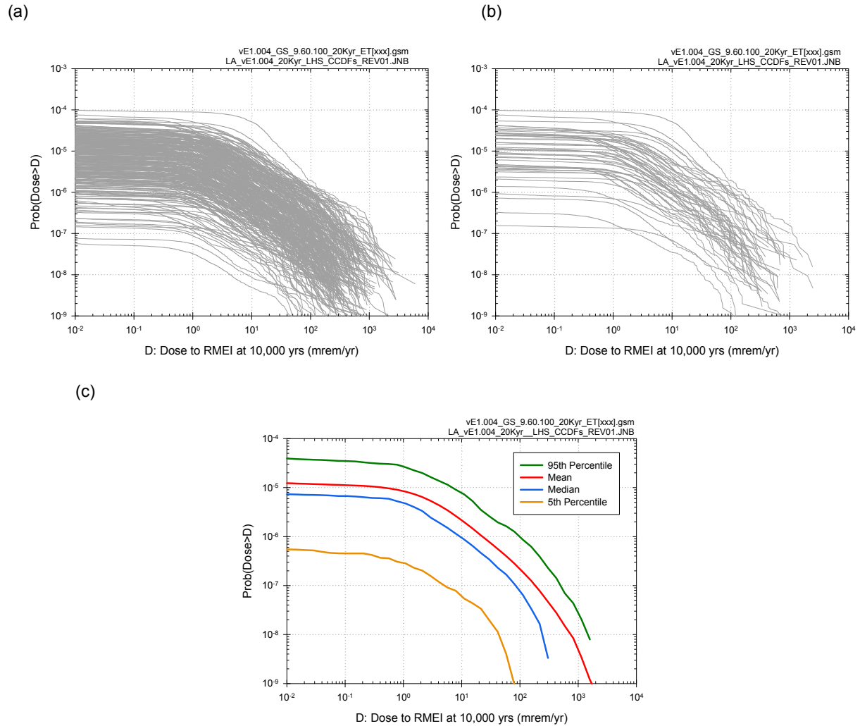
Figure J7.3-8. Results associated with D_{IE}(10^4 \text{ yr} | \mathbf{a}_{IE}, \mathbf{e}_M) obtained with sampling-based (Monte Carlo) procedures for an LHS of size nLHS = 300 : (a) CCDFs for D_{IE}(10^4 \text{ yr} | \mathbf{e}_{IE}, \mathbf{e}_{Mi}) with exceedance probabilities p_A[D < D_{IE}(10^4 \text{ yr} | \mathbf{a}, \mathbf{e}_{Mi}) | \mathbf{e}_{Ai}] defined in Equation J7.3-20 for i = 1, 2, \dots, nLHS = 300 , (b) CCDFs for D_{IE}(10^4 \text{ yr} | \mathbf{a}_{IE}, \mathbf{e}_{Mi}) with exceedance probabilities p_A[D < D_{IE}(10^4 \text{ yr} | \mathbf{a}, \mathbf{e}_{Mi}) | \mathbf{e}_{Ai}] defined in Equation J7.3-20 for i = 1, 2, \dots, 50 , and (c) expected (mean) CCDF and quantile curves, q = 0.05, 0.5, 0.95 , for CCDFs in (a).
