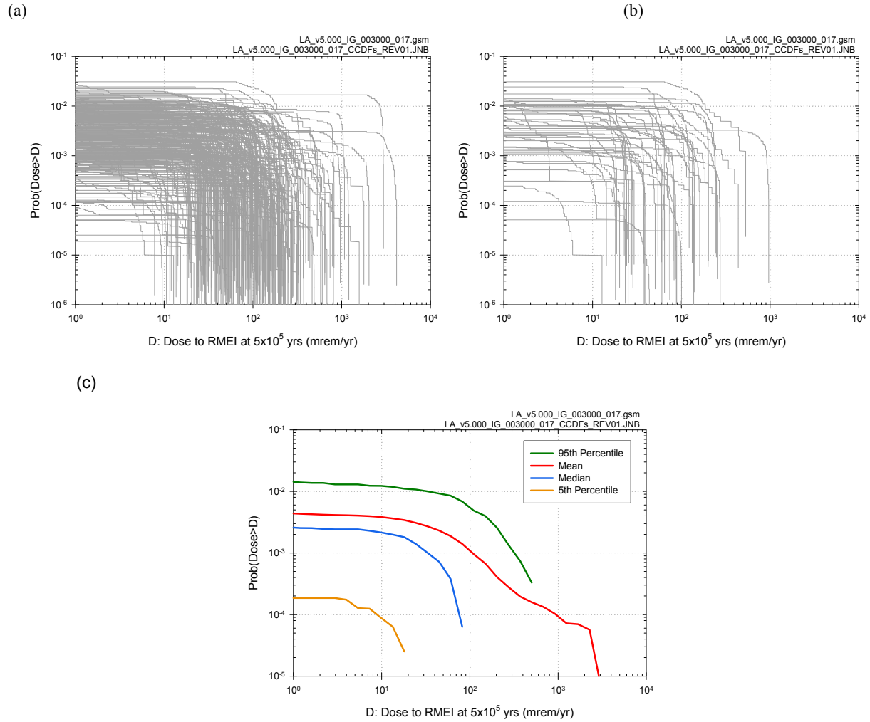
Figure J7.2-19. Results associated with D_{IJ}(5 \times 10^5 \text{ yr} | \mathbf{a}_{IJ}, \mathbf{e}_M) obtained with sampling-based (Monte Carlo) procedures for an LHS of size nLHS = 300 : (a) CCDFs for D_{IJ}(5 \times 10^5 \text{ yr} | \mathbf{a}_{IJ}, \mathbf{e}_{Mi}) with exceedance probabilities p_A[D < D_{IJ}(5 \times 10^5 \text{ yr} | \mathbf{a}, \mathbf{e}_{Mi}) | \mathbf{e}_{Ai}] defined in Equation J7.2-23 for i = 1, 2, \dots, nLHS = 300 , (b) CCDFs for D_{IJ}(5 \times 10^5 \text{ yr} | \mathbf{a}_{IJ}, \mathbf{e}_{Mi}) with exceedance probabilities p_A[D < D_{IJ}(5 \times 10^5 \text{ yr} | \mathbf{a}, \mathbf{e}_{Mi}) | \mathbf{a}_{Ai}] defined in Equation J7.2-23 for i = 1, 2, \dots, 50 , and (c) expected (mean) CCDF and quantile curves, q = 0.05, 0.5, 0.95 , for CCDFs in (a).
