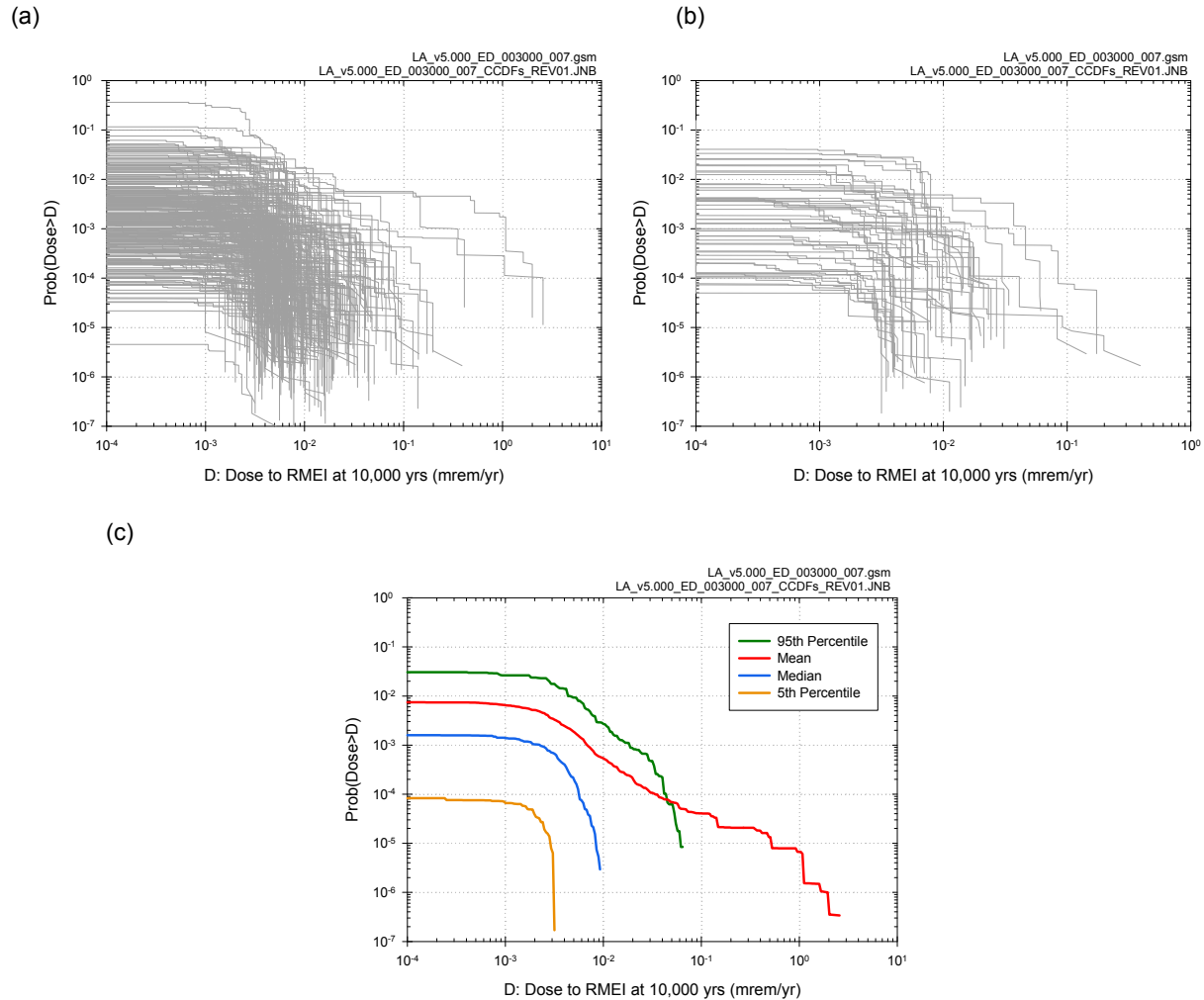
Figure J6.3-10. Results associated with D_{ED}(10^4 \text{ yr} | \mathbf{a}_{ED}, \mathbf{e}_M) obtained with sampling-based (Monte Carlo) procedures for an LHS of size nLHS = 300 : (a) CCDFs for D_{ED}(10^4 \text{ yr} | \mathbf{a}_{ED}, \mathbf{e}_{Mi}) with exceedance probabilities p_A[D < D_{ED}(10^4 \text{ yr} | \mathbf{a}_{ED}, \mathbf{e}_{Mi}) | \mathbf{e}_{Ai}] defined similarly to p_A[D < D_{EW}(\tau | \mathbf{a}, \mathbf{e}_{M1}) | \mathbf{e}_{A1}] in Equation (J6.2-12) for i = 1, 2, \dots, nLHS = 300 , (b) CCDFs for D_{ED}(10^4 \text{ yr} | \mathbf{a}_{ED}, \mathbf{e}_{Mi}) with exceedance probabilities p_A[D < D_{ED}(10^4 \text{ yr} | \mathbf{a}_{ED}, \mathbf{e}_{Mi}) | \mathbf{e}_{Ai}] defined similarly to p_A[D < D_{EW}(\tau | \mathbf{a}, \mathbf{e}_{M1}) | \mathbf{e}_{A1}] in Equation (J6.2-12) for i = 1, 2, \dots, 50 , and (c) expected (mean) CCDF and quantile curves, q = 0.05, 0.5, 0.95 , for CCDFs in (a).
