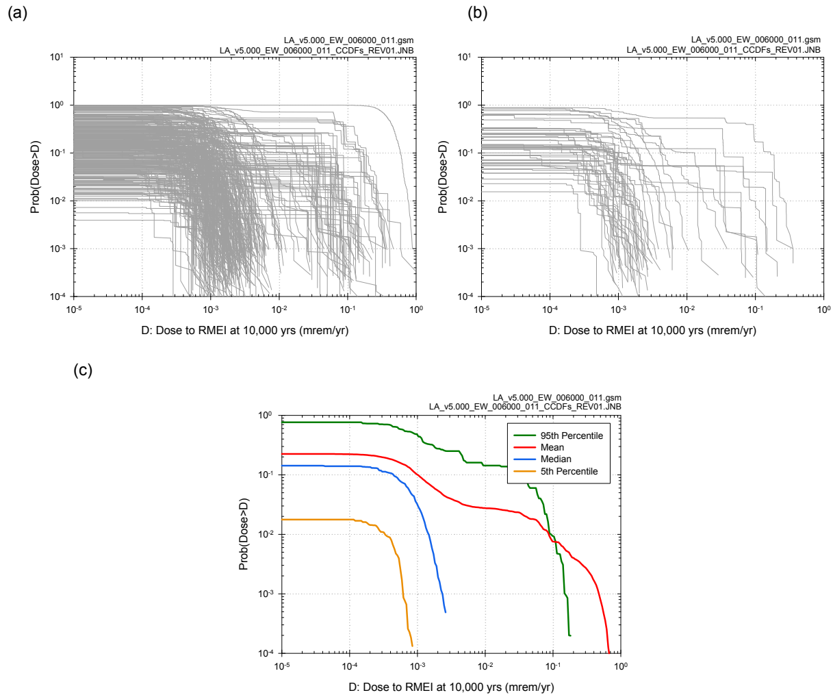
Figure J6.2-10. Results associated with D_{EW}(10^4 \text{ yr} | \mathbf{a}_{EW}, \mathbf{e}_M) obtained with sampling-based (Monte Carlo) procedures for an LHS of size nLHS = 300 : (a) CCDFs for D_{EW}(10^4 \text{ yr} | \mathbf{a}_{EW}, \mathbf{e}_{Mi}) with exceedance probabilities p_A[D < D_{EW}(10^4 \text{ yr} | \mathbf{a}, \mathbf{e}_{Mi}) | \mathbf{e}_{Ai}] defined in Equation J6.2-12 for i = 1, 2, \dots, nLHS = 300 , (b) CCDFs for D_{EW}(10^4 \text{ yr} | \mathbf{a}_{EW}, \mathbf{e}_M) with exceedance probabilities p_A[D < D_{EW}(10^4 \text{ yr} | \mathbf{a}, \mathbf{e}_{Mi}) | \mathbf{e}_{Ai}] defined in Equation J6.2-13 for i = 1, 2, \dots, 50 , and (c) expected (mean) CCDF and quantile curves, q = 0.05, 0.5, 0.95 , for CCDFs in (a).
