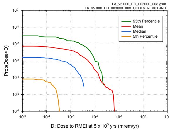
Figure J6.3-20. Results associated with D_{ED}(5 \times 10^5 \text{ yr} | \mathbf{a}_{ED}, \mathbf{e}_M) obtained with sampling-based (Monte Carlo) procedures for an LHS of size nLHS = 300 : (a) CCDFs for D_{ED}(5 \times 10^5 \text{ yr} | \mathbf{a}_{ED}, \mathbf{e}_{Mi}) with exceedance probabilities p_A[D < D_{ED}(5 \times 10^5 \text{ yr} | \mathbf{a}_{ED}, \mathbf{e}_{Mi}) | \mathbf{e}_{Ai}] defined similarly to p_A[D < D_{EW}(\tau | \mathbf{a}, \mathbf{e}_{M1}) | \mathbf{e}_{A1}] in Equation (J6.2-12) for i = 1, 2, \dots, nLHS = 300 , (b) CCDFs for D_{ED}(10^4 \text{ yr} | \mathbf{a}_{ED}, \mathbf{e}_{Mi}) with exceedance probabilities p_A[D < D_{ED}(5 \times 10^5 \text{ yr} | \mathbf{a}_{ED}, \mathbf{e}_{Mi}) | \mathbf{e}_{Ai}] defined similarly to p_A[D < D_{EW}(\tau | \mathbf{a}, \mathbf{e}_{M1}) | \mathbf{e}_{A1}] in Equation (J6.2-12) for i = 1, 2, \dots, 50 , and (c) expected (mean) CCDF and quantile curves, q = 0.05, 0.5, 0.95 , for CCDFs in (a).
