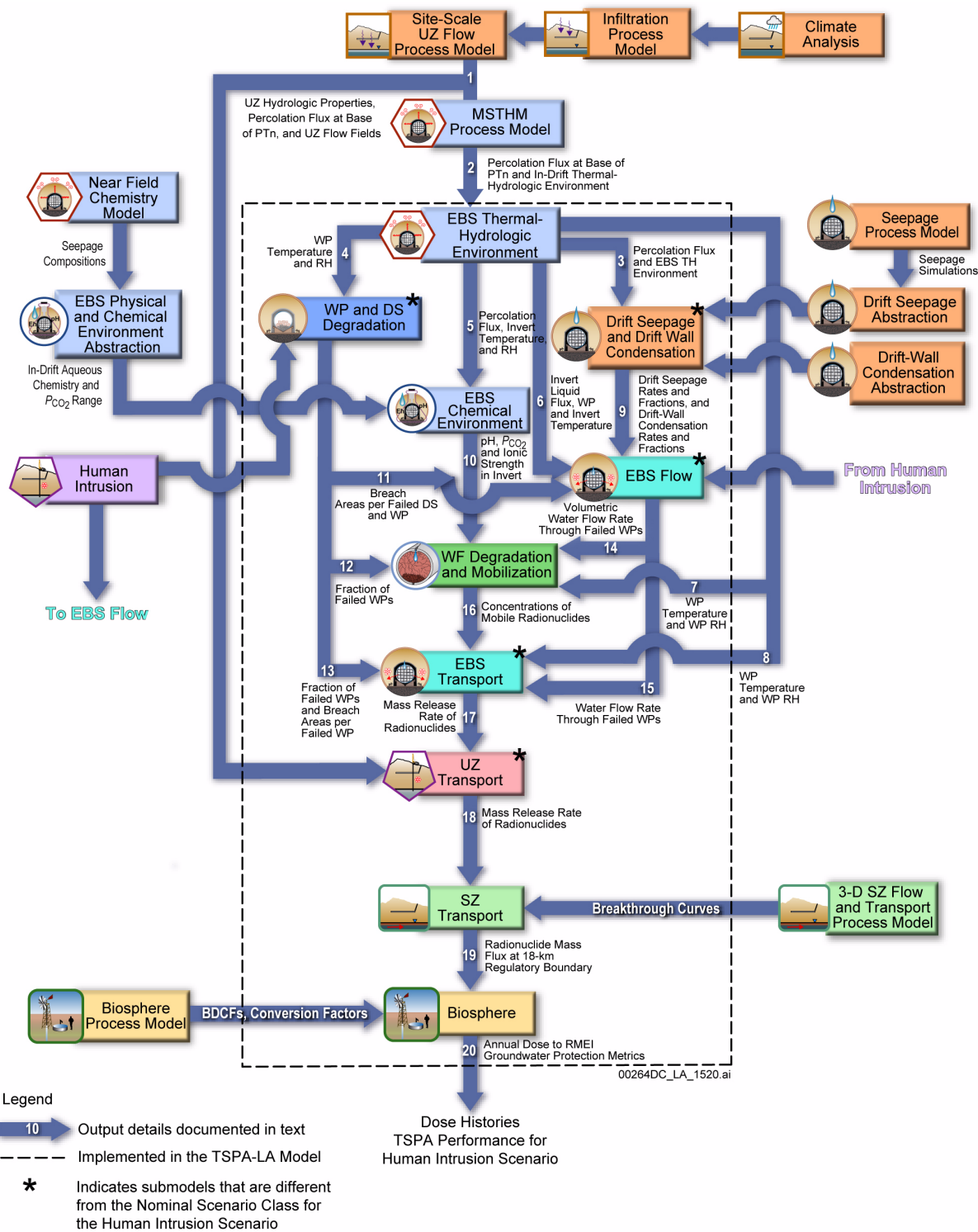
Figure 2.4-158. Information Transfer between the Model Components and Submodels of the TSPA Human Intrusion Scenario
