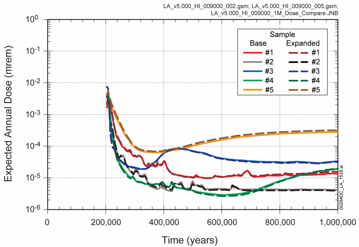
Figure 2.4-161. Expected Annual Dose over 1 Million Years for the Human Intrusion Modeling Case Considering Increased Aleatory Sample Size
