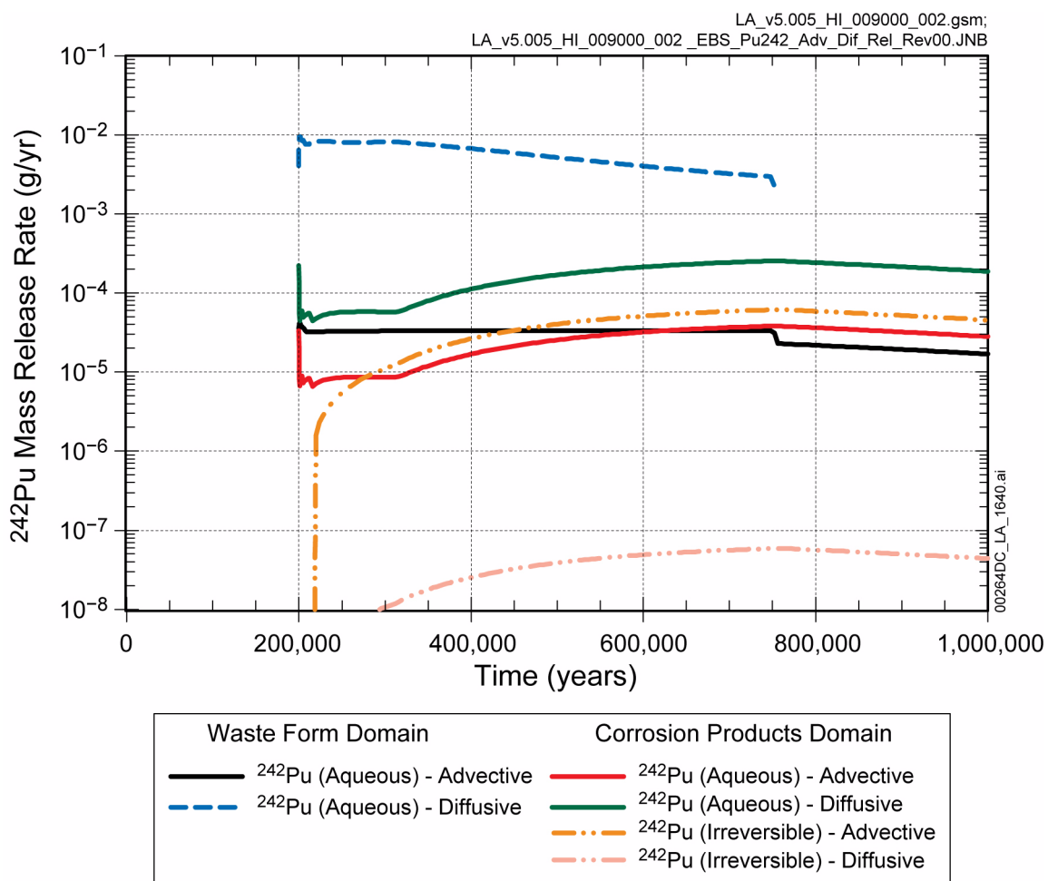
Figure 2.4-167. Advective and Diffusive Release Rates of ^{242}\text{Pu} (Aqueous) from Waste Form and Corrosion Products Domain and ^{242}\text{Pu} (Irreversibly Sorbed on Iron Oxyhydroxide Colloids) from Corrosion Products Domain for Failed Commercial SNF Waste Packages for Realization 8,309 of the Human Intrusion Modeling Case for the 1-Million-Year Period after Repository Closure
