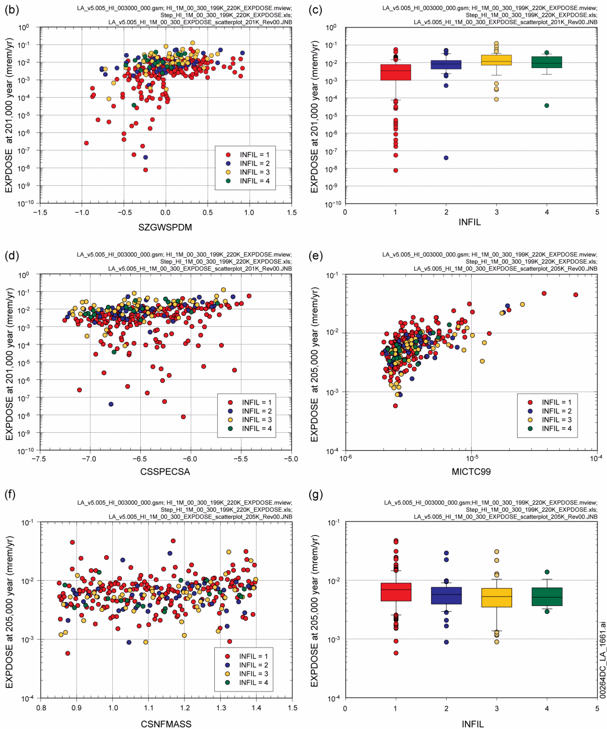
Figure 2.4-174. Stepwise Rank Regression Analyses and Selected LA Scatterplots for Expected Dose to the RMEI ( EXPDOSE , mrem) over [200,000, 220,000 Year] Resulting from a Human Intrusion Event at 200,000 Years: (a) Regressions for EXPDOSE at 201,000, 203,000 and 205,000 Years, (b,c,d) Scatterplots for EXPDOSE at 201,000 Years, and (e, f, g) Scatterplots for EXPDOSE at 205,000 Years (Continued)
