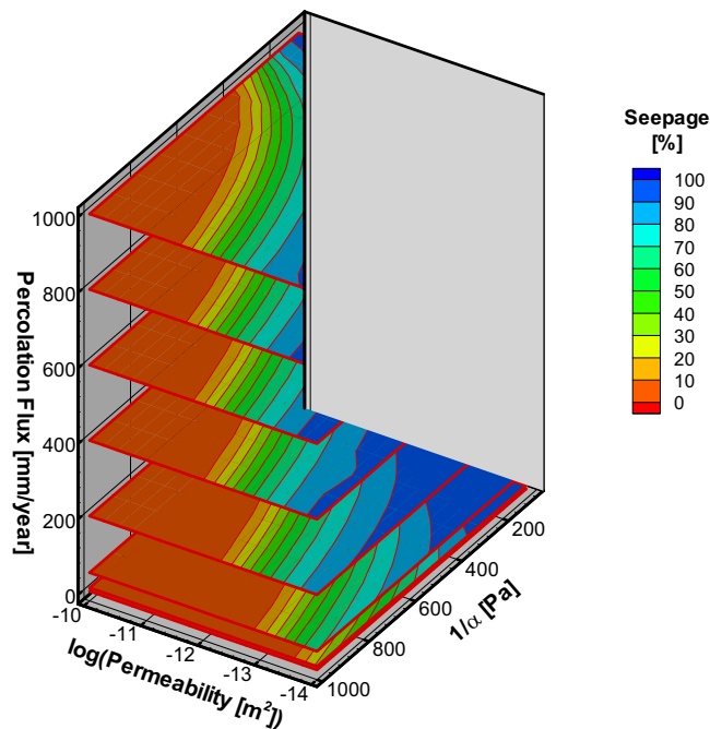
Figure 6-7. The Mean of Seepage Percentage on Vertical Planes of Permeability Field for \log_{10}(k_{FC} \text{ [m}^2\text{)}) = -14, -13, -12, -11, \text{ and } -10
