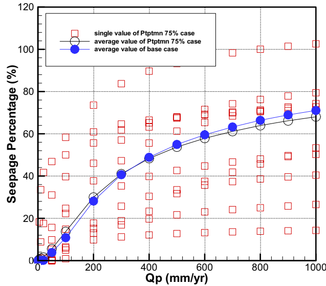
Figure 6-15. Seepage Percentage as a Function of Percolation Flux for the 75 Percentile Case Profile in Tptpmn Unit [ \log_{10}(k_{FC} [m^2]) = -11.86 , 1/\alpha = 600 Pa]. Red Open Squares Are Results for 10 Realizations. The Mean Seepage Percentages Are Shown as Black Open Circles (See Text). For Comparison, the Mean over 10 Realizations for No-Degradation Case (Base Case) Is Shown as Blue Filled Circles
