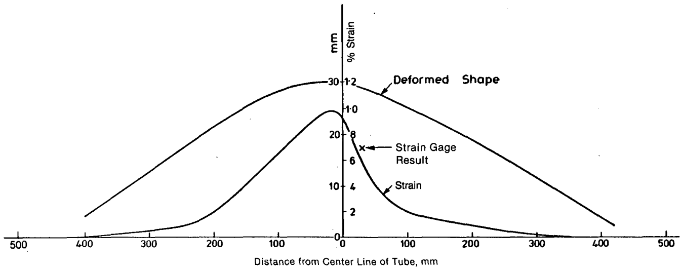
Figure 4 Deformed shape and permanent strain after tests Source: Reference 7.
