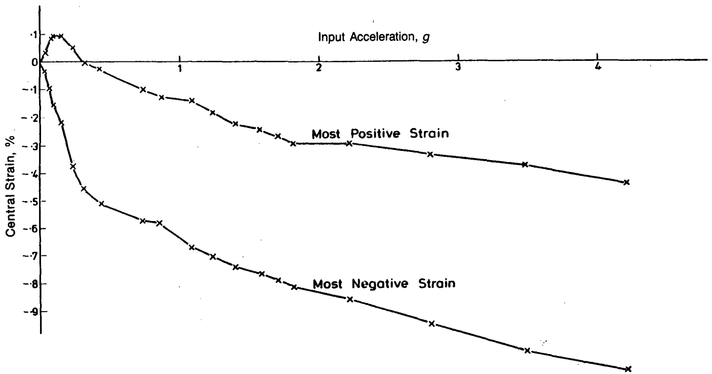
Figure 3 Strain at pipe midspan versus input acceleration Source: Reference 7.
