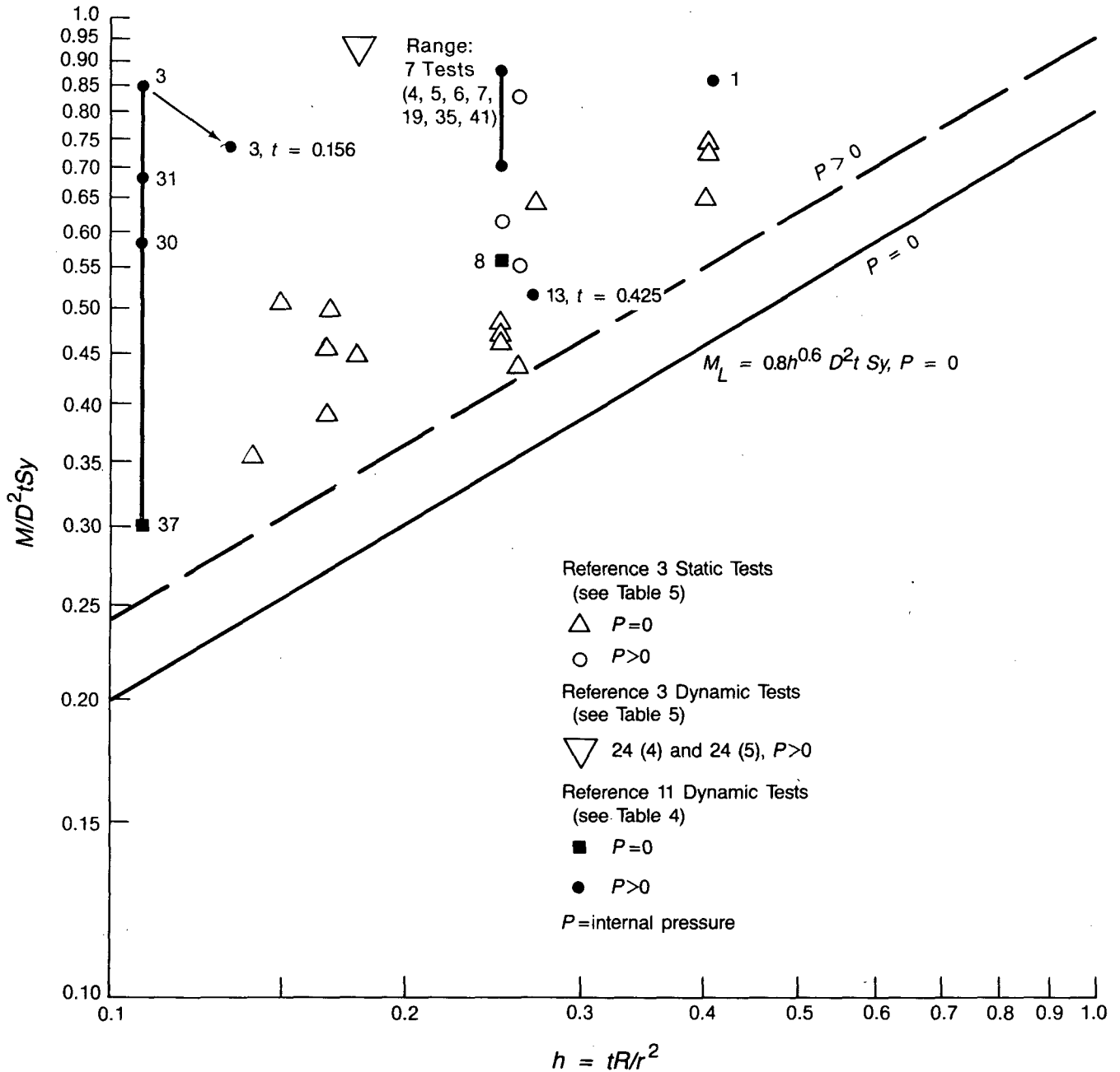
Figure 12 Elbows: Static in-plane closing moment capacity and dynamic in-plane moment capacity tests Source: References 3 and 11.
