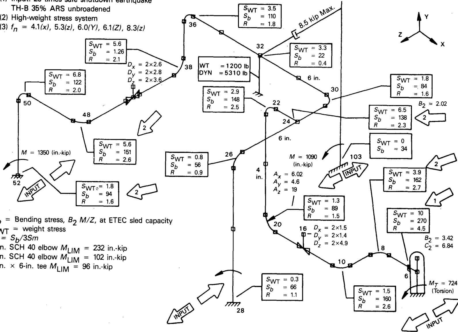
Figure 19 Piping System 2, weight stresses, S_{WT} Source: Reference 13.
