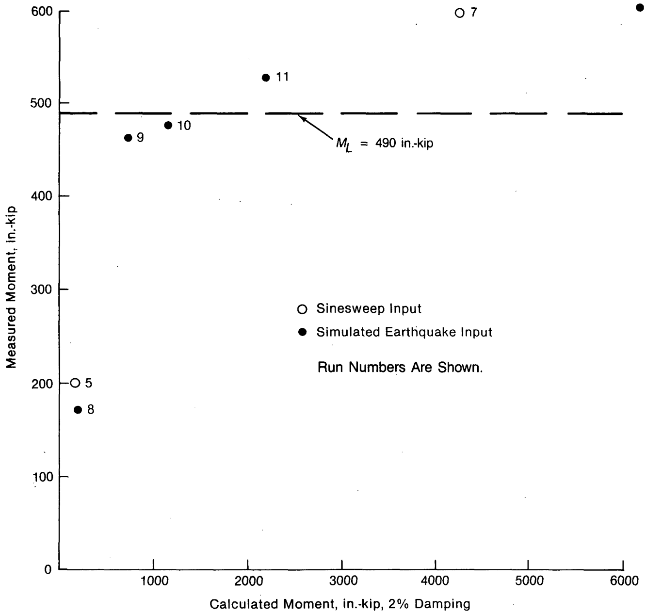
Figure 9 6 NPS, Sch. 40 carbon steel pipe, Test 34 Source: Reference 11.
