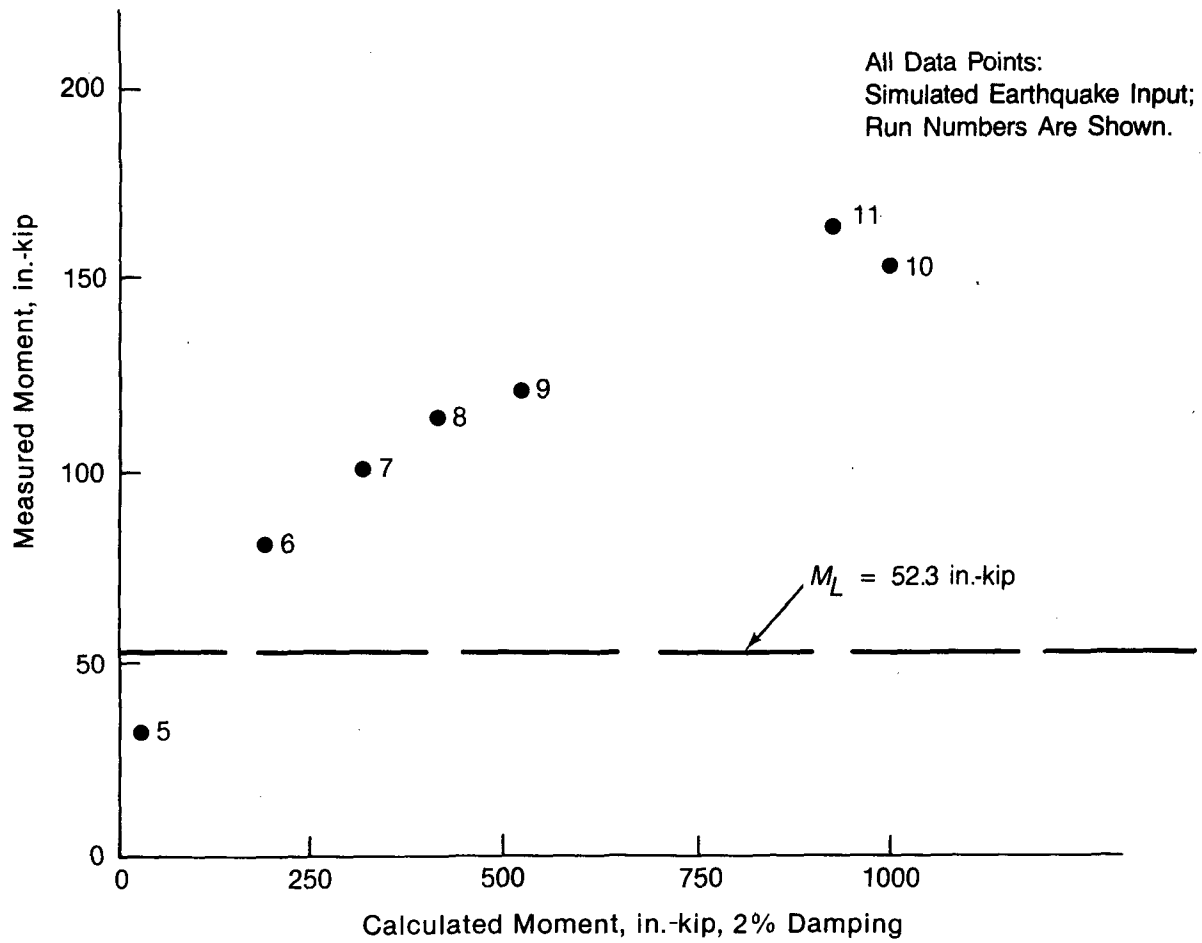
Figure 10 6 NPS, 9-in. bend radius, Sch. 10 stainless steel elbow, Test 3 Source: Reference 11.
