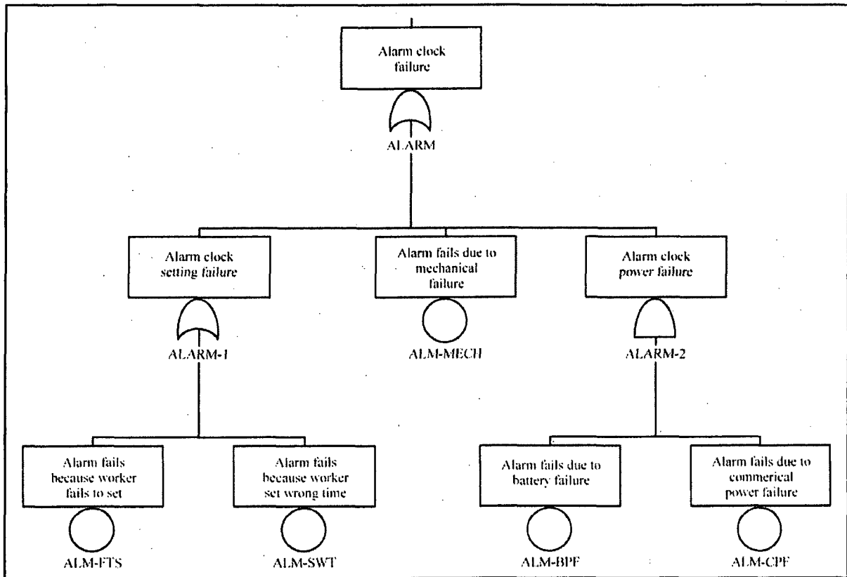
Figure 3-2 Alarm clock failure fault tree
