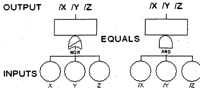
Figure 11 Equivalence for the NOR gate
