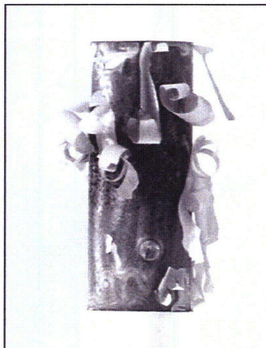
Oxidation of a foreign niobium-bearing cladding alloy under LOCA conditions
