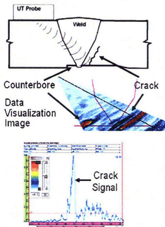
Schematic view of flaw detection at far side of weld using phased array ultrasonic (PA-UT) technique
