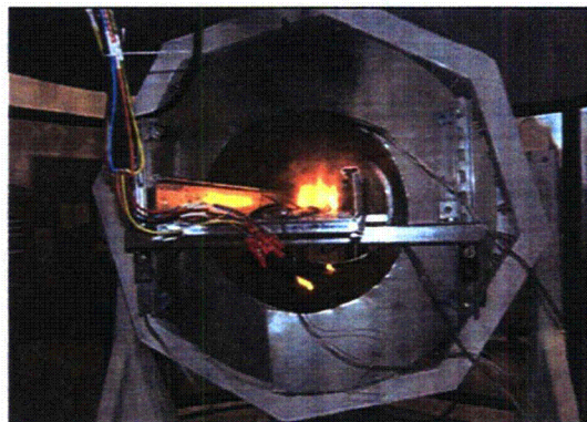
The "small-scale" (Penlight) radiant heating test facility at SNL, shown testing two multi-conductor cables for the US NRC's CAROLFIRE program
