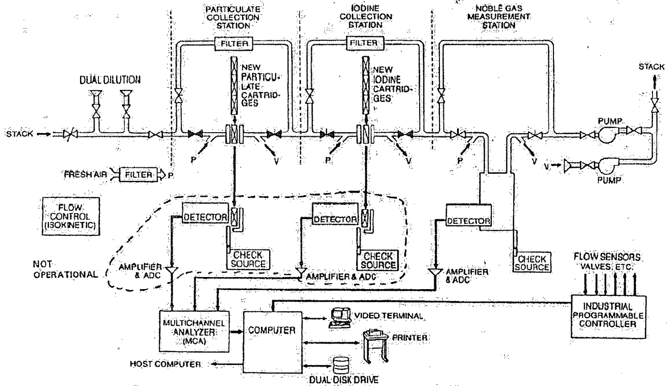
BLOCK DIAGRAM TYPICAL GASEOUS EFFLUENT MONITORING SYSTEM
