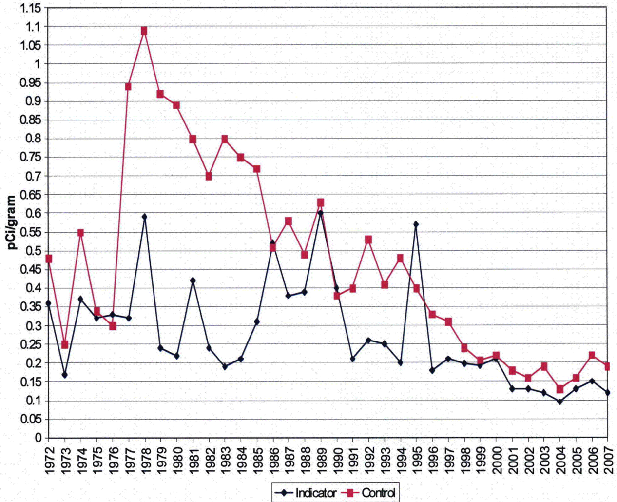
Figure 15: The concentration of Cesium-137 in soil has steadily declined in recent years. The peak seen in 1978 was due to fallout from nuclear weapons testing.
