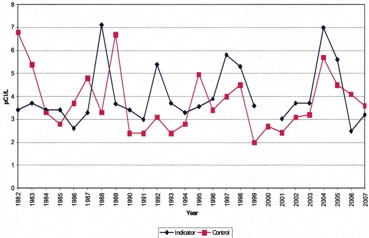
Figure 14: Shown above are the annual averages for gross beta in groundwater from 1982-2007. There were no known indicator samples available in 2000.
