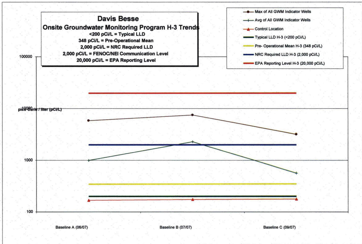
Figure 30. Groundwater Monitoring 2007
