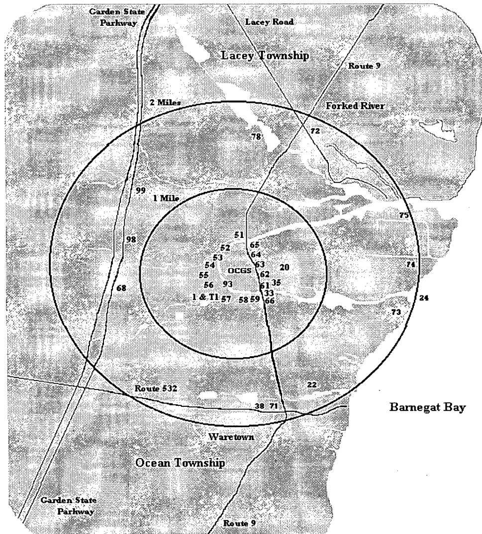
Oyster Creek Generating Station (OCGS) Locations of Radiological Environmental Monitoring Program (REMP) Stations within two miles of the OCGS
