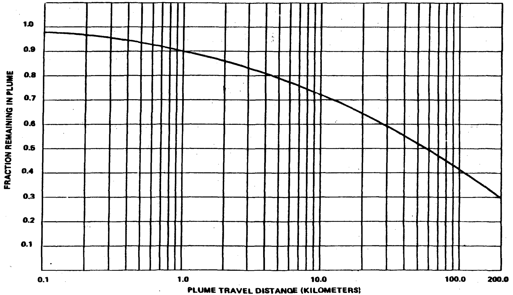
Figure 2.2 Plume Depletion Effect for Ground-Level Releases
