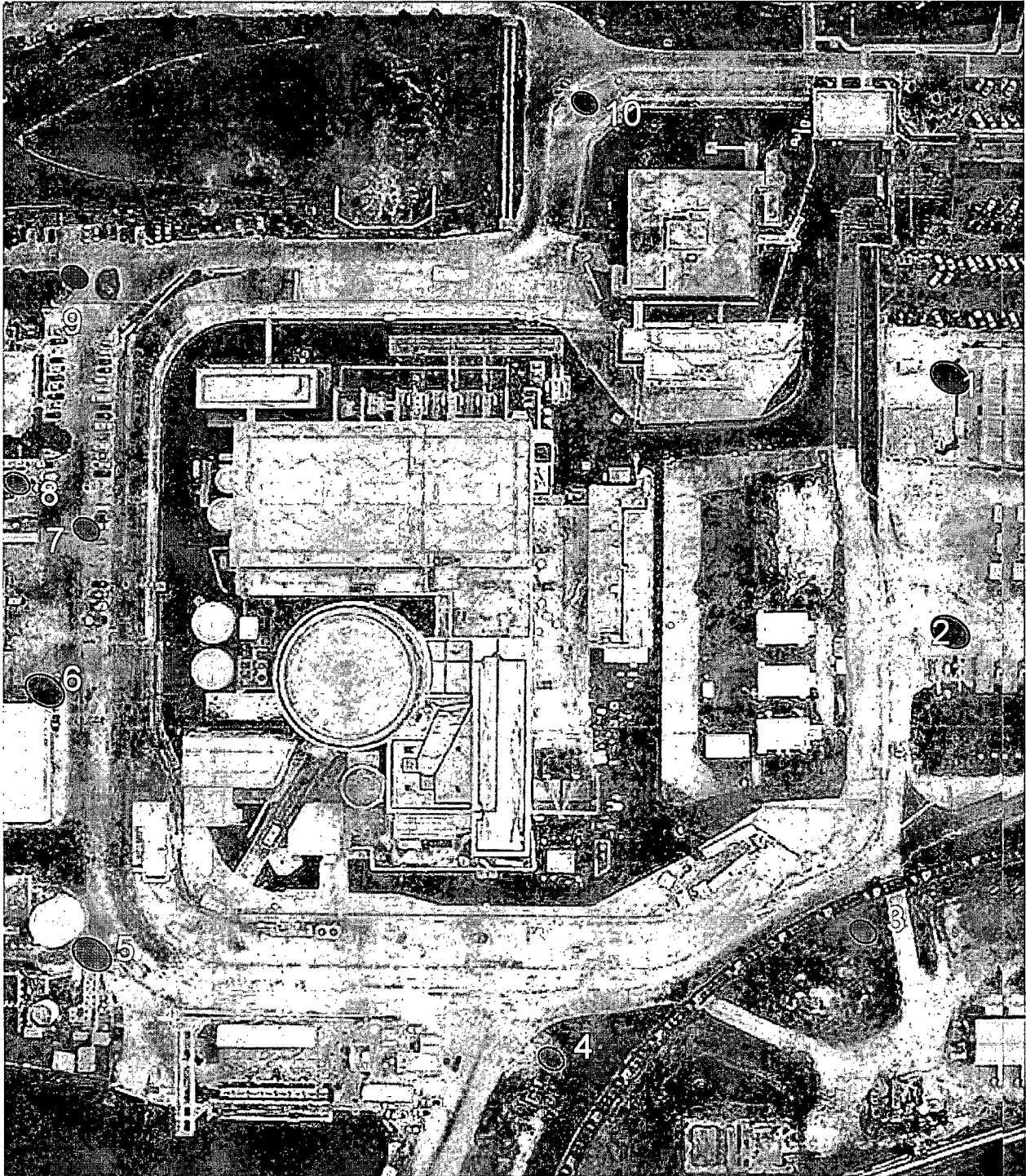
FIGURE 5.4 CR3 Groundwater Monitoring Well Locations Deep Wells Are Also Installed at #'s 1, 3, 6
