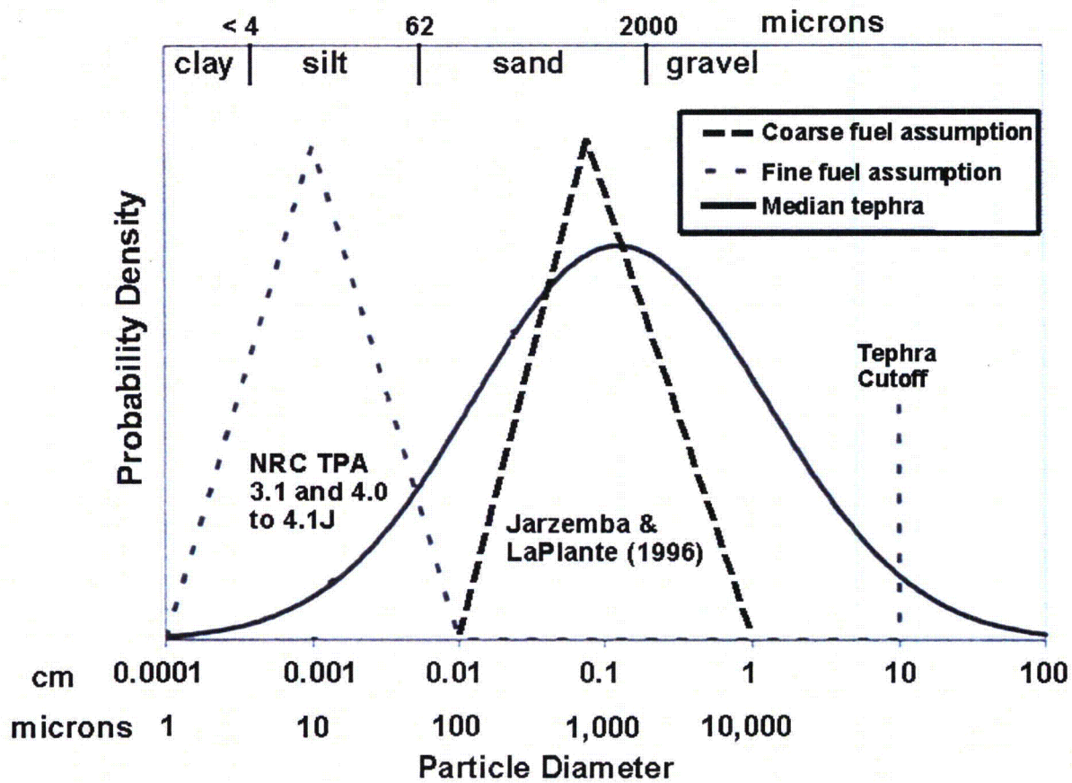
Figure 58 Median tephra diameter distribution plotted with spent fuel particle size distributions used in TPA versions 3.1 to 4.1. For comparison the size distribution suggested by Jarzempa and LaPlante (1996) is also shown. The Wentworth scale of particle sizes appears at top of figure for comparison. The intermediate size distribution used by Codell (2004) is not shown, but is a triangular distribution that ranges from 10 to 1000 microns. The distribution for median tephra particle diameter is a sampled parameter in the TPA code. The distribution of tephra particle sizes was postulated by Hill et al. (1998) based on data from the 1995 Cerro Negro eruption (Codell, 2004). The tephra “cutoff” identifies the maximum particle size that can be transported through convective dispersal (Mohanty et al., 2002, p. A-165). Particles larger than 10 cm would fall in close proximity to the volcanic vent.
