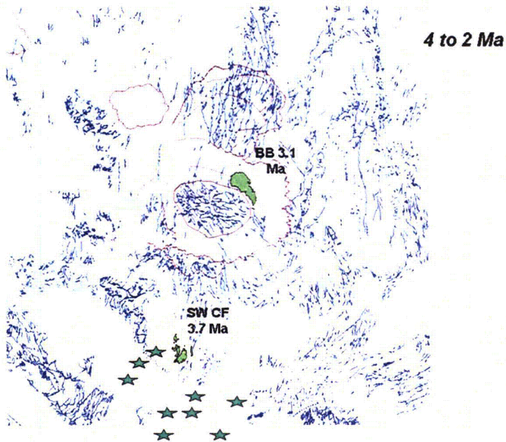
Figure 9 Actual basaltic volcanism during the period 4 to 2 Ma in the Yucca Mountain region. Exposed basalts of this age range are shown in green and green stars are magnetic anomalies that are interpreted to have a source of basaltic volcanism during this time interval. Note the significant spatial displacement of much the volcanism during this period from the basaltic rocks of the previous 2 Myr (Figure 8) (After Crowe, 2005).
