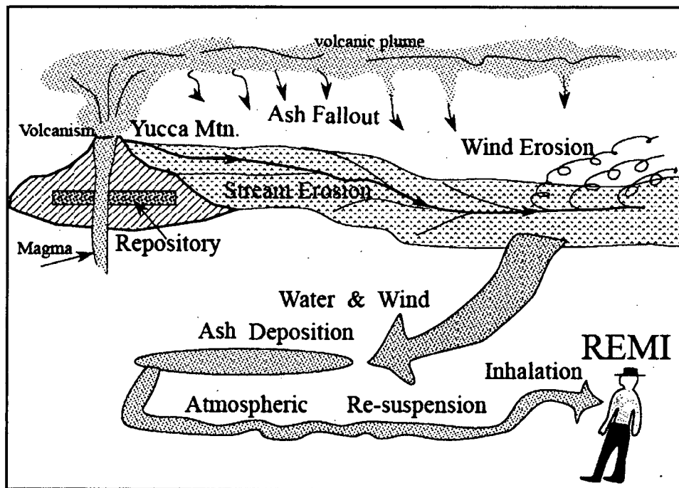
Figure 24 Schematic diagram of processes involved in ash remobilization.
