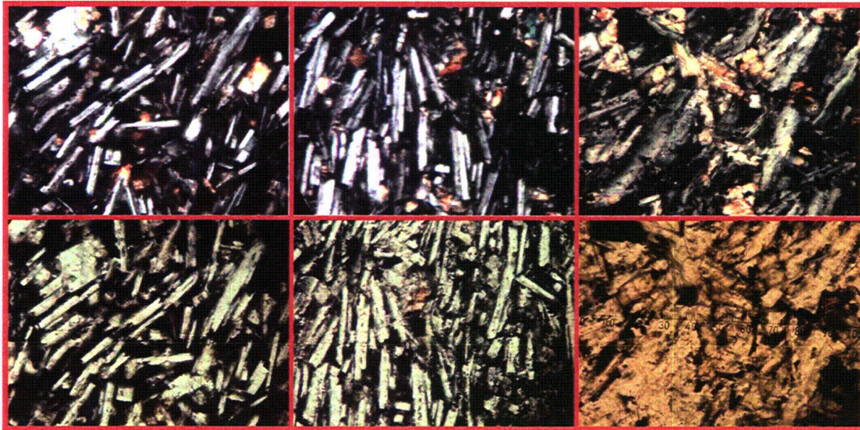
Figure 52 Photomicrographs of thin sections of samples of lava from Lathrop Wells. The field of view in each view is ~1 mm, and the upper row is under crossed Nicols and polarized light and the bottom row are the same sections in uncrossed Nicols. The white laths are plagioclase and the brown interstitial material is glass. The left pair of thin sections is nearest the vent and the others to the right are at successively greater distances from the vent, approximately evenly spaced out to a distance of approximately 1 km. The degree of crystallinity increases from left to right from about 40 vol.% to over 70 vol.% and the crystals coarsen in size, which reflects the overall cooling of the flow with distance from the vent. As the effective viscosity becomes very large, the flow moves more as a debris flow than as a viscous fluid.
