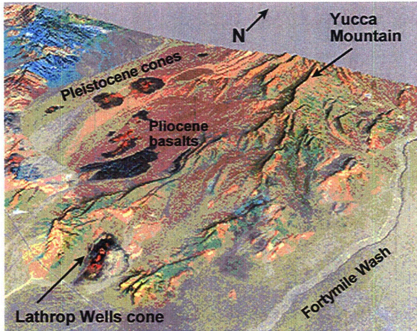
Figure 26 Pleistocene and Pliocene volcanoes in Crater Flat. The 80,000-yr-old Lathrop wells cone is the youngest volcano in this area. Diagram courtesy of Dennis W. O’Leary, U.S. Geological Survey.
