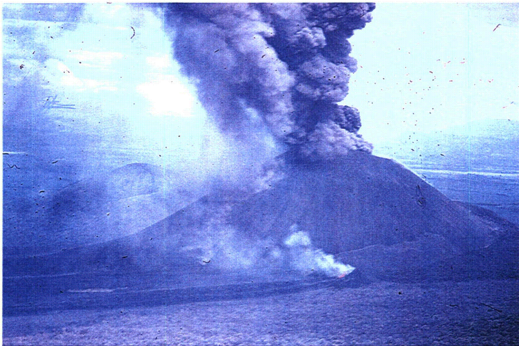
Figure 28 The 1968 Strombolian eruption of Cerro Negro Volcano, Nicaragua. In the foreground is a small crater that is emitting fire fountains of magma that are feeding a lava flow during the central crater's Strombolian eruption. Diameter of the base of the volcano is about 1.5 km (After Melson (2002) from a photo by Robert Citron).
