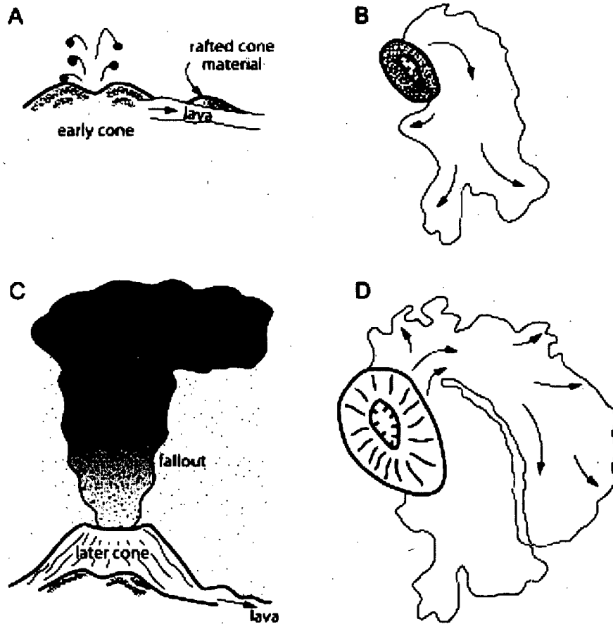
Figure 2: Schematic of (A-D) four possible eruptive events for the main cone at Lathrop Wells basalt center (Valentine et al., 2005).
