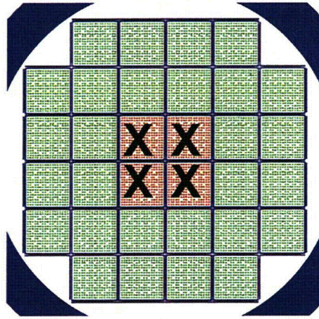
4 misloaded assemblies
