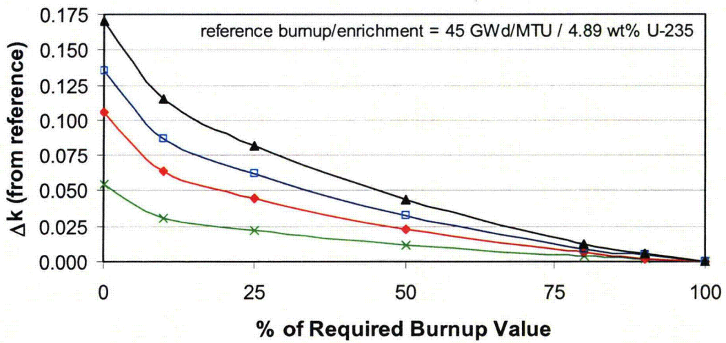
Figure 8. \Delta k effect as a function of the percentage of required burnup for cases involving 1–4 misloaded assemblies, using the Set 2 nuclides.
