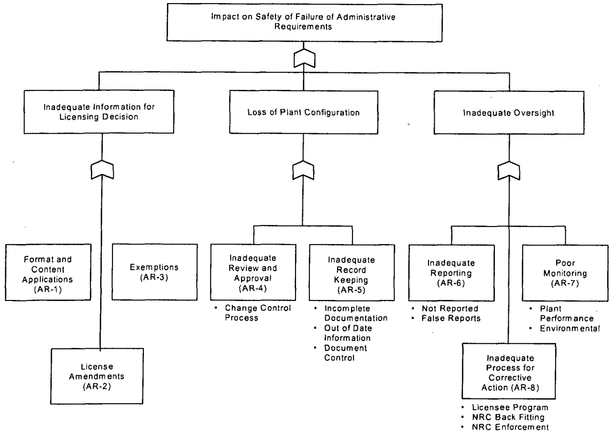
Figure G-6 Logic tree for the administrative area.
