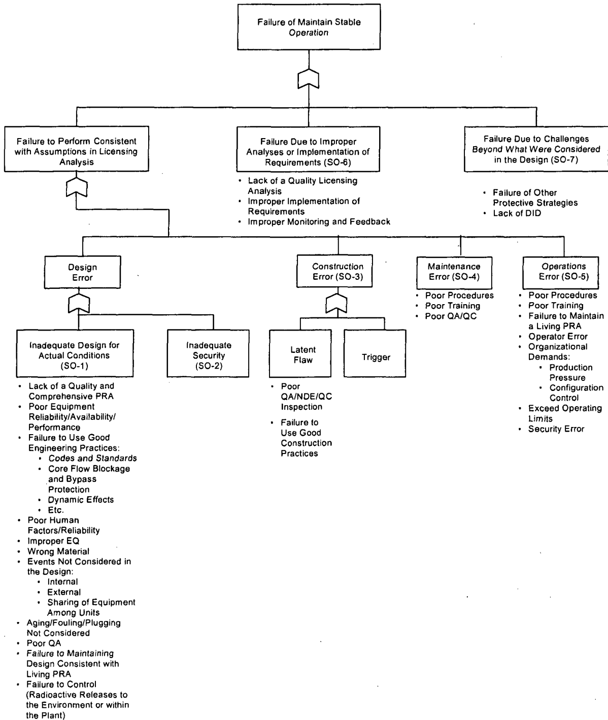
Figure G-2 Logic tree for the stable operation strategy.
