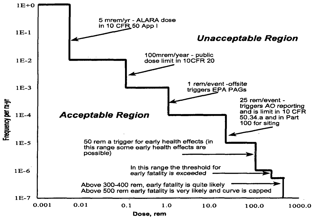
Figure J-1 Dose (rem) at the EAB and at the Outer Edge of the LPZ (EAB per year for event scenario frequencies greater than 10^{-3}/\text{yr} and for the worst 2 hours for event scenario frequencies less than 10^{-3}/\text{yr} and for the LPZ, the duration of the event scenario).
