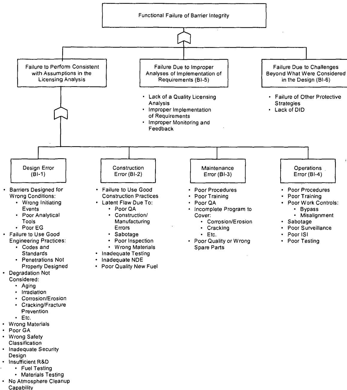
Figure G-4 Logic tree for the barrier integrity strategy.
