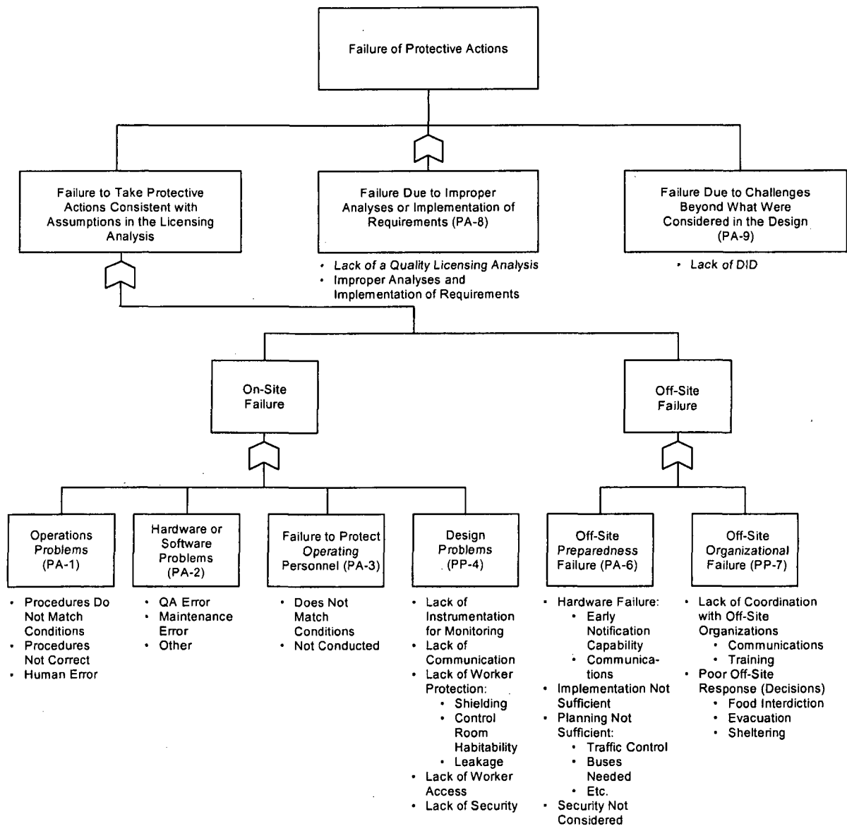
Figure G-5 Logic tree for the protective actions strategy.
