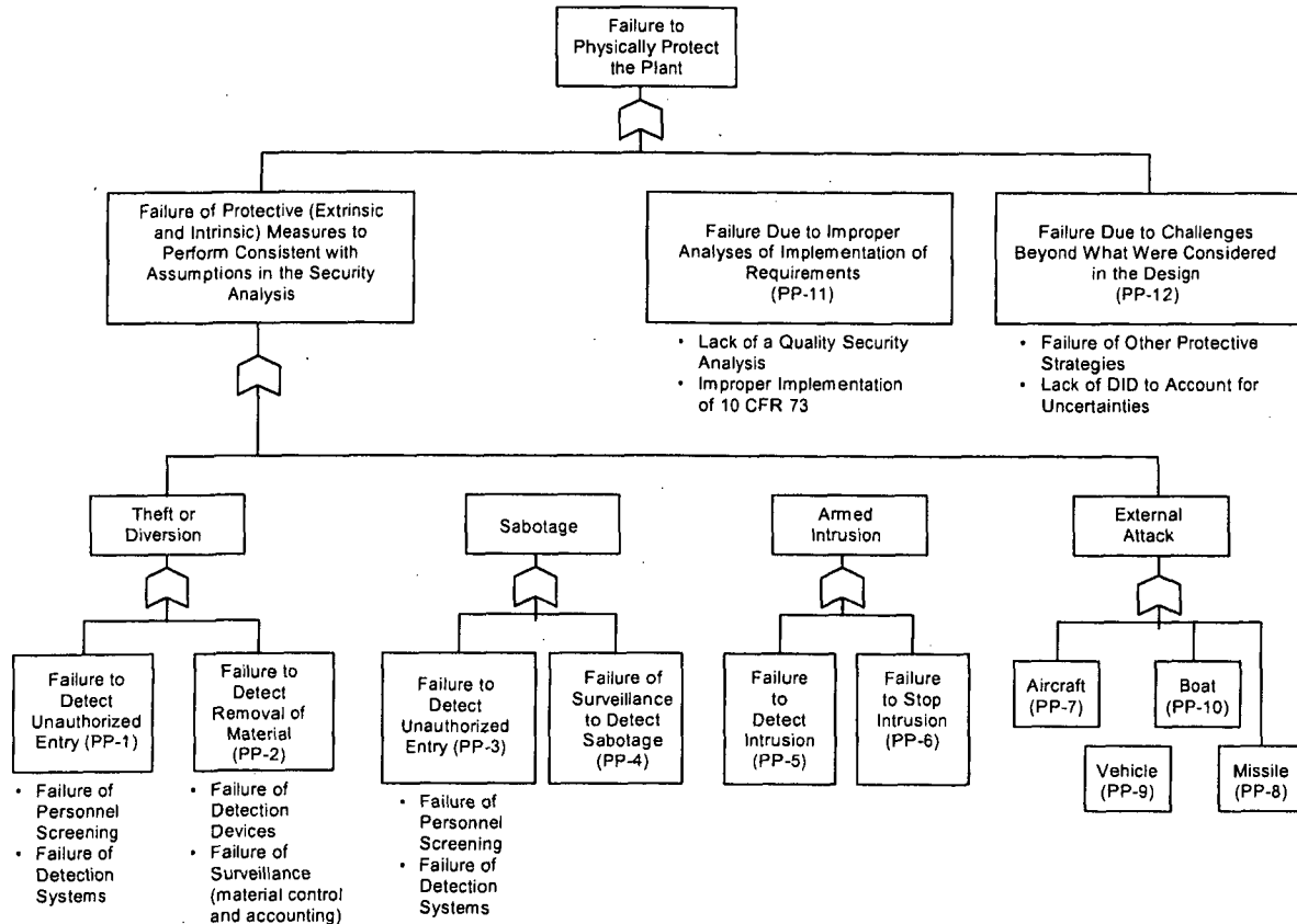
Figure G-1 Logic tree for the physical protection strategy.
