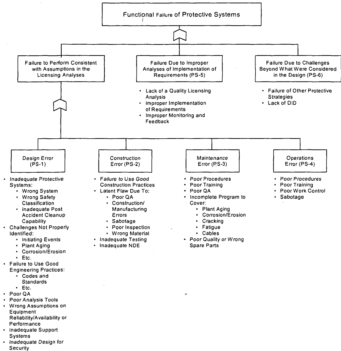
Figure G-3 Logic tree for the protective systems strategy.
