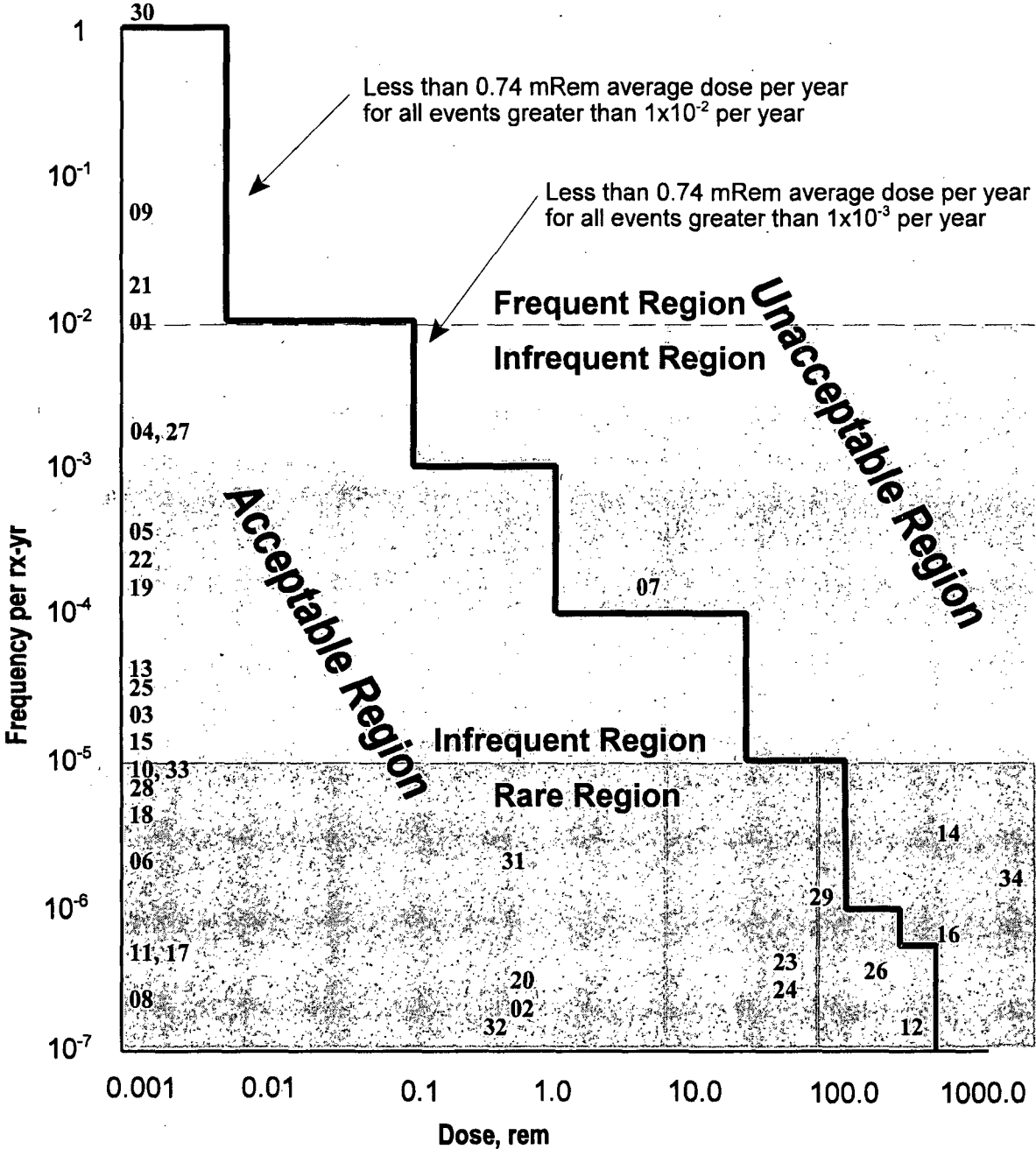
Figure E-2 Frequency-consequence curve with mean values
