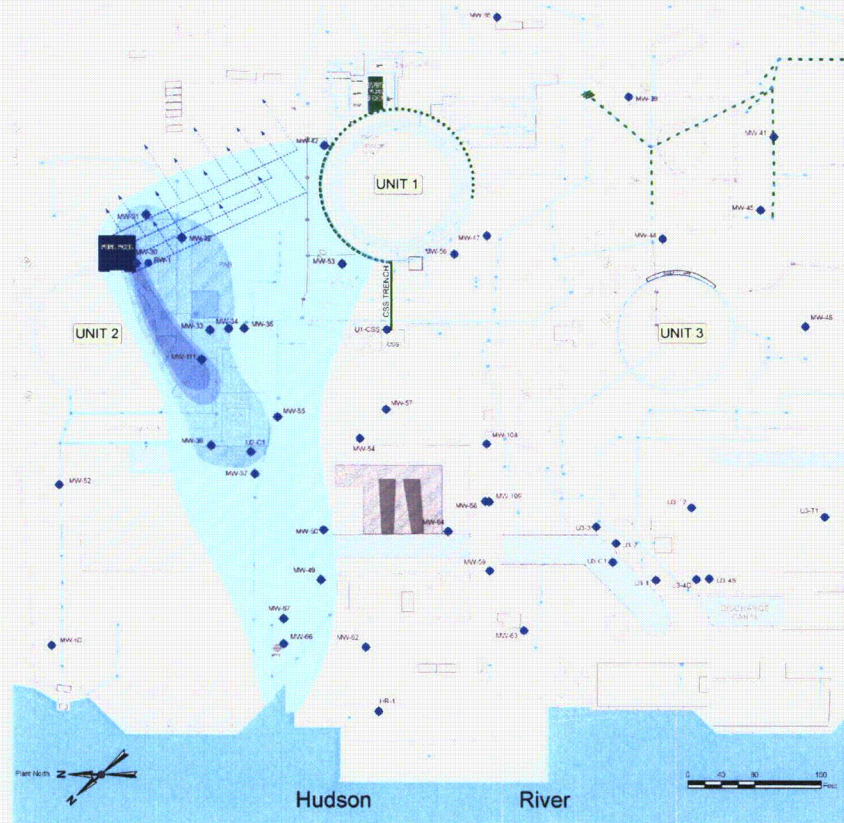
CURRENT UNIT 2 PLUME
