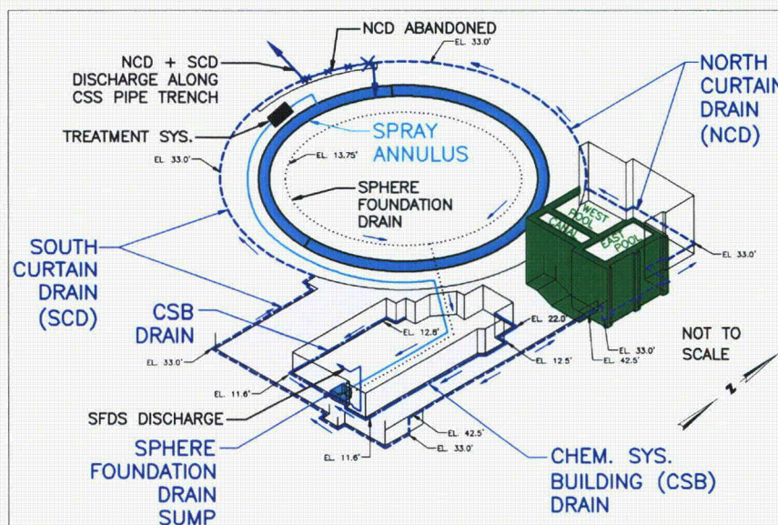
UNIT 1 FOOTING DRAINS AND DISCHARGE SUMP
