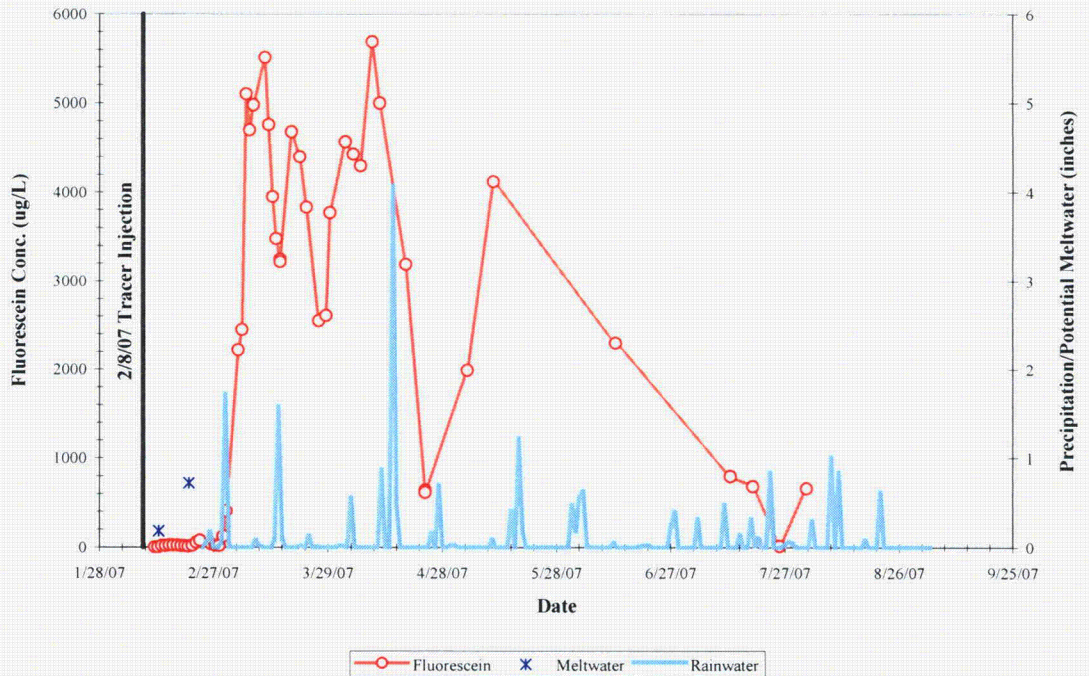
MW-30-69 FLOURESCEIN AND PRECIPITATION VS TIME
