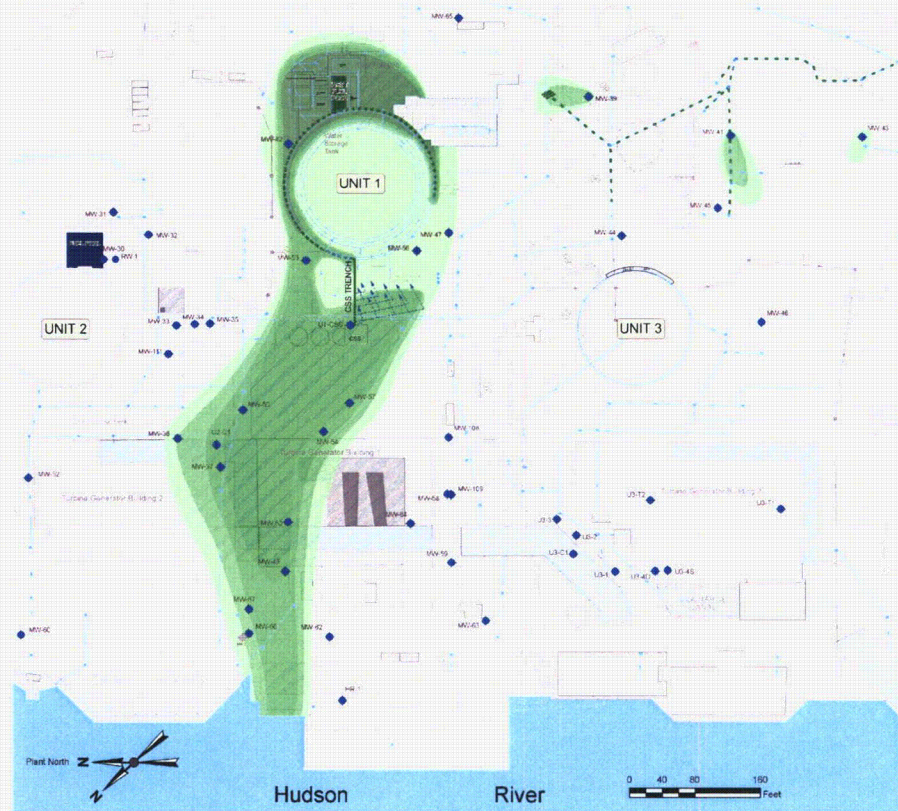
UNIT 1 BOUNDING ACTIVITY ISOPLETHS
