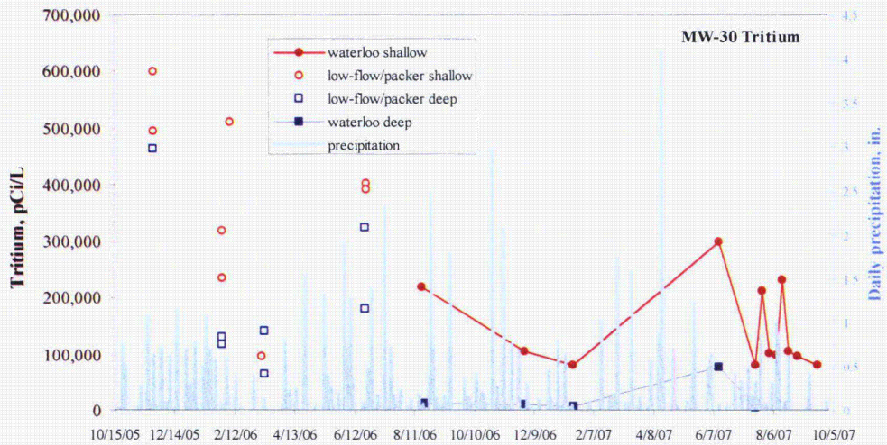
TRITIUM CONCENTRATIONS AND PRECIPITATION VS TIME FOR MW-30
