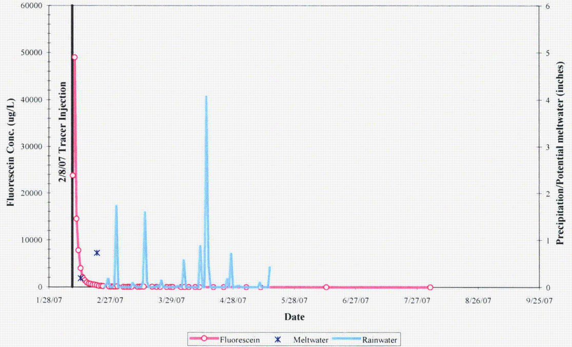
MW-32-62 FLOURESCEIN AND PRECIPITATION VS TIME
