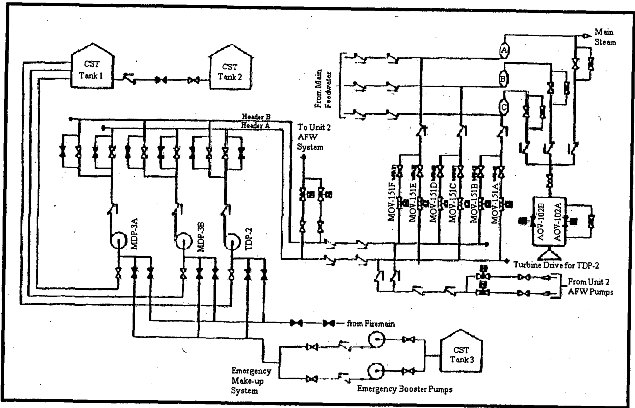
Figure 5.2.4 P&ID for Example Plant Simplified AFW System
