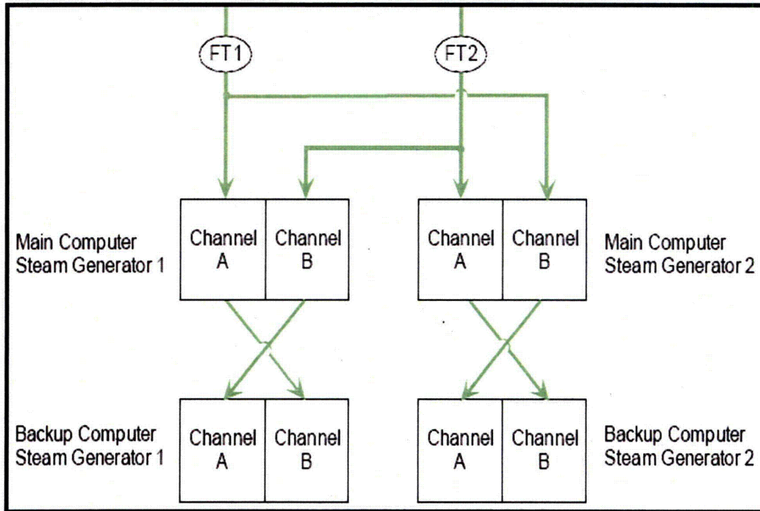
Figure 2.2.1 Feedwater Temperature Sensor Signals
