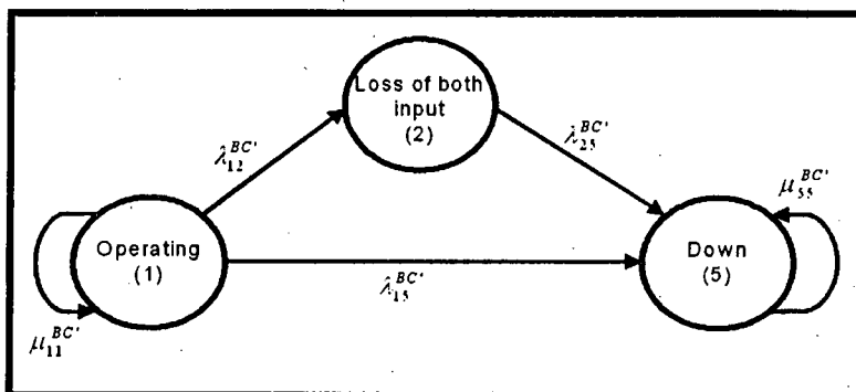
Figure 4.2.6 Failure states for the Example Initiating Event of the BC
