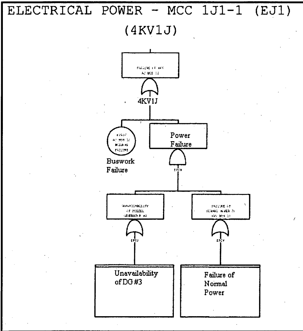
Figure 5.2.20 4KV1J - Failure of 4KV AC Bus 1J
