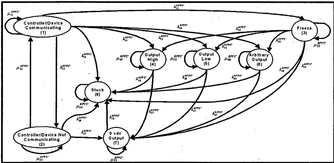
Figure 4.2.10 Failure States for the Combined BFV and BFV Controller
