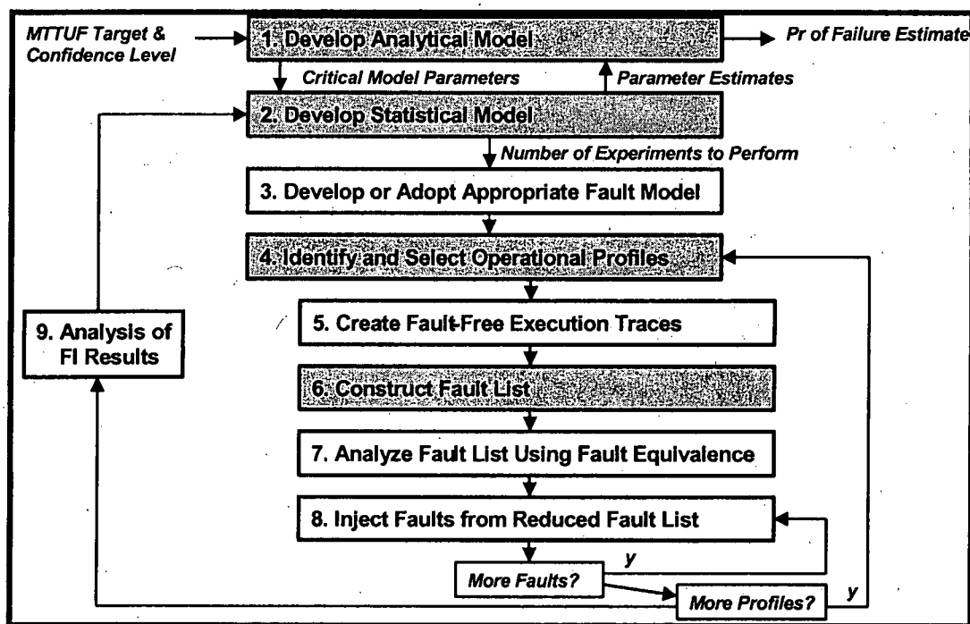
Figure 2.4.2 Operation of the Quantitative Dependability Assessment Process
