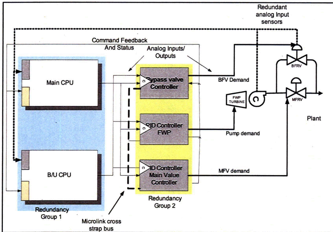
Figure 2.4.9 Architectural View of the Benchmark DFWCS.
