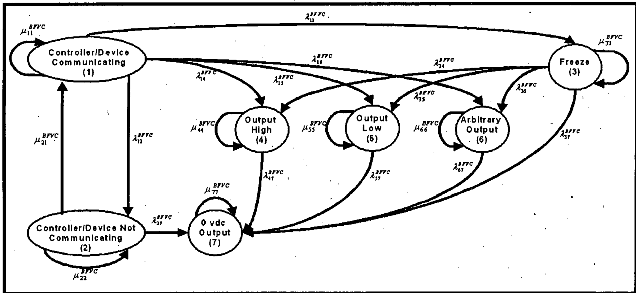
Figure 4.2.8 Failure States for the BFV Controller
