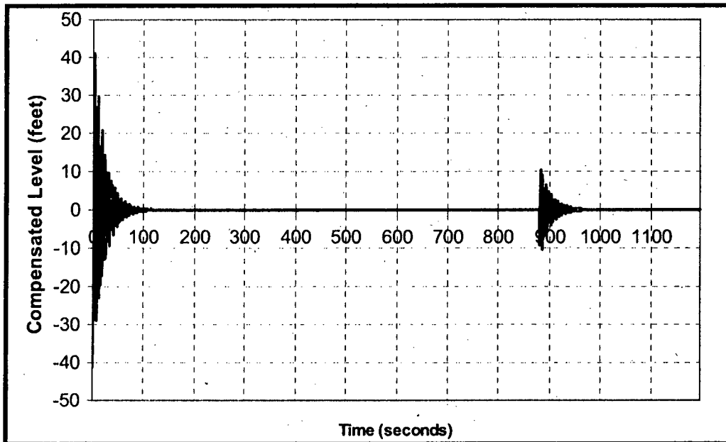
Figure 2.5.9 Variation of Compensated Level with Time with Artifact
