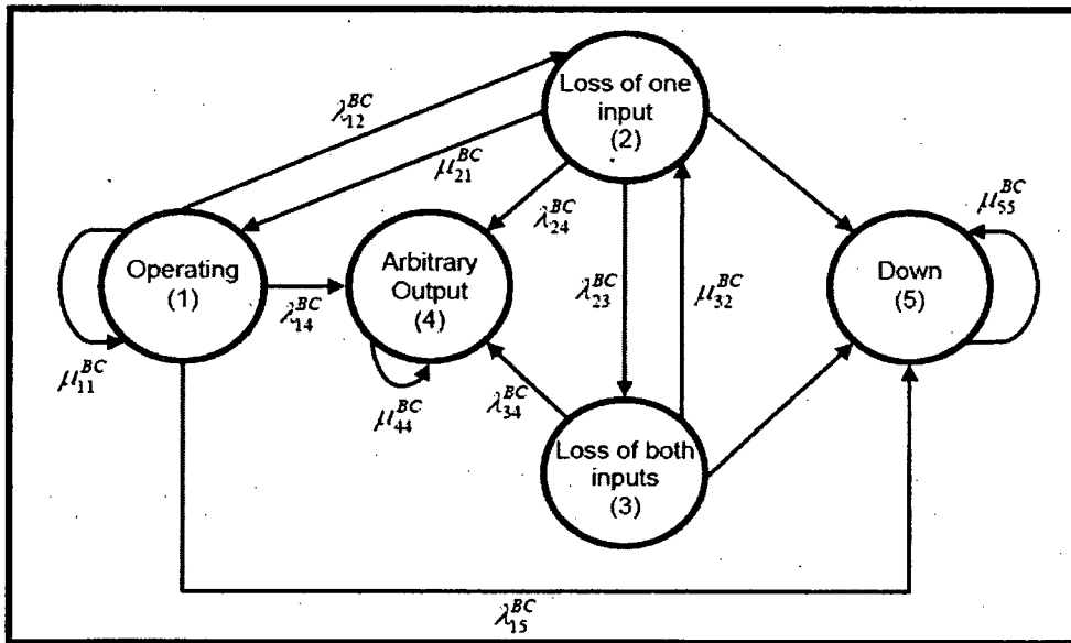
Figure 4.2.5 Failure States for the Backup Computer
