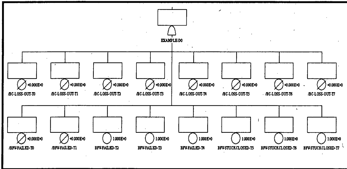
Figure 6.2.1 A Sample Fault Tree Imported into SAPHIRE
