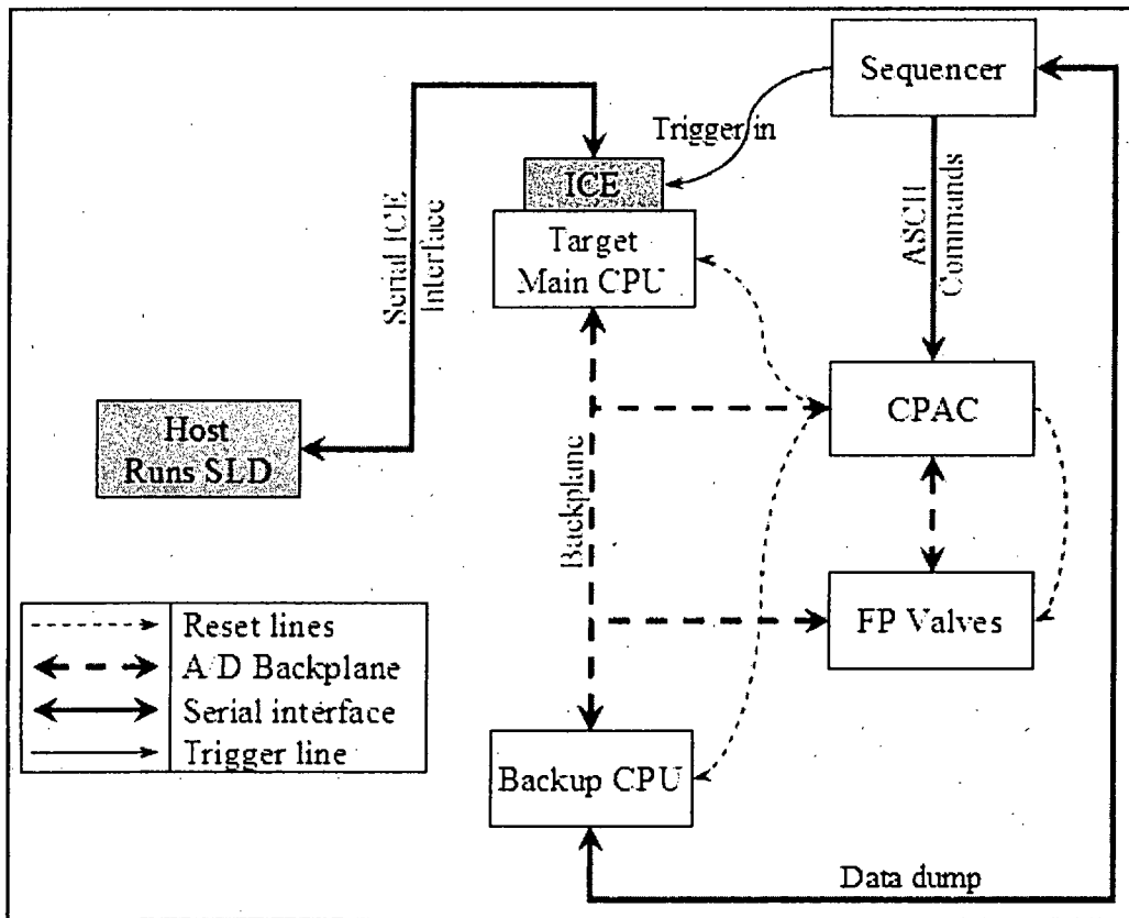
Figure 2.4.10 Integration of the In-circuit Emulator into DFWCS Lab
