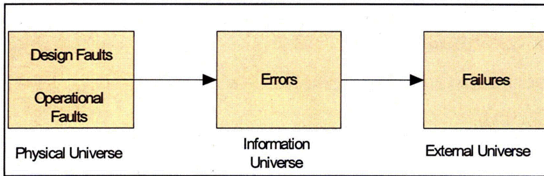
Figure 2.4.1 Cause-Effect Relationship Among Faults, Errors, and Failures using the 3- Universe Model
