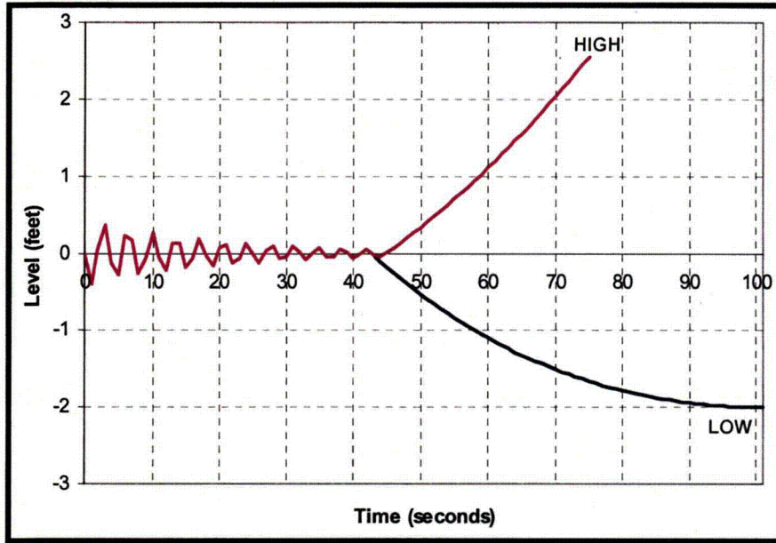
Figure 2.5.7 Different Failure Modes as Result of Timing of BFV Failure
