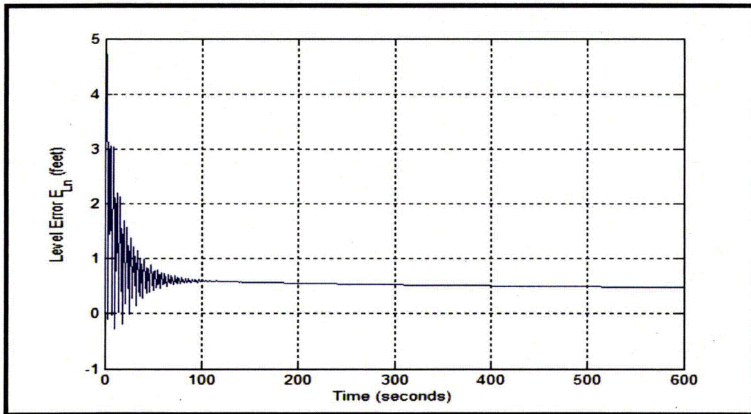
Figure 2.5.6 Variation of Level Error with Time For the Example Initiating Event
