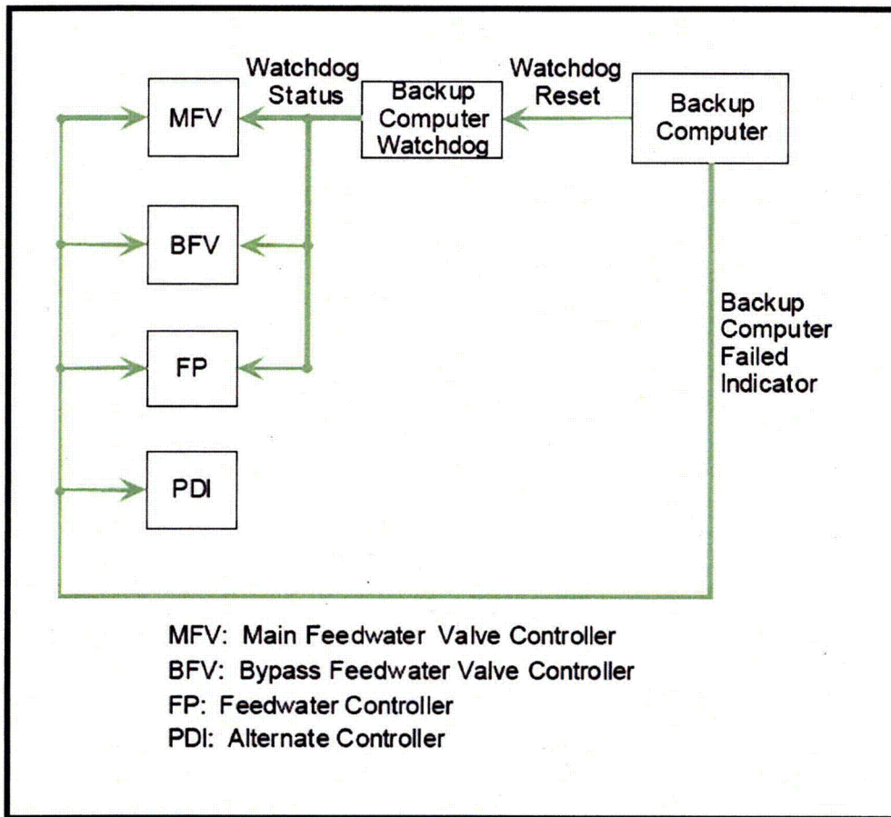
Figure 2.2.7 Digital Feedwater Controller Status Interconnection for BC
