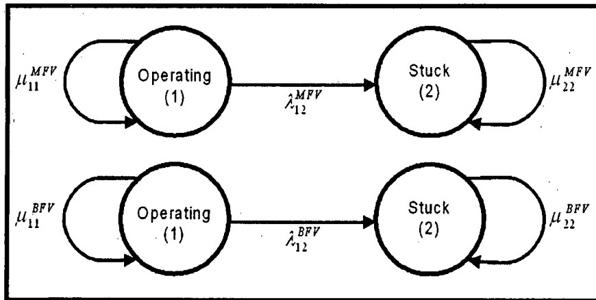
Figure 4.2.2 Failure States for the MFV and BFV
