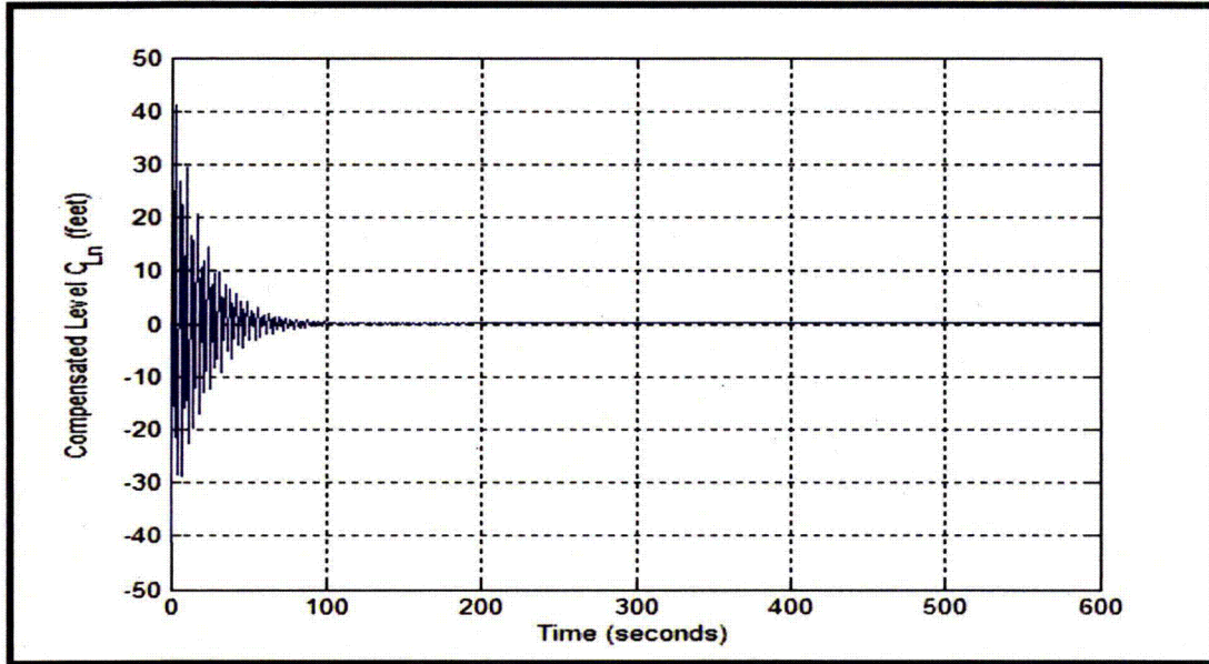
Figure 2.5.5 Variation of Compensated Level with Time for the Example Initiating Event
