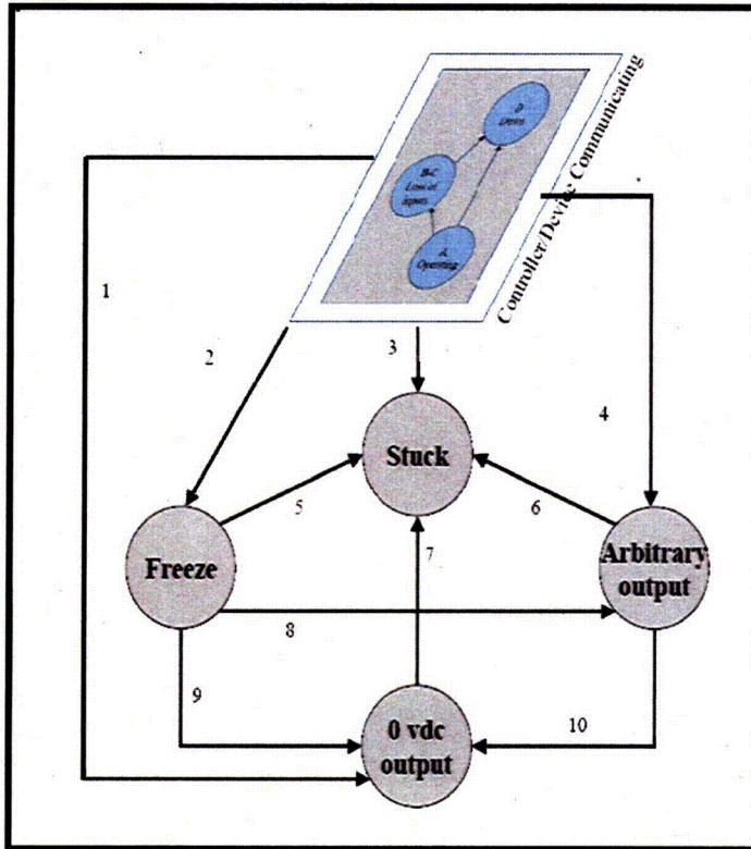
Figure 4.3.1 Markov Modeling of the Example Initiating Event
