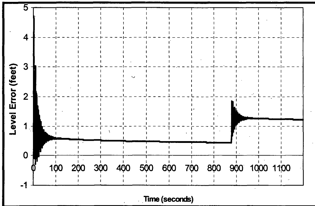
Figure 2.5.10 Variation of Level Error with Time with Artifact
