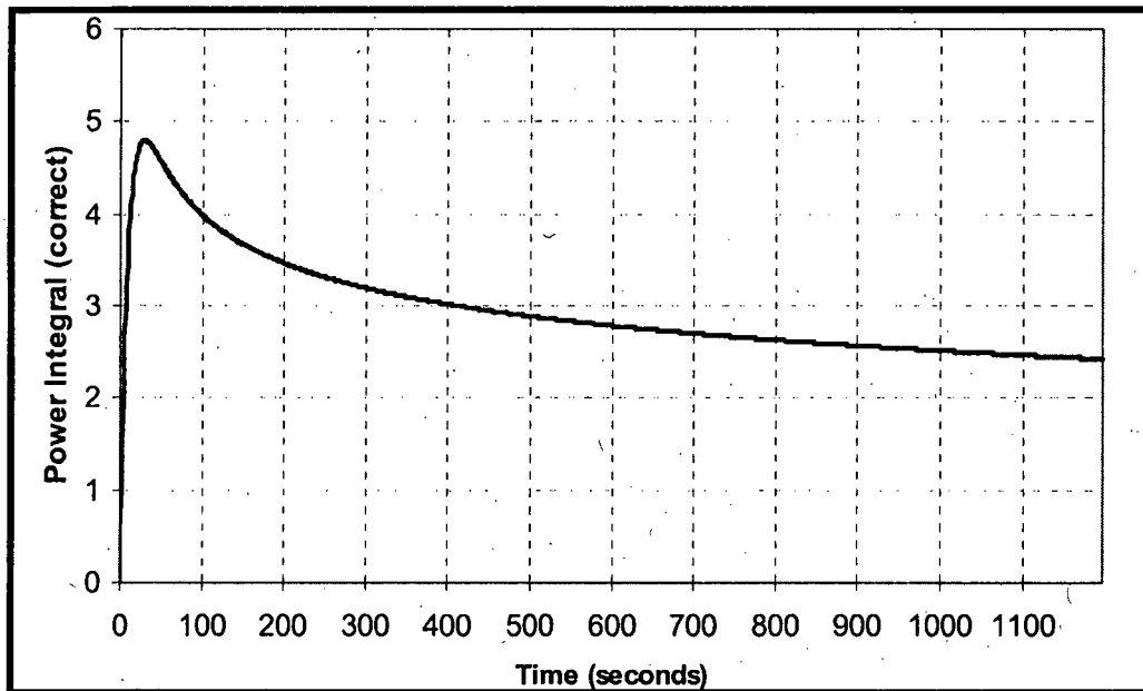
Figure 2.5.11 Correct Evaluation of the Integral in Eq. (2.5.20)
