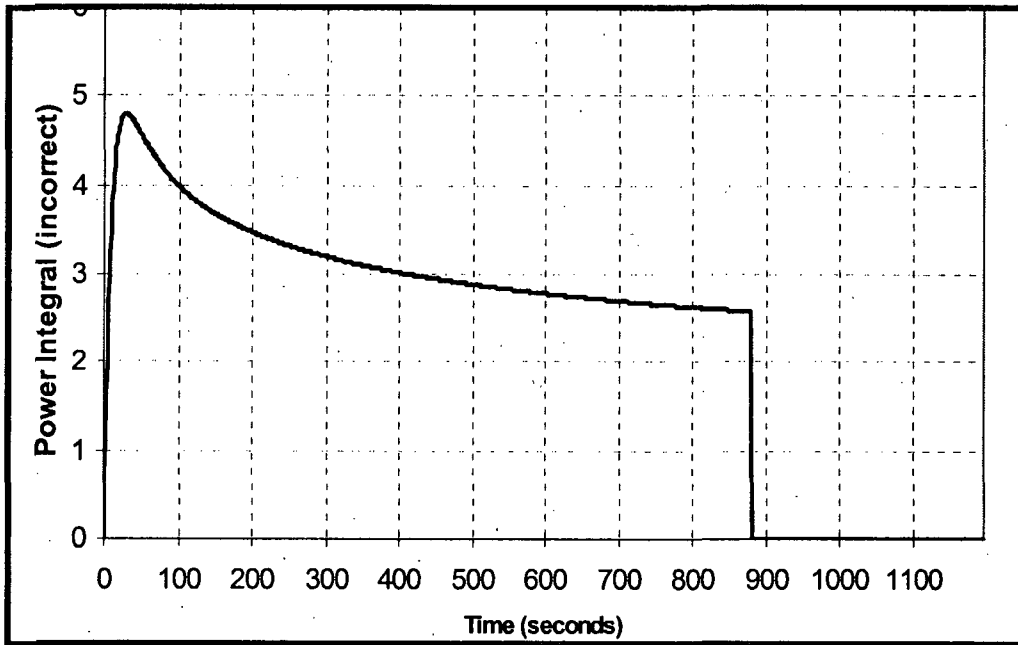
Figure 2.5.12 Incorrect Evaluation of the Integral in Eq. (2.5.20)
