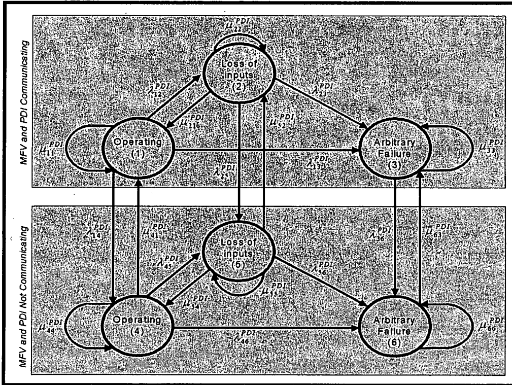
Figure 4.2.9 Failure States for the PDI Controller
