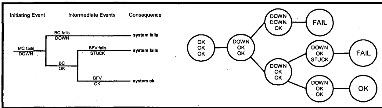
Figure 5.4.1 Event Tree vs. Tree Data Structure
