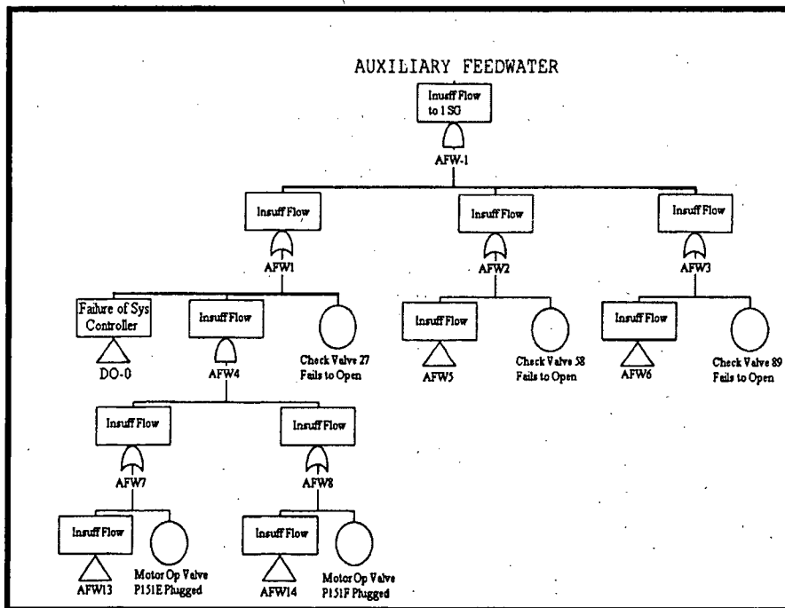
Figure 6.3.1: Appended Fault Tree to Include Imported DFWCS
