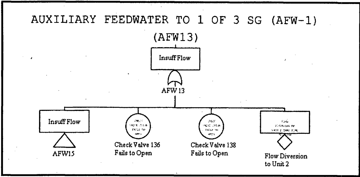
Figure 5.2.6 AFW13 - Subtree for Example Plant AFW System
