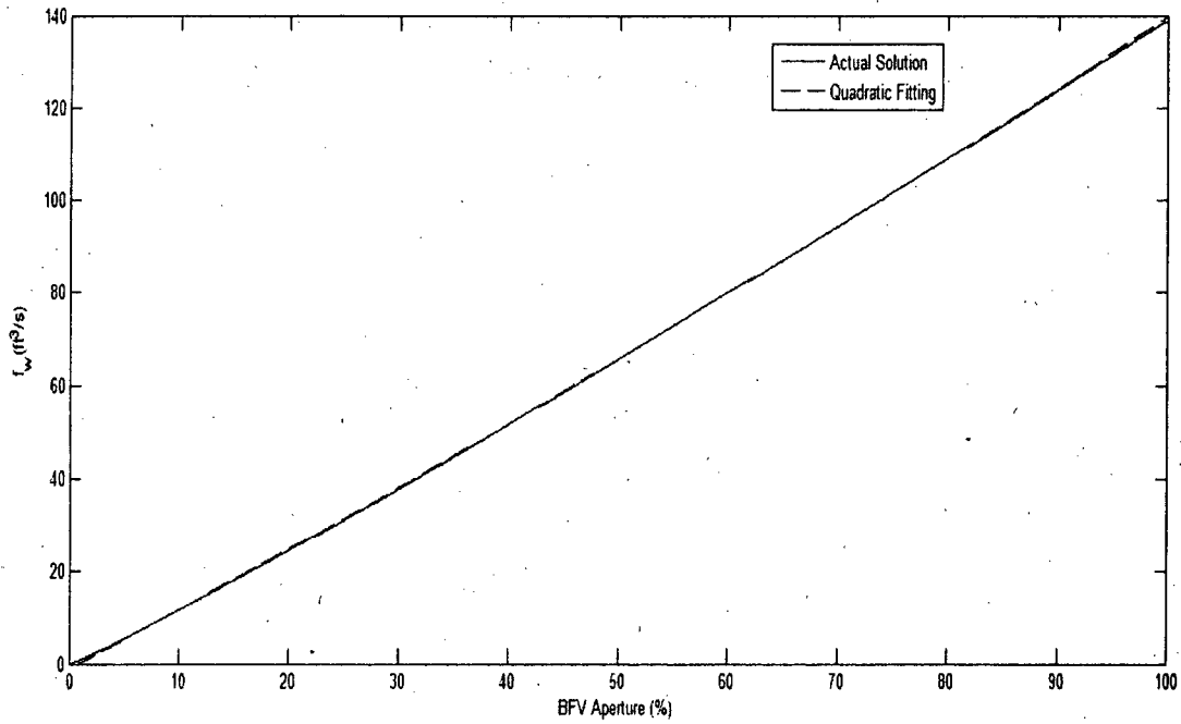
Figure 2.5.1 The Solution of f_{wn} from Eq.(2.5.15) as a Function of \tilde{S}_{Bn}
