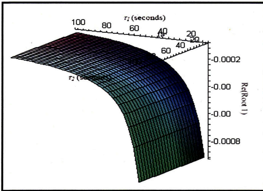
Figure 2.5.2 Real Part of Root 1 of the Transfer function of Eqs.(2.5.17), (2.5.18) and (2.5.19) Following Linearization Around E_{Ln} = 0
