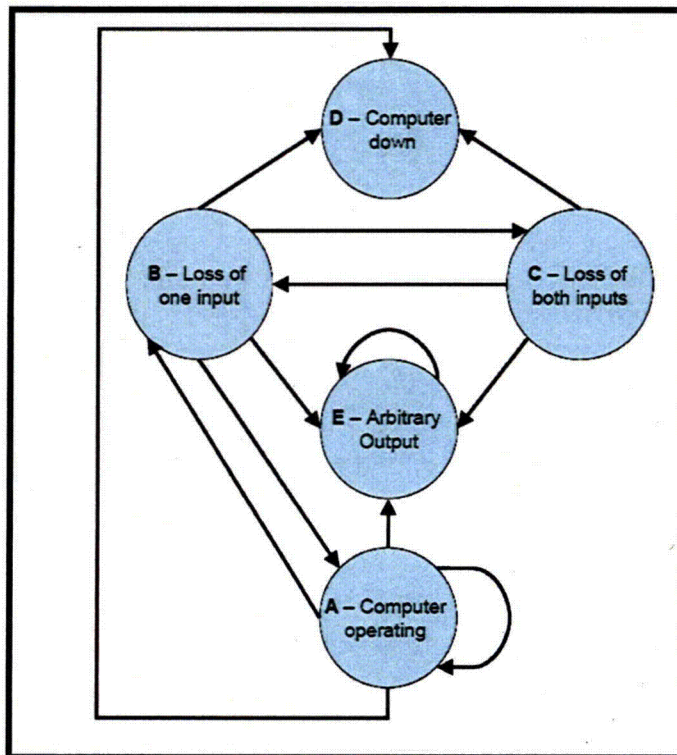
Figure 2.3.1 Intra-computer interactions of the DFWCS
