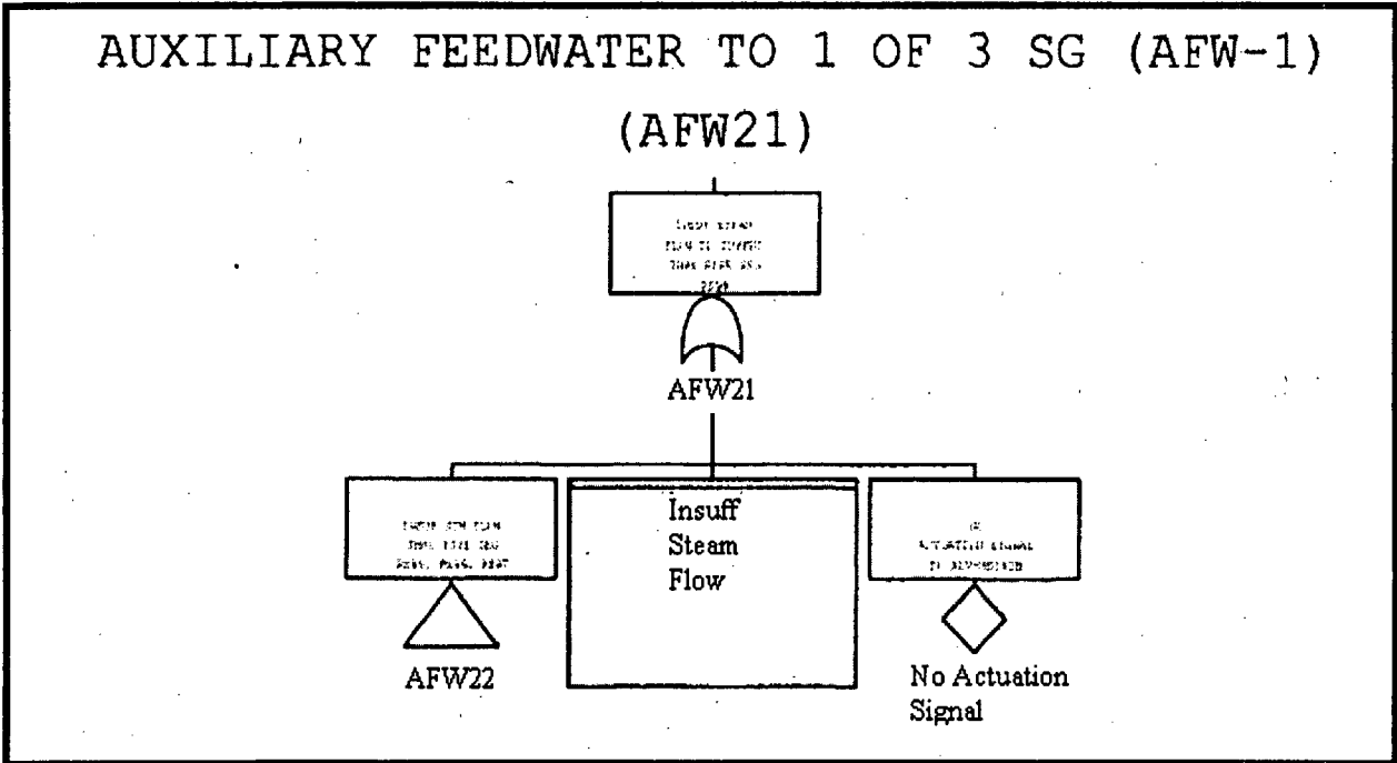
Figure 5.2.11 AFW21 - Subtree for Example Plant AFW System
