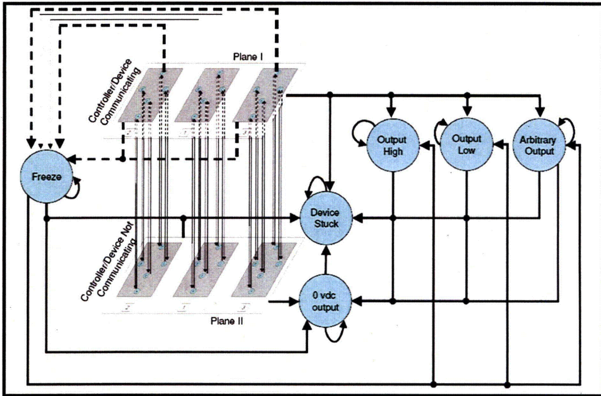
Figure 2.3.3 Computer-Controller-Actuated Device Interactions
