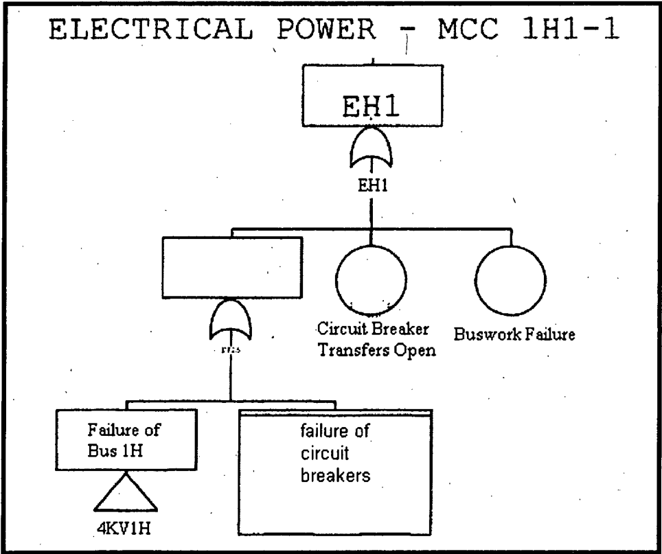
Figure 5.2.15 EH1 - Failure of 480 V AC MCC
