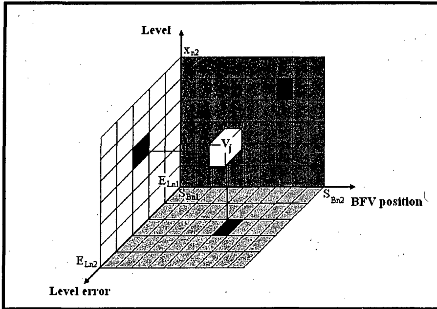
Figure 4.2.1 The CVSS for the Benchmark System based on Eqs (2.5.17) - (2.5.20)
