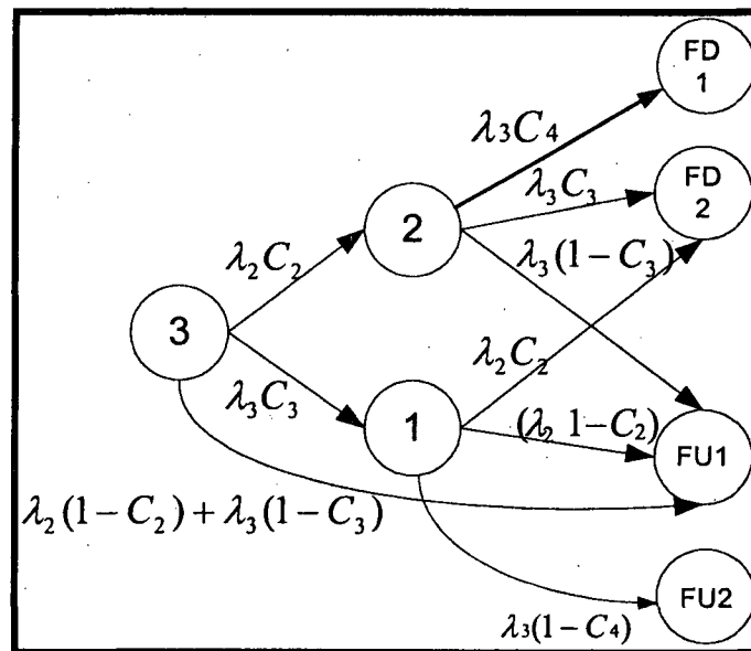
Figure 2.4.3 Markov model of main computer of the DFWCS.
