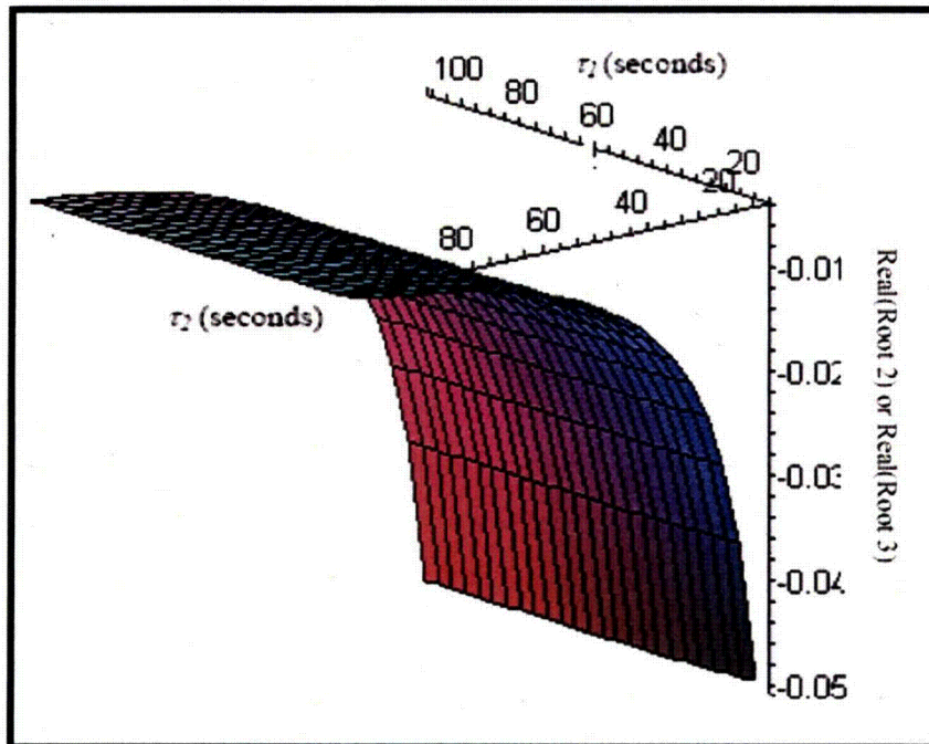
Figure 2.5.3 Real Part of Root 2 or Root 3 of the Transfer Function of Eqs.(2.15.17), (2.15.18) and (2.15.19) Following Linearization Around E_{Ln}=0
