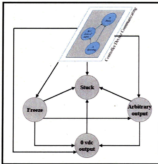
Figure 2.5.13 Example Initiating Event Transitions
