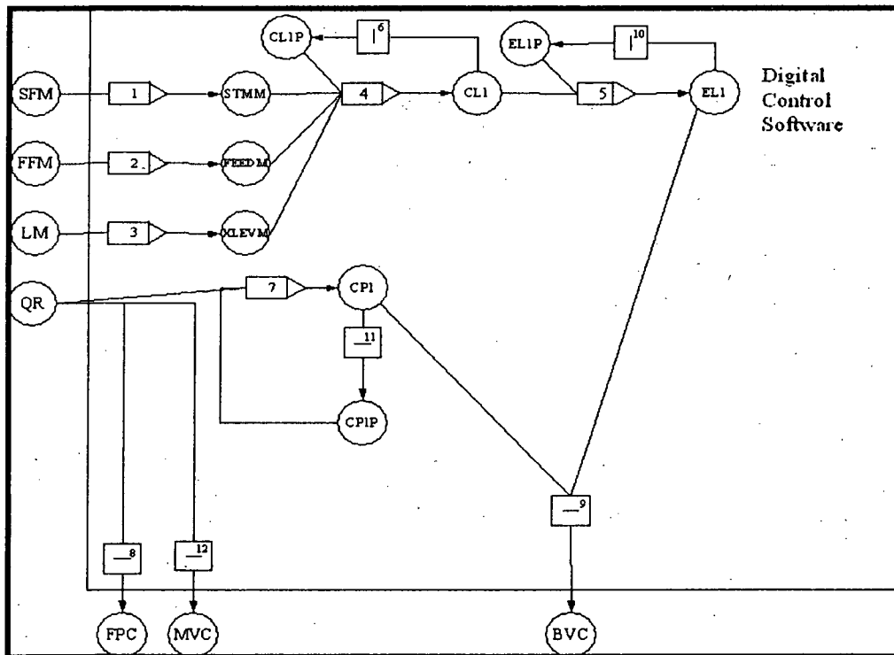
Figure 3.4.2 DFM Model of the Digital Feedwater Control System
