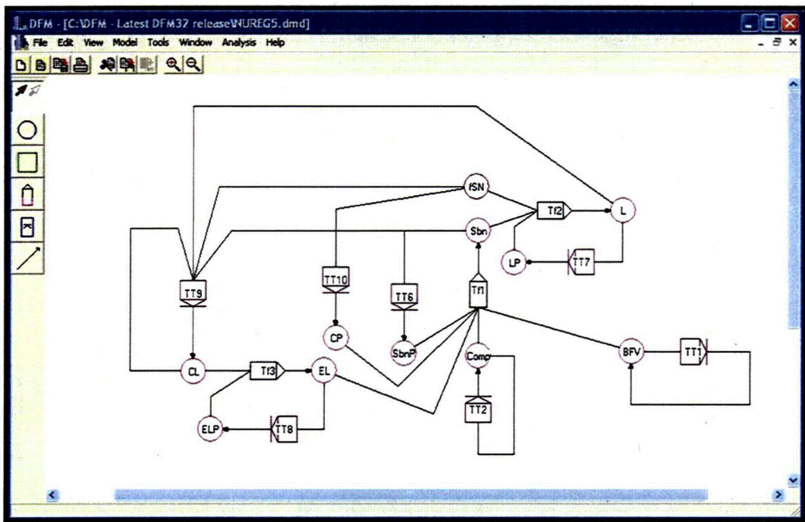
Figure 3.5.1 DFM Model for the Example Initiating Event
