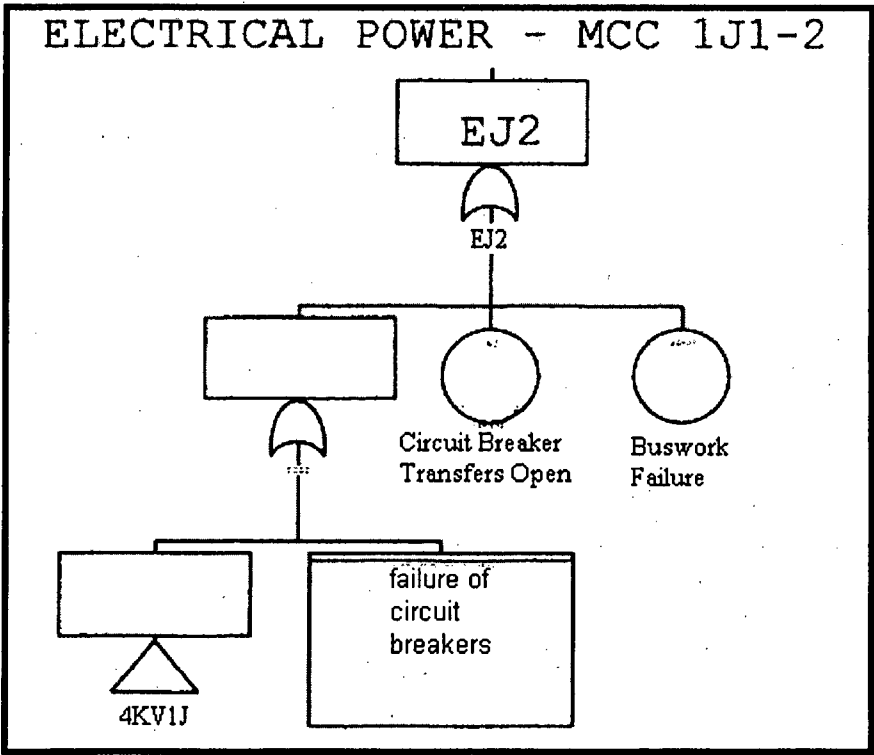
Figure 5.2.18 EJ2 - Failure of 480 V AC MCC
