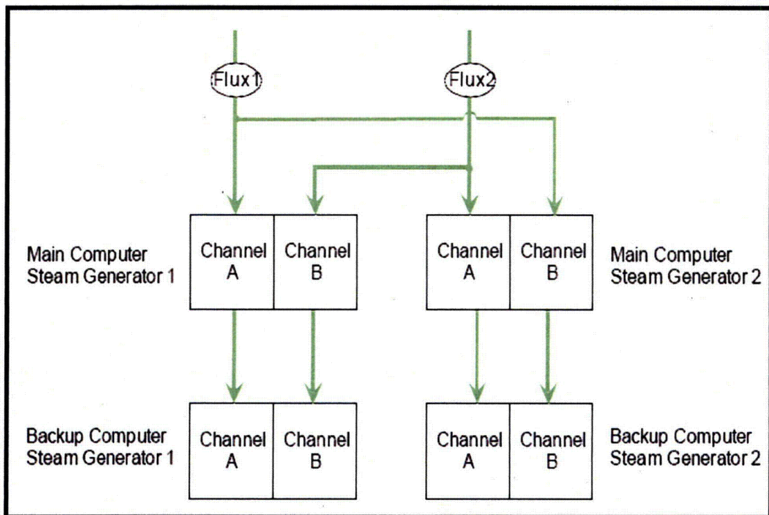
Figure 2.2.3 Neutron Flux Sensor Signals
