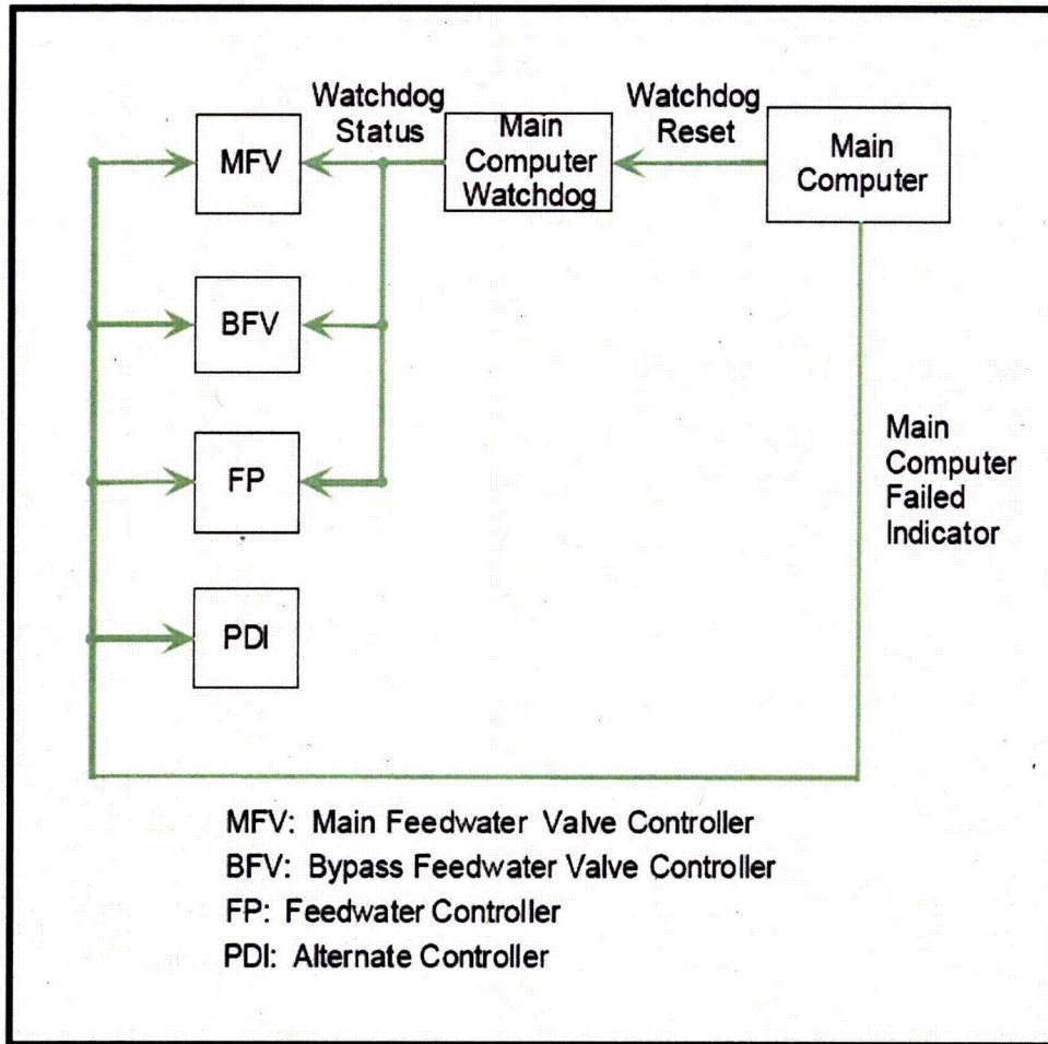
Figure 2.2.6 Digital Feedwater Controller Status Interconnections for MC
