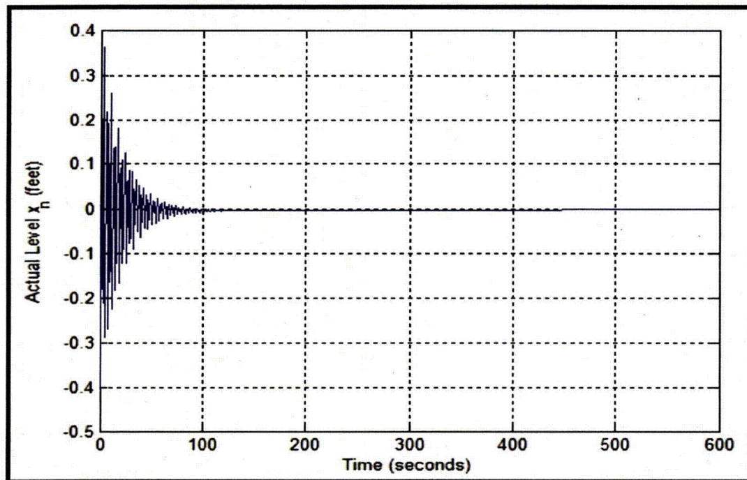
Figure 2.5.4 Variation of Actual level with Time for the Example Initiating Event
