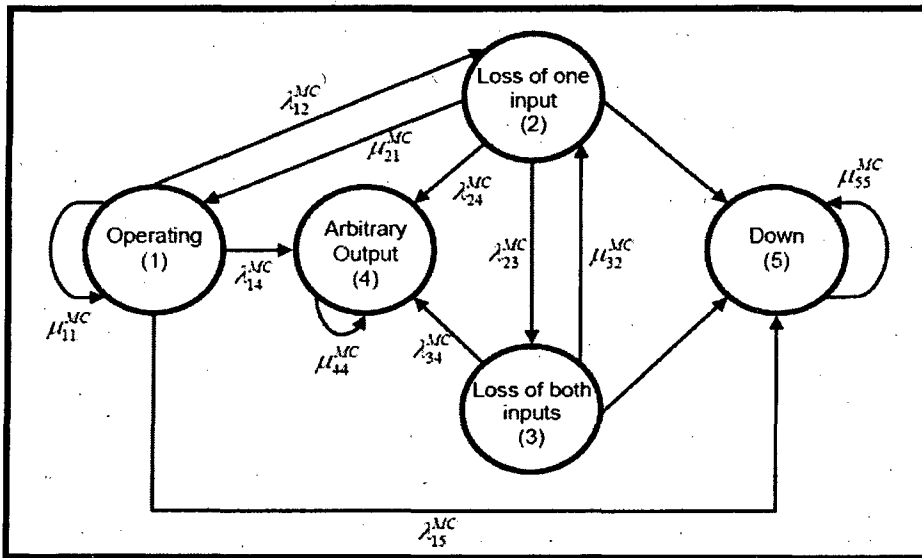
Figure 4.2.4 Failure States for the Main Computer (MC)
