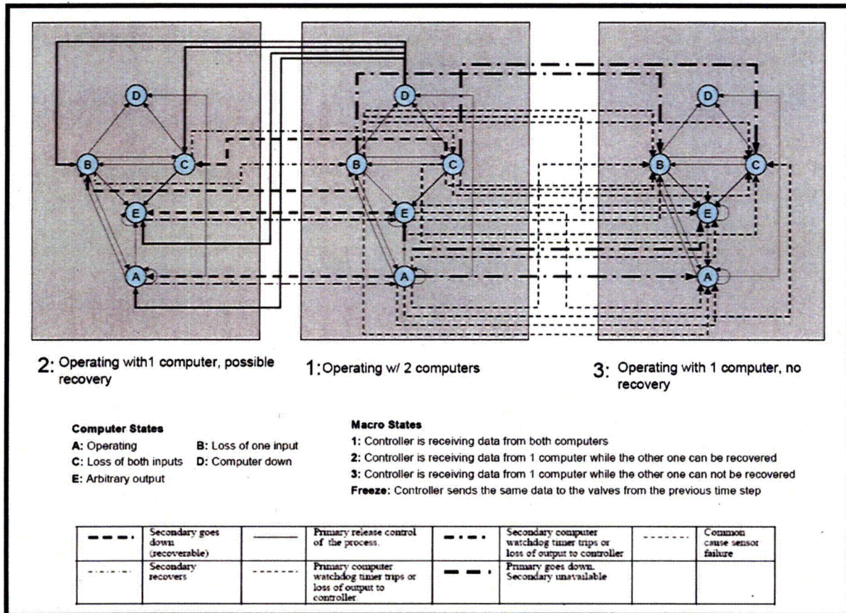
Figure 2.3.2 Inter-computer interactions of the DFWCS and definition of the macro-states (MSs)
