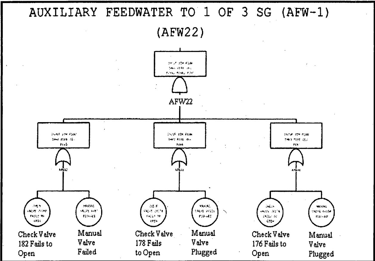
Figure 5.2.12 AFW22 - Subtree for Example Plant AFW System
