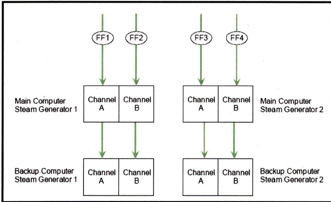
Figure 2.2.2 Feedwater Flow Sensor Signals
