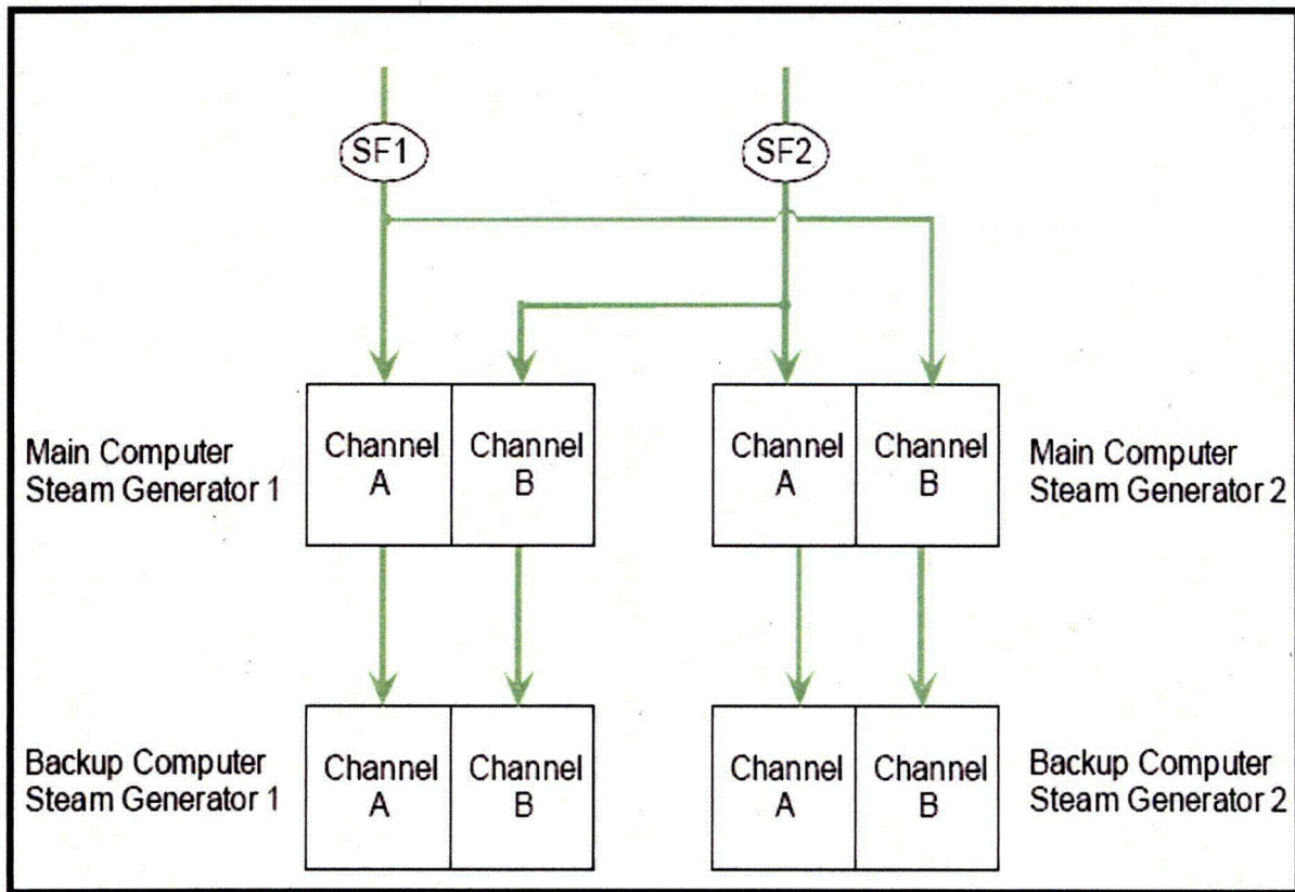
Figure 2.2.5 Steam Flow Sensor Signals
