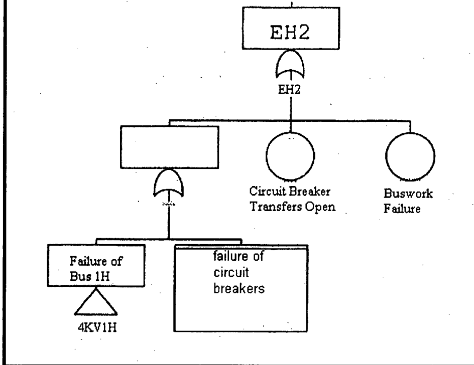
Figure 5.2.16 EH2 - Failure of 480 V AC MCC
