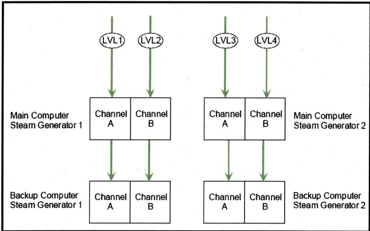
Figure 2.2.4 Feedwater Level Sensor Signals
