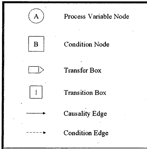
Figure 3.1.1 DFM Model Elements
