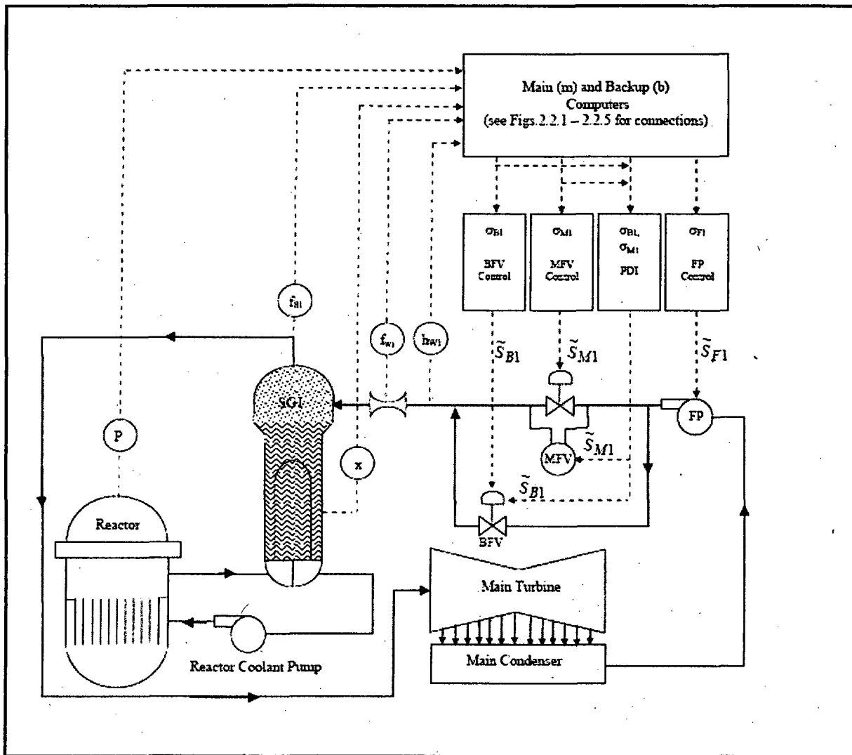
Figure 2.1.2 Detailed View of the DFWCS for SG1
