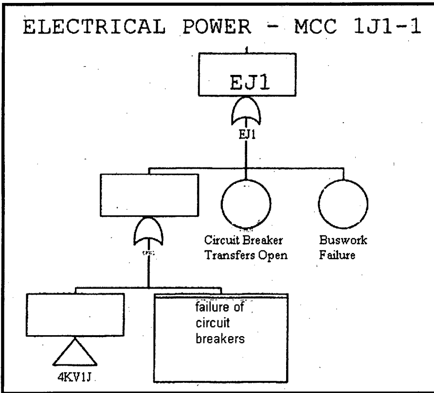
Figure 5.2.17 EJ1 - Failure of 480 V AC MCC
