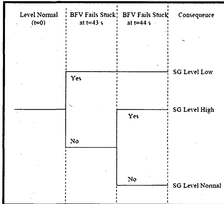
Figure 6.3.2 Incorporation of the trajectory bifurcation in Fig. 2.5.7 into a conventional PRA. Level Normal corresponds to -0.17 < x < 0.17 ft (see Fig. 4.3.1)
