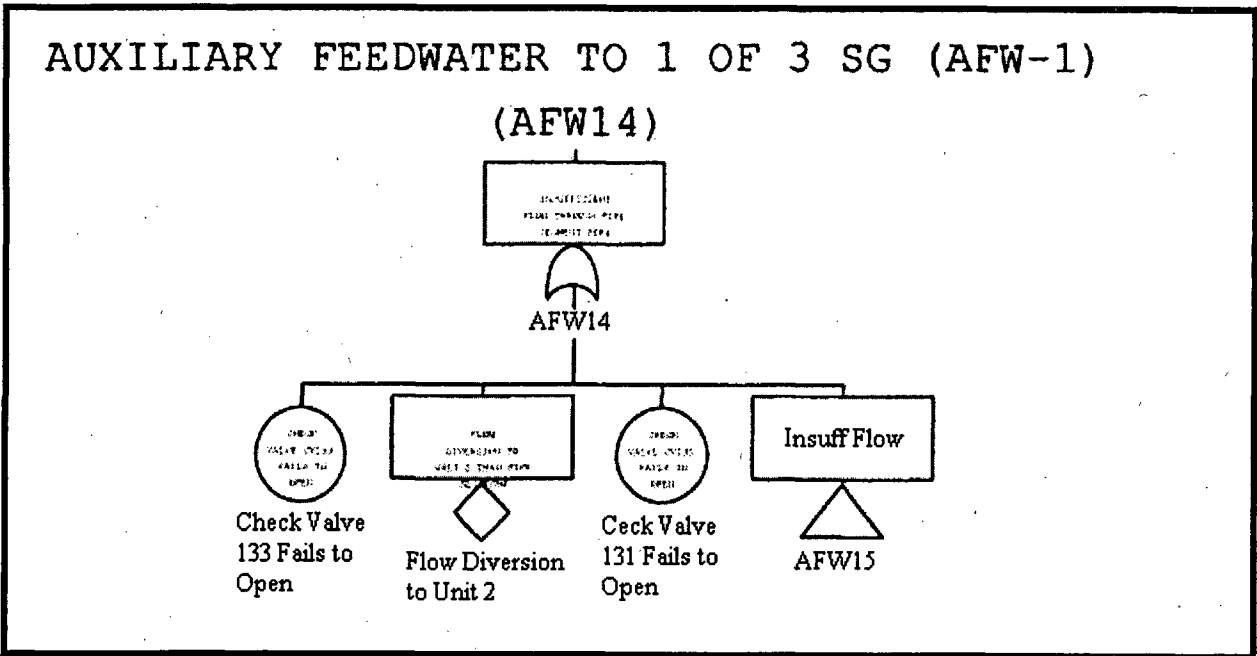
Figure 5.2.7 AFW14 - Subtree for Example Plant AFW System
