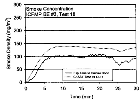
Figure A-27. Smoke Concentration, ICFMP BE #3, Open-Door Tests
