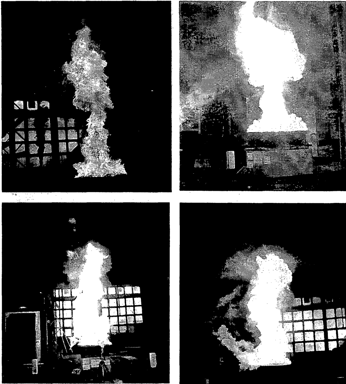
Figure A-22. Photographs of Heptane Pan Fires, ICFMP BE #2, Case 2 (Courtesy, Simo Hostikka, VTT Building and Transport, Espoo, Finland)
