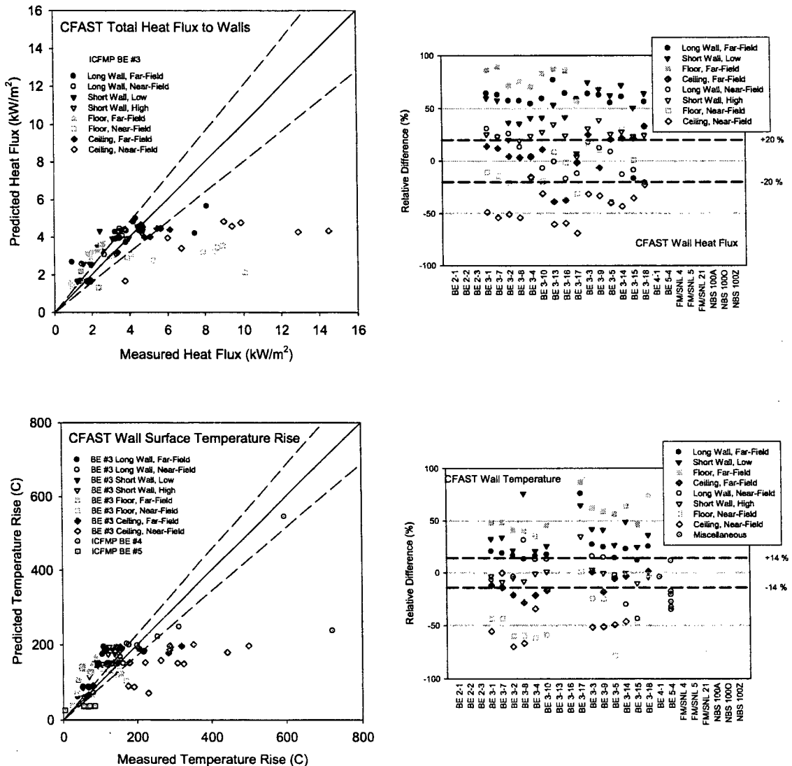
Figure 6-7. Comparisons and Relative Differences for Surface Heat Flux and Temperature
