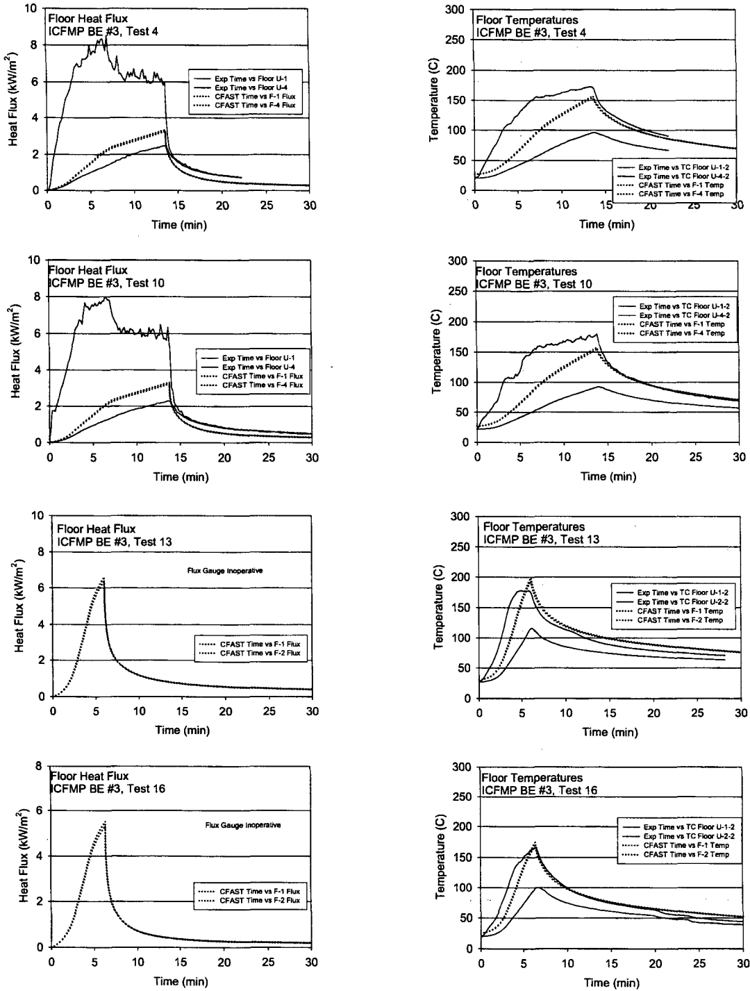
Figure A-74. Floor Heat Flux and Surface Temperature, ICMP BE #3, Closed-Door Tests
