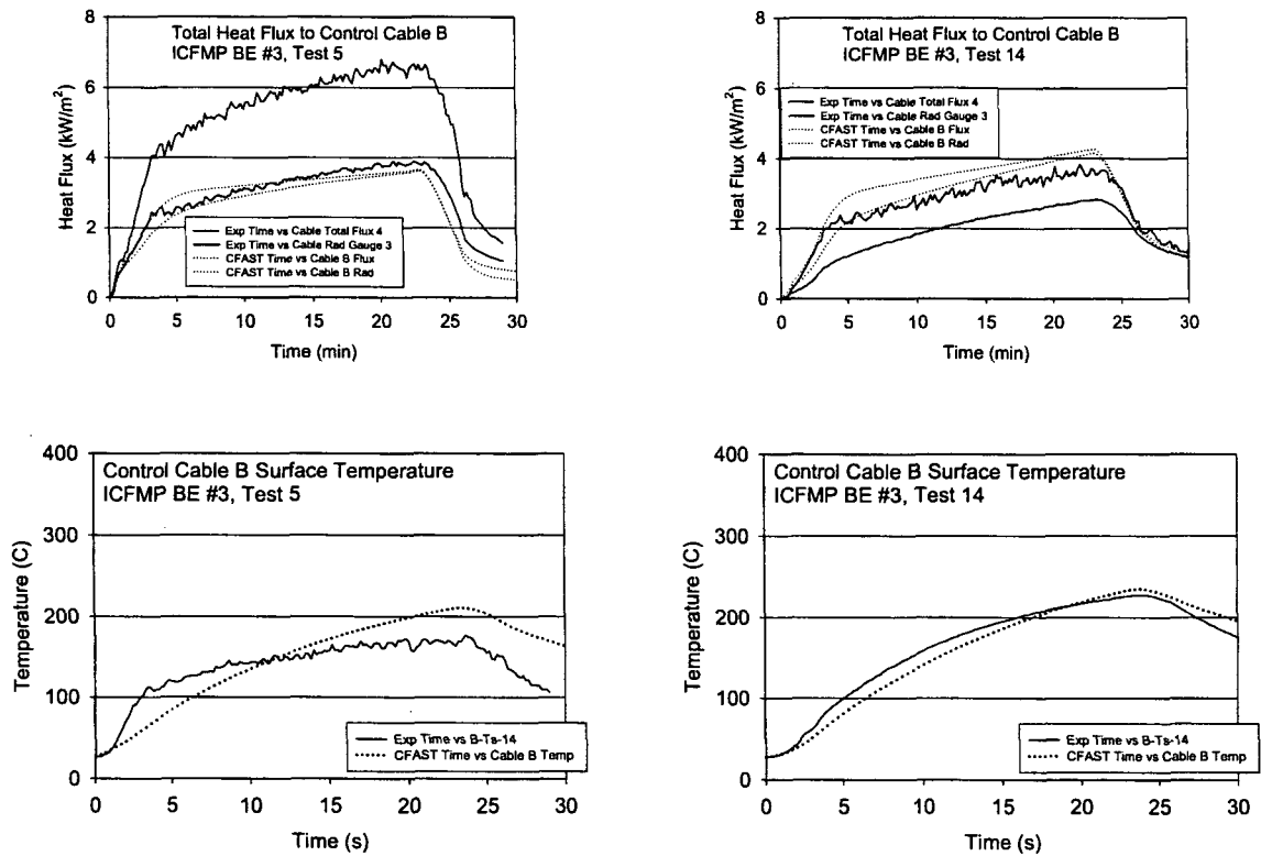
Figure A-35. Thermal Environment near Cable B, ICFMP BE #3, Tests 5 and 14
