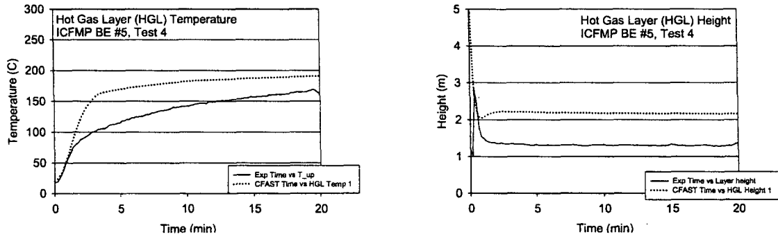
Figure A-11. Hot Gas Layer (HGL) Temperature and Height, ICFMP BE #5, Test 4
