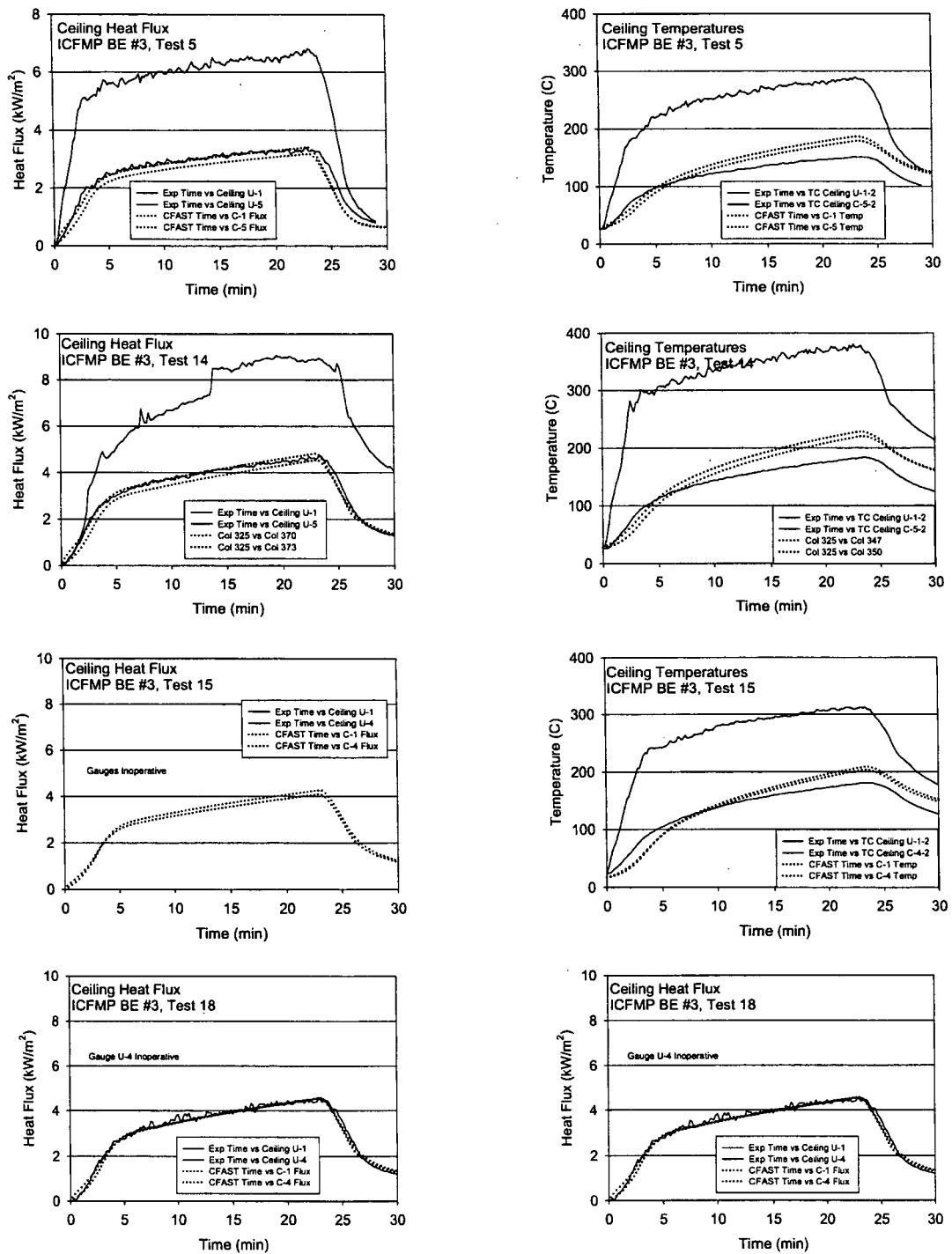
Figure A-72. Ceiling Heat Flux and Surface Temperature, ICFMP BE #3, Open-Door Tests
