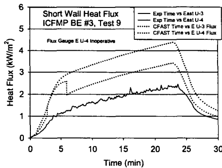
Figure A-67. Short Wall Heat Flux and Surface Temperature, ICFMP BE #3, Open-Door Tests
