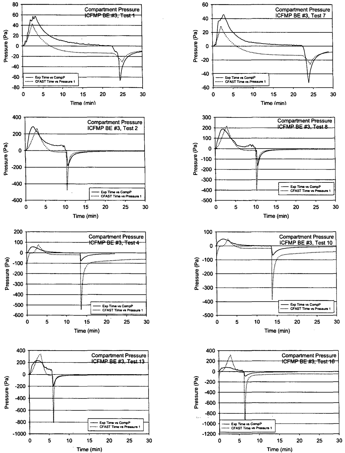
Figure A-28. Compartment Pressure, ICFMP BE #3, Closed-Door Tests
