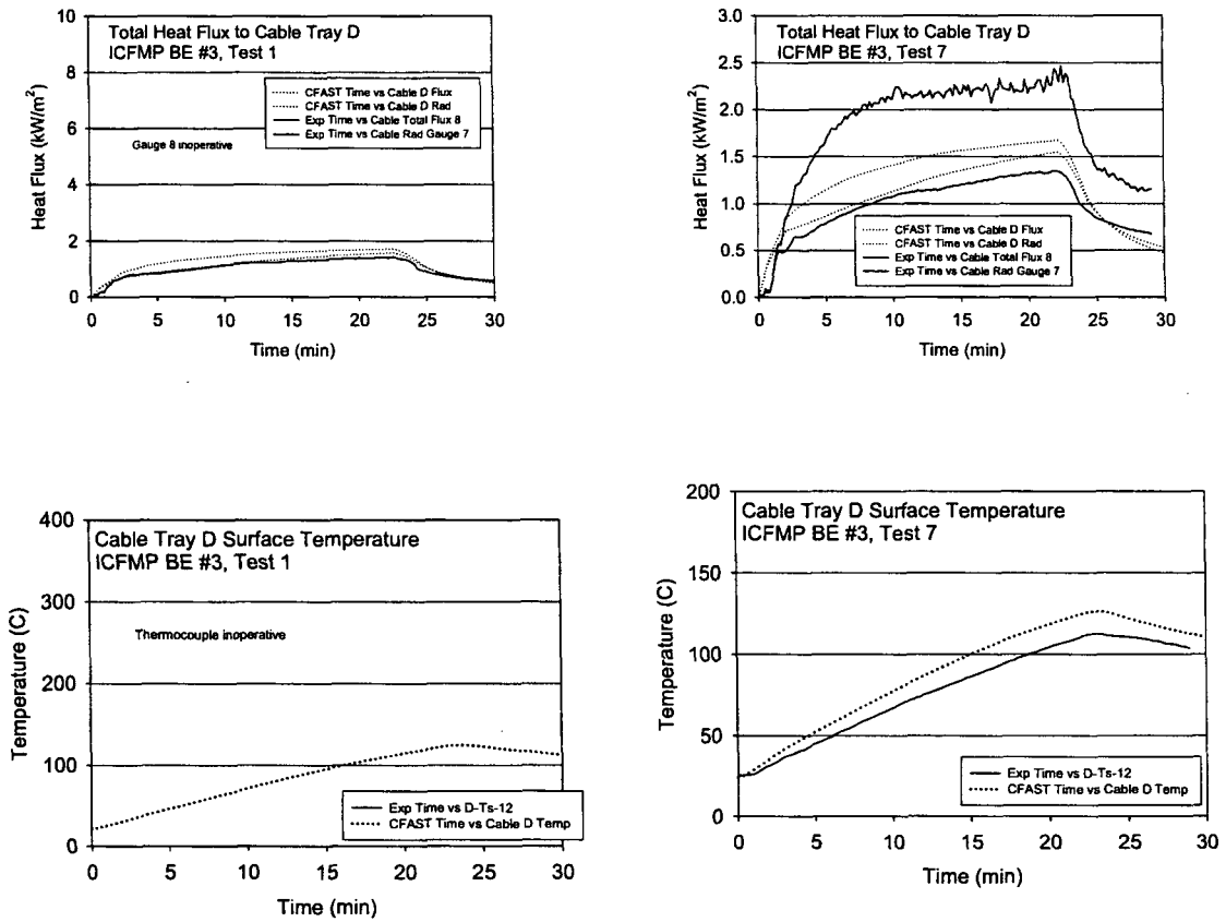
Figure A-37. Thermal Environment near Cable Tray D, ICFMP BE #3, Tests 1 and 7
