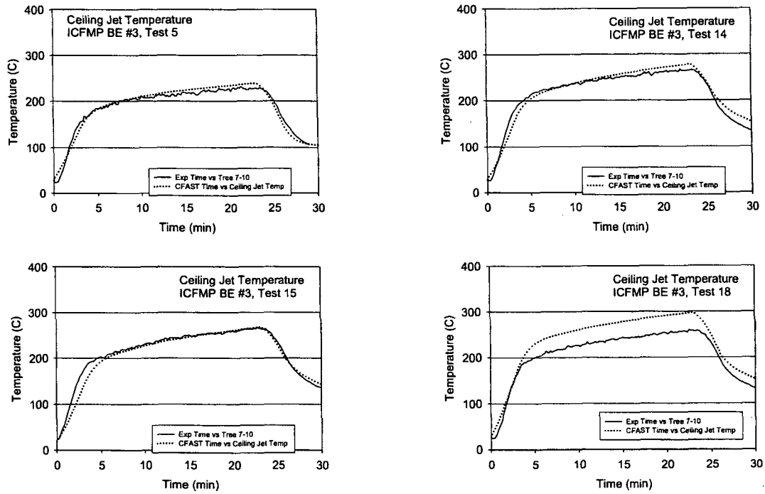
Figure A-20. Ceiling Jet Temperature, ICFMP BE #3, Open-Door Tests
