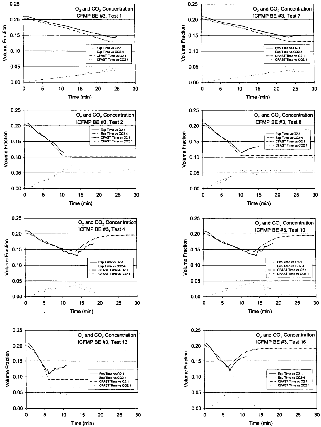
Figure A-24. Oxygen and Carbon Dioxide Concentration, ICMP BE #3, Closed-Door Tests
