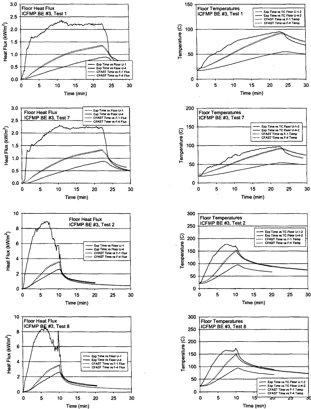
Figure A-73. Floor Heat Flux and Surface Temperature, ICMP BE #3, Closed-Door Tests
