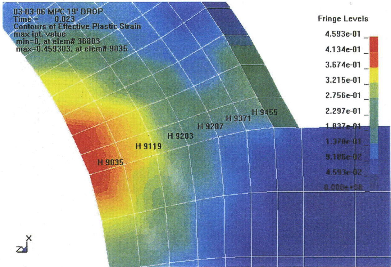
Figure A.30. Labels the Elements Through the Shell Thickness at the Junction of the Shell And Baseplate at the Location of Maximum EPS
