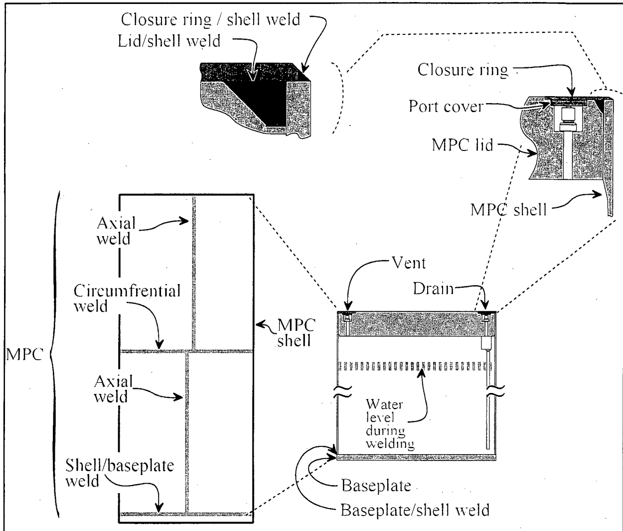
Figure B.1. Major Welds of the MPC
