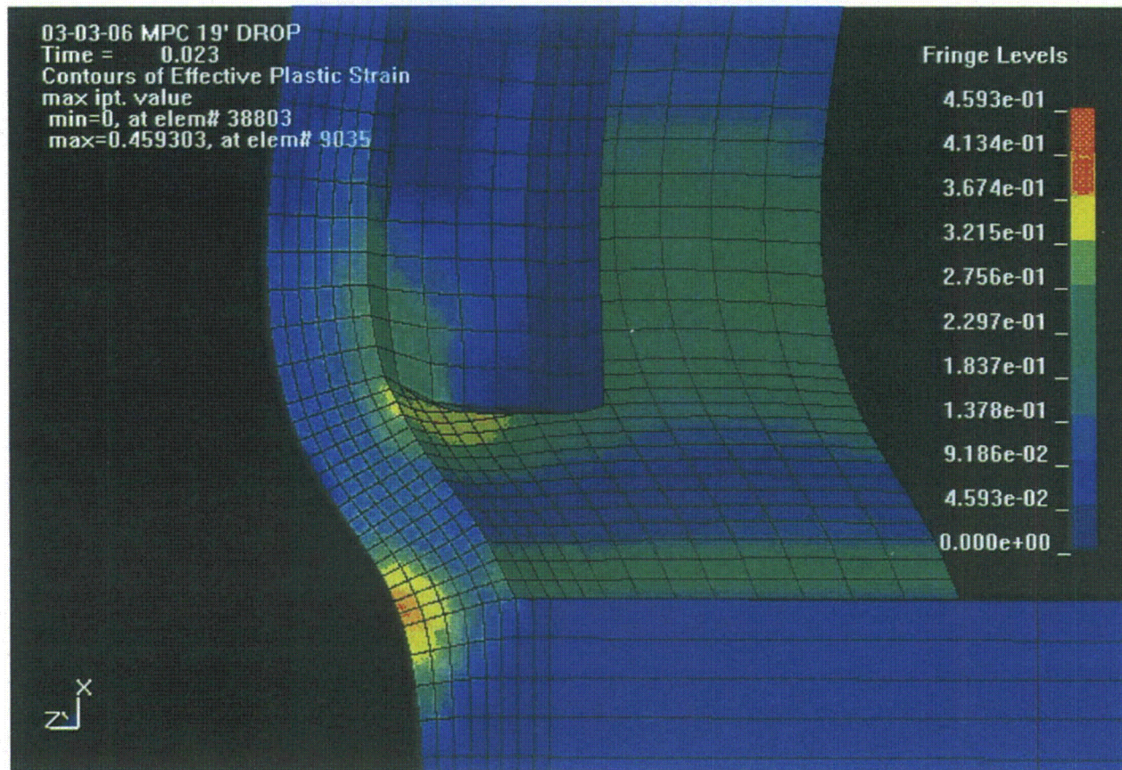
Figure B.3. Deformation and Contours of EPS in the Vicinity of the Stitch Weld Attaching the Basket Support to the Shell
