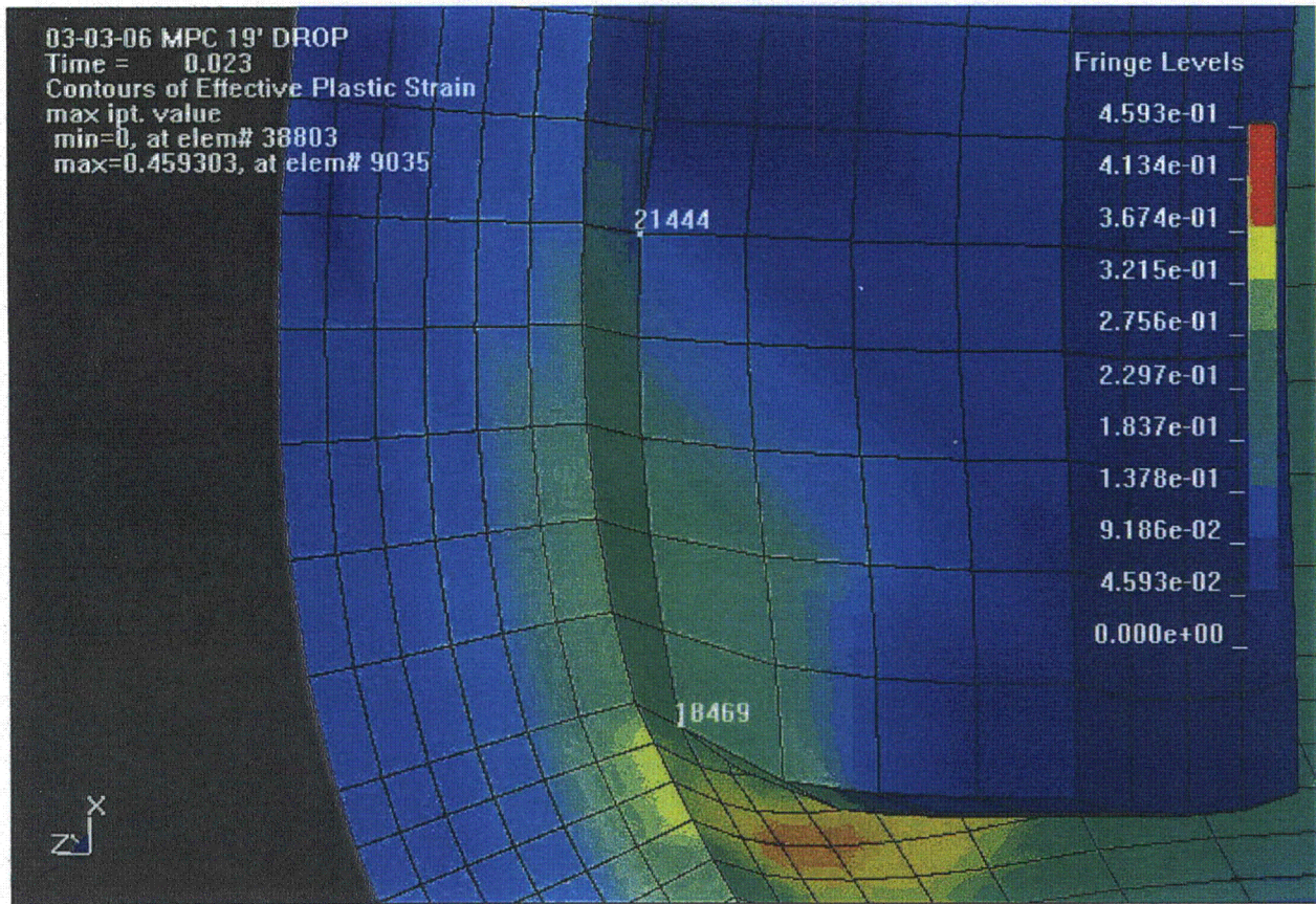
Figure B.4. Shear Deformation and Shear-Lag Are Evident in the Elements of the Support at the Location of the Fillet Weld Between Nodes 18469 and 21444
