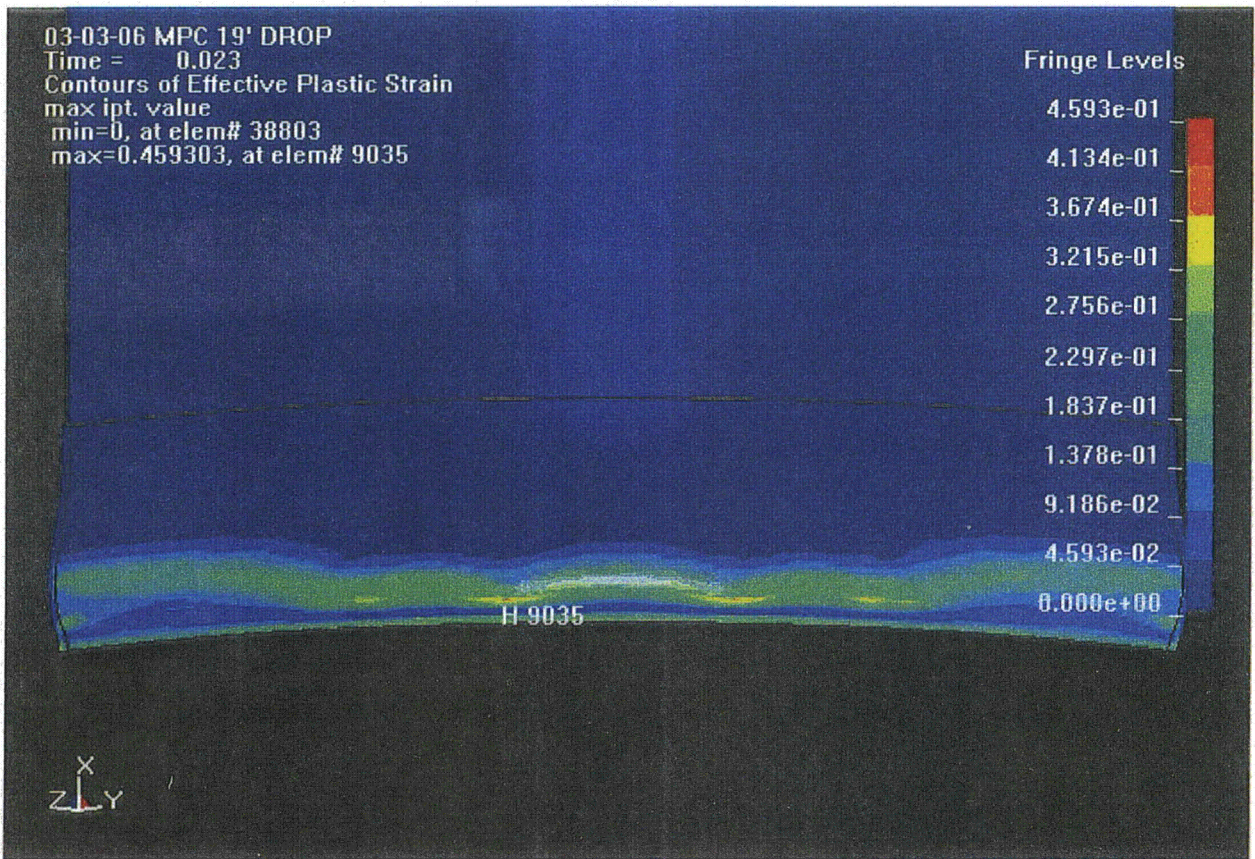
Figure A.24. With the Basket Supports Removed from Figure A22, Figure A.24 Shows the Location of Element 9035 Where the Maximum EPS of 0.459 Occurs
