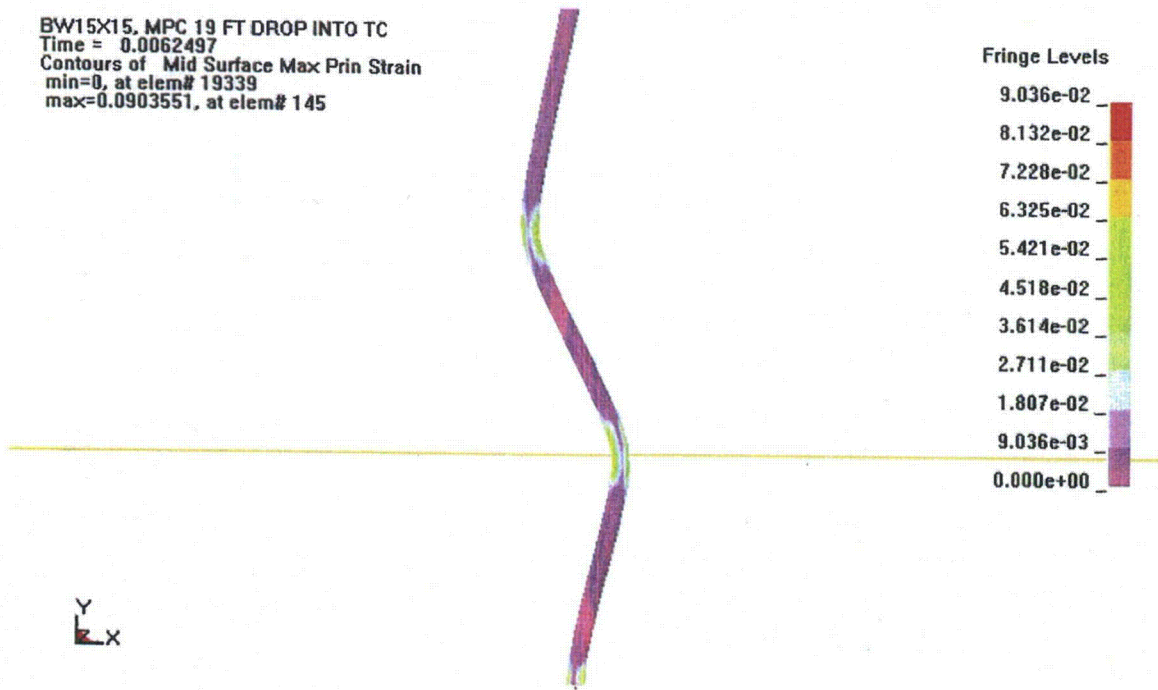
Figure C.17. Maximum Principal Strain at Time of Maximum Response (19-Foot Drop)
