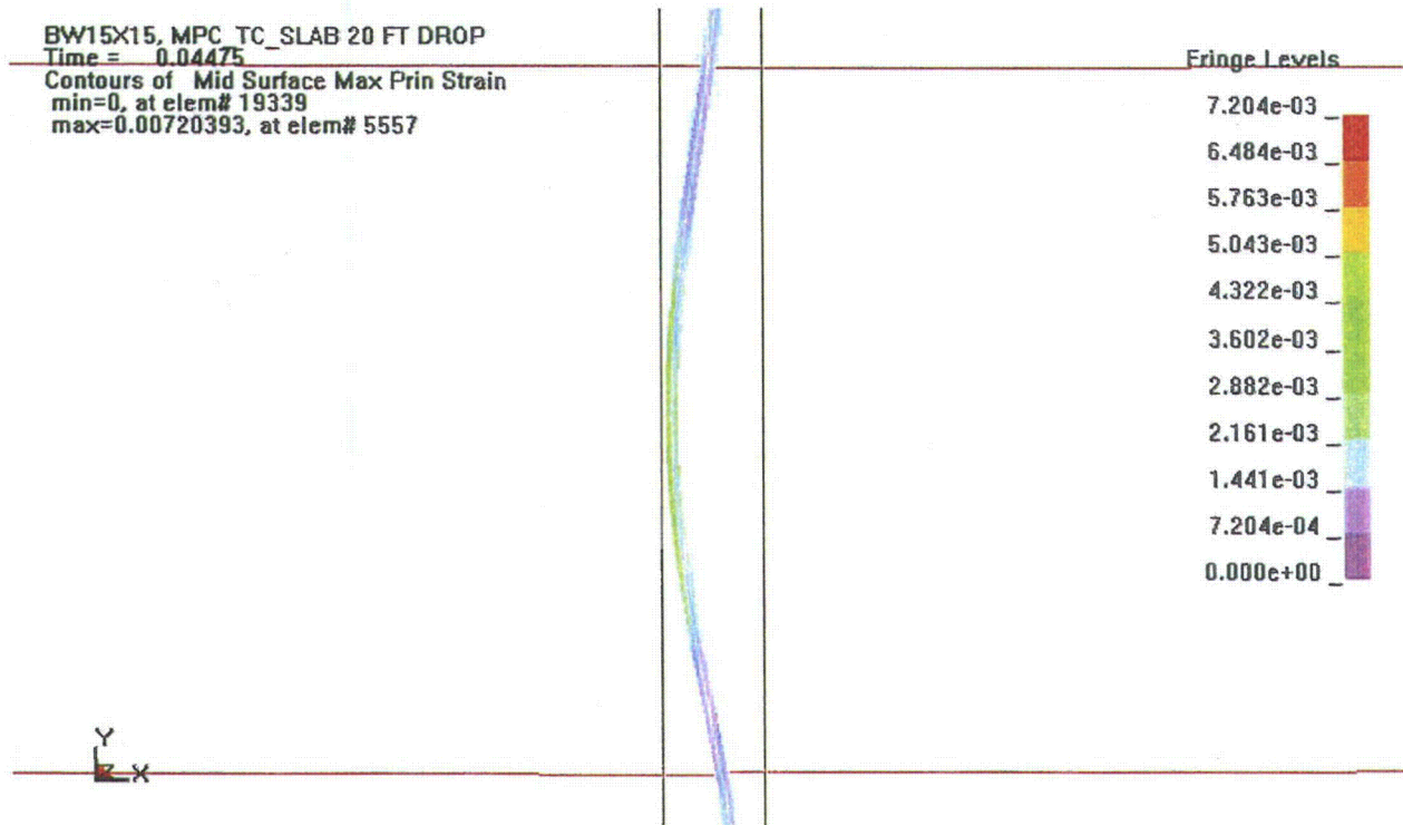
Figure C.5. Maximum Principal Strain at Time of Maximum Response (20-Foot Drop)
