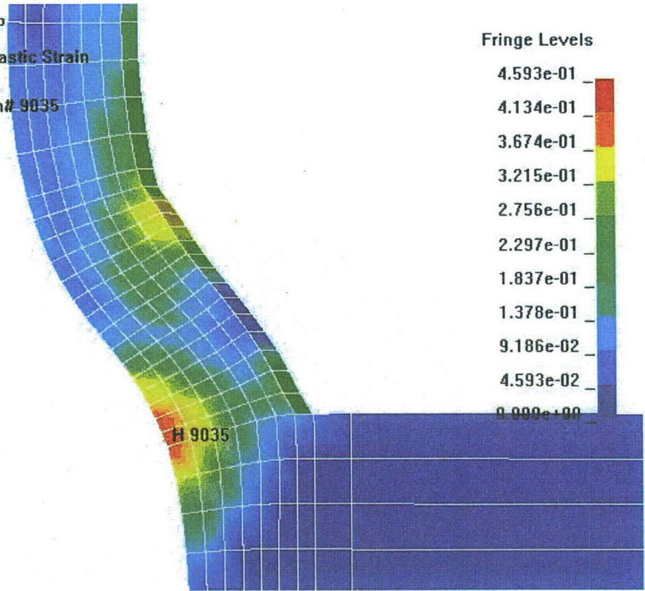
Figure A.29. Slice Through the MPC Shell and Baseplate Showing the Location of Element 9035 and the Local Distribution of EPS Within the Shell
