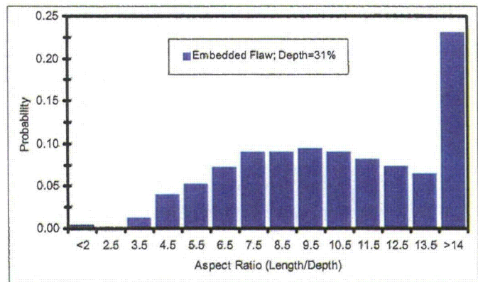
Figure B.11. Distribution of Aspect Ratios for an Embedded Flaw with a Depth of 31% of the Weld Thickness
