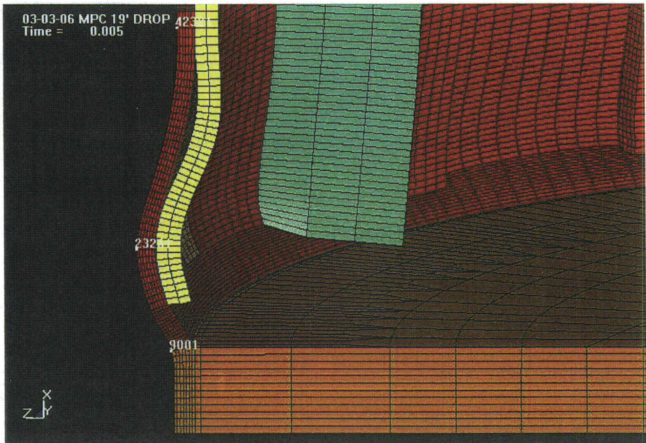
Figure A.19. Displacement of the MPC Shell and Basket Support Along the xz Plane of Symmetry at the Time of Maximum Displacement (0.005 seconds)
