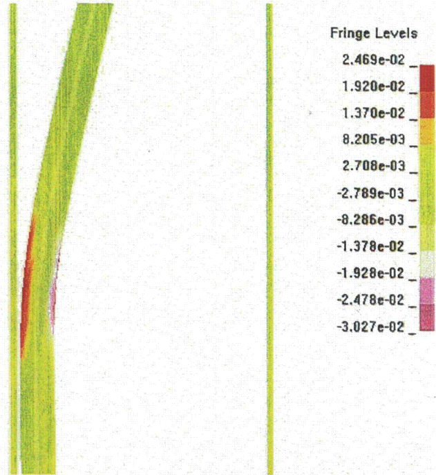
Figure C.15. Closer View of Figure C.14 Showing the Longitudinal Strain Distribution (55-Foot Drop)
