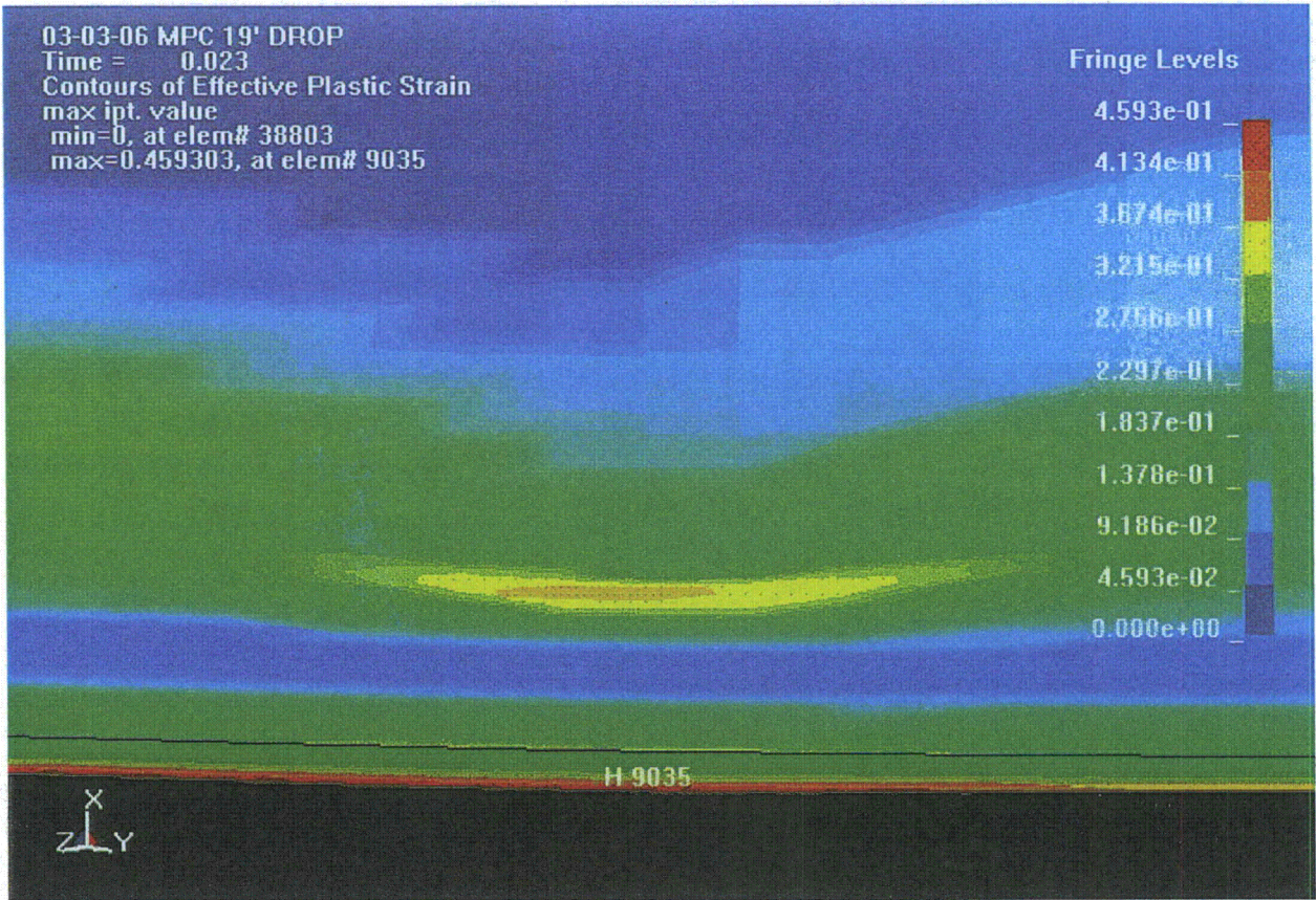
Figure A.25. Closeup View of the Location of Element 9035 On the Bottom Outside Edge of the MPC Shell
