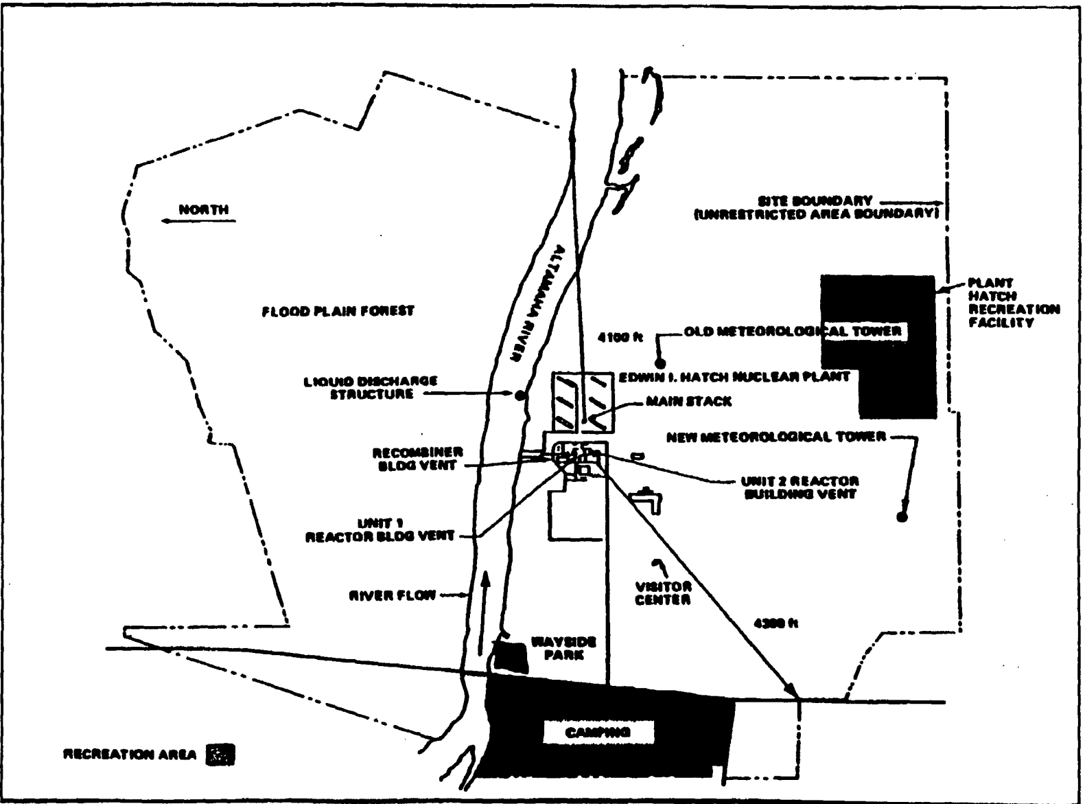
Figure 10-1 Site Map for Effluent Controls
