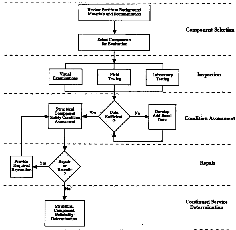
Figure 5.2 Evaluation methodology for nuclear power plant concrete structures.
