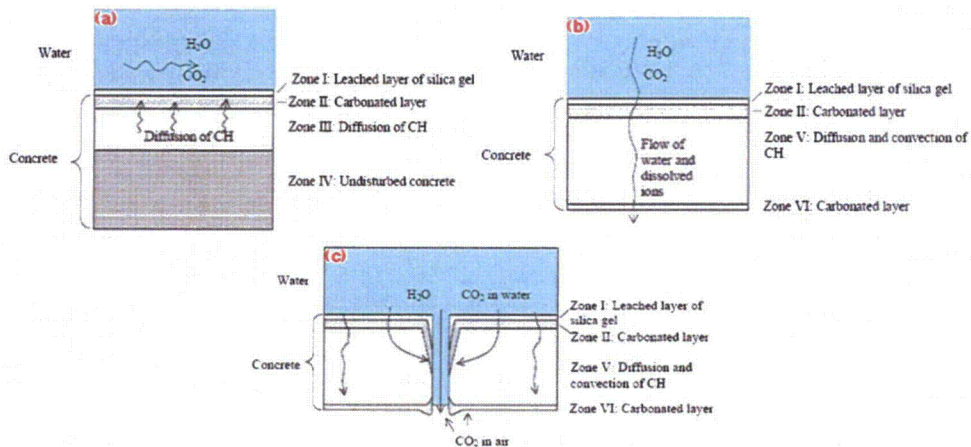
Figure 4.13 Conceptual models for concrete leaching mechanisms: (a) leaching from free surfaces, (b) homogeneous percolation through porous concrete, and (c) leaching from surfaces of cracks. CH = calcium hydroxide.
