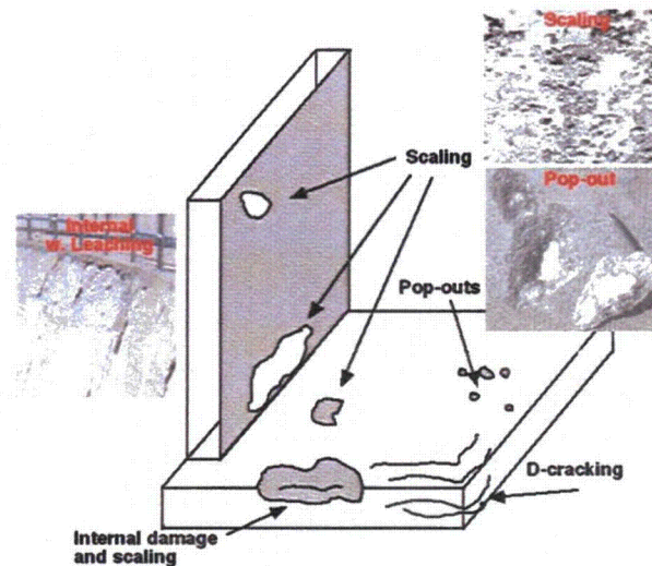
Figure 4.4 Types of freeze-thaw damage.
