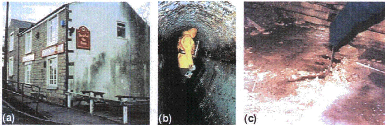
Figure 4.21 Concrete biological attack: (a) algae growth on outside wall of house, (b) biogenic sulfuric acid attack in sewer system, (c) decaying concrete floor in flooded cellar.
