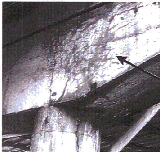
Figure 4.16 Cracking damage in a concrete structure due to DEF.
