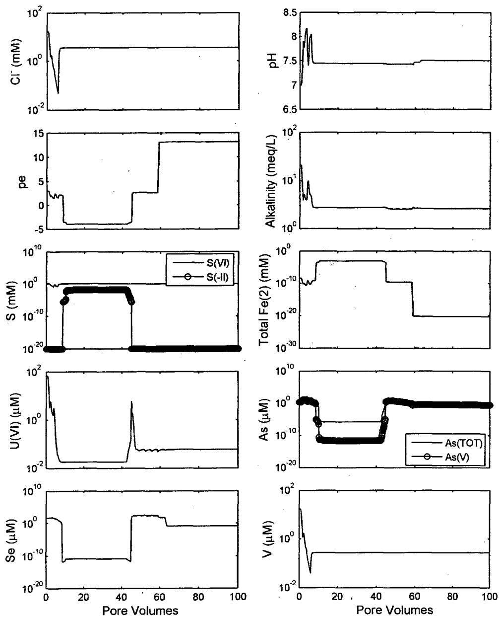
Figure 30. Simulation 13 results. Influent groundwater pH changed to 7.5. Oxic influent groundwater. Calcite, goethite, and elemental Se (50 ppm) initially present. 265 mg/L of H_2S(g) added to the influent water during pore volumes 3.0 to 3.6. Pyrite and uraninite precipitation not allowed. Amorphous FeS and UO_2 precipitation allowed. Mass transfer coefficient = 10. Sulfide concentration indicated at 1 \times 10^{-20} M is actually \leq 1 \times 10^{-20} M in plot.
