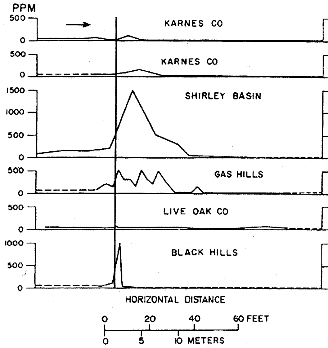
Figure 7. Concentration and distribution of vanadium in various uranium roll front deposits (after Harshman, 1974).
