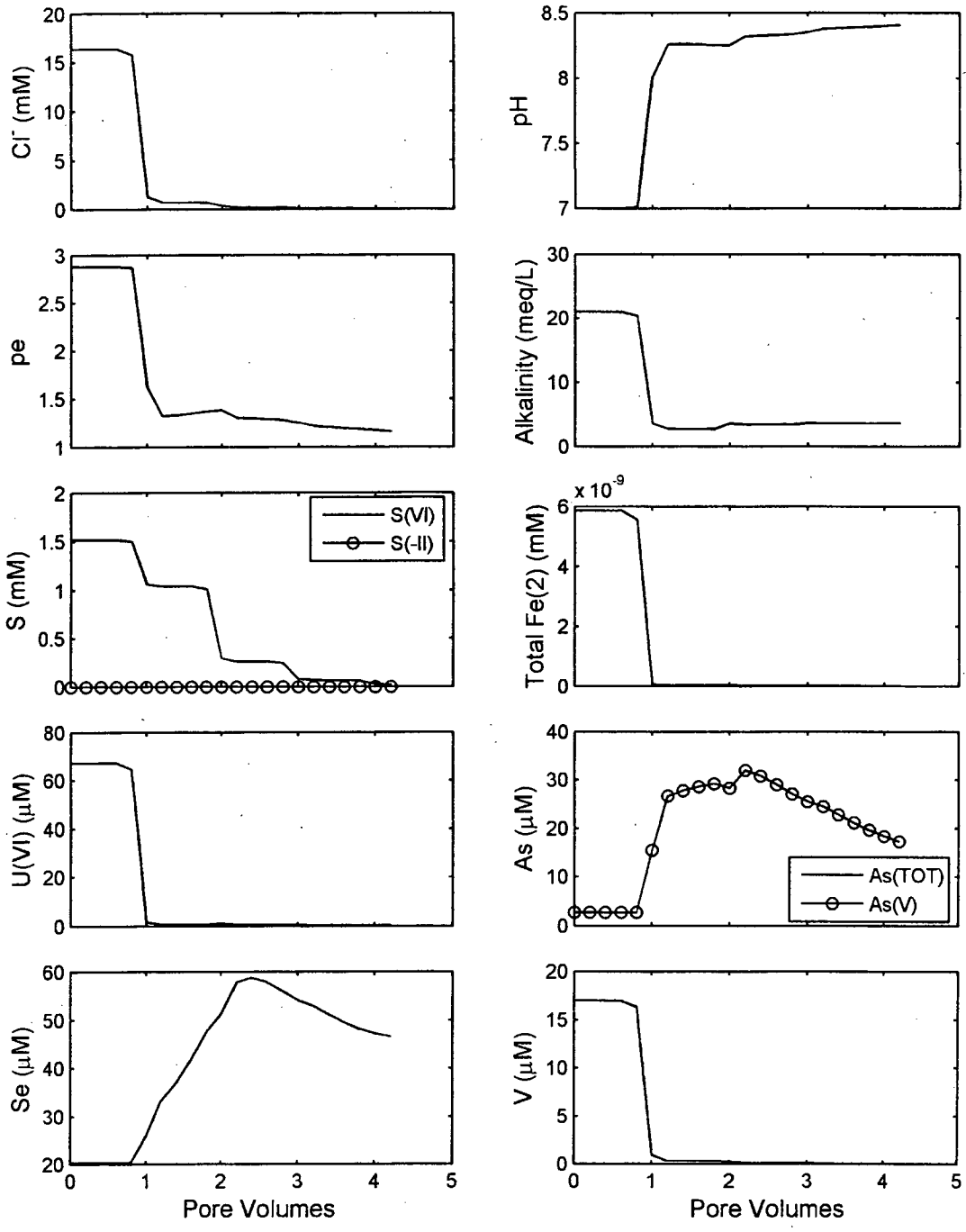
Figure 17. Simulation 6 results. Oxic influent groundwater. Calcite and goethite initially present in all cells. Elemental Se initially present at 50 ppm in the mobile cells. Elemental Se (500 ppm), pyrite (2000 ppm), and uraninite (1000 ppm) initially present in the immobile cells. Mass transfer coefficient = 10^{-4} .
