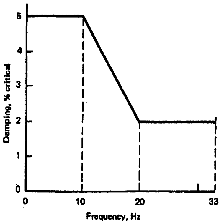
Figure 1 Frequency-dependent damping
