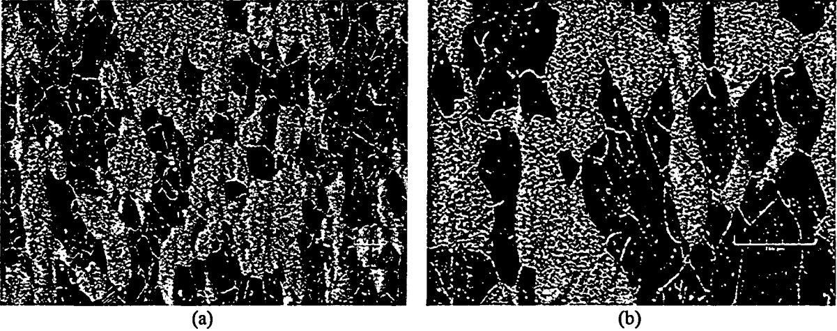
Figure 64. Microstructure of the round robin alloy in the plane of the crack at two magnifications.
