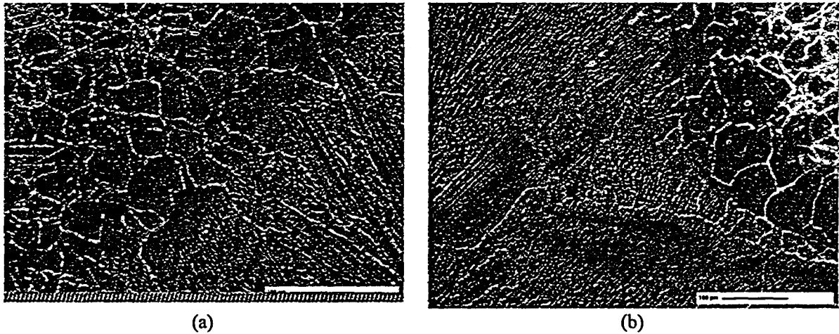
Figure 68. Large grain microstructure in the HAZ at two opposite positions (a and b).
