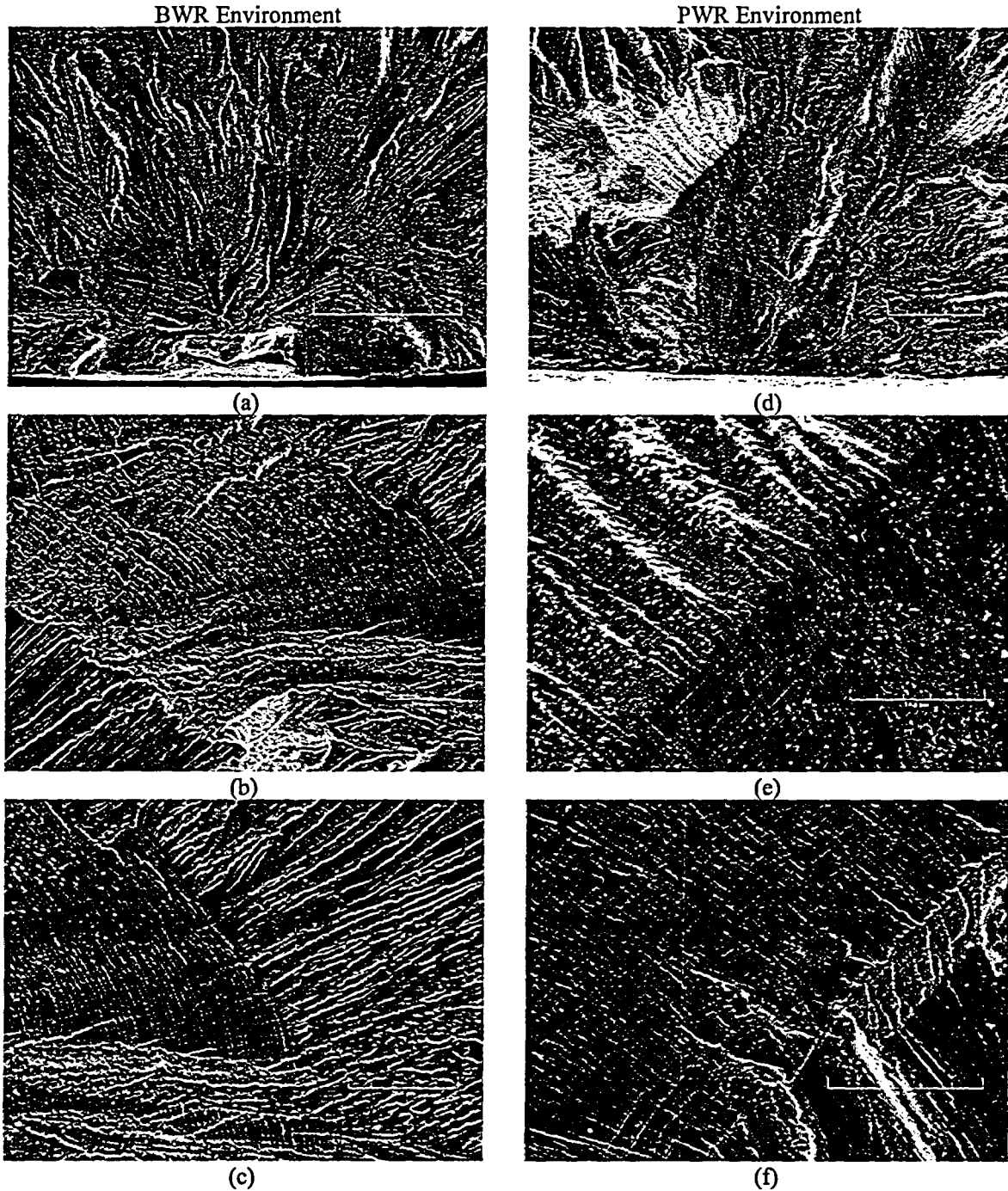
Figure 17. Photomicrographs showing crack initiation site and striations at select locations in Type 316NG SS tested in (a–c) BWR and (d–f) PWR environment.
