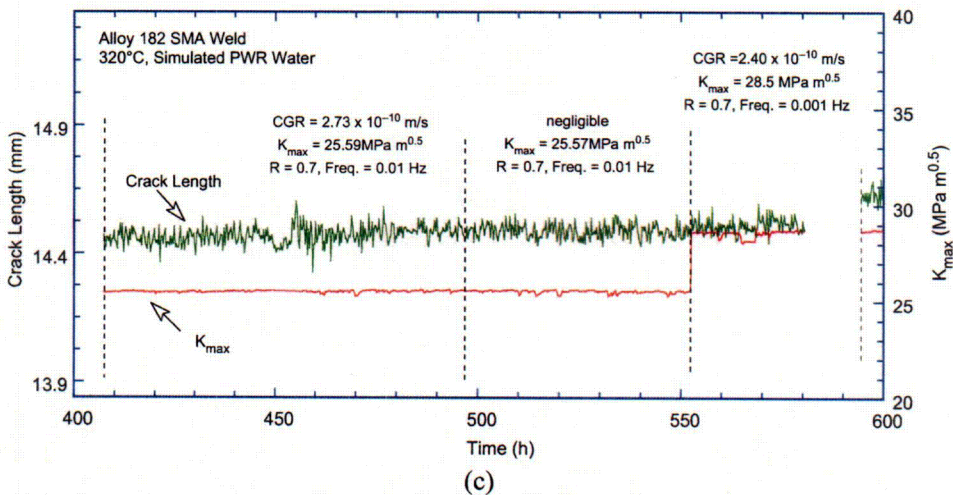
Figure 85. Crack length vs. time plot for Alloy 182 SMA weld-metal specimen in simulated PWR environment at 320°C during test periods (a) 1-4a, (b) 4b-5, (c) 6-8, (d) 9, and (e) 10.
