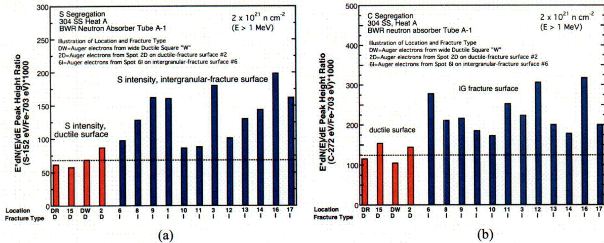
Figure 23. Summary of AES analysis of grain-boundary segregation of S (a) and C (b) in BWR neutron absorber tube fabricated from Type 304 SS Heat A and irradiated to 3 dpa: S and C peak heights from ductile (denoted "D") and IG (denoted "I") fracture surfaces are compared.
