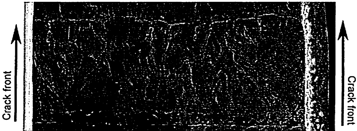
Figure 54. Micrograph of the fracture surface of Specimen GG3B-A-TT tested in high-DO water at 289°C.
