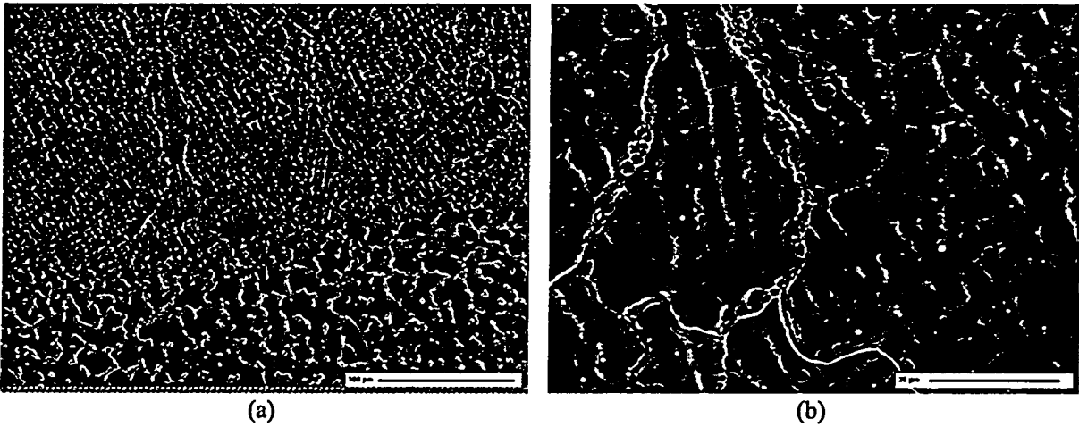
Figure 71. (a) Dendritic microstructure on sample 3B and (b) high magnification of a region from (a).
