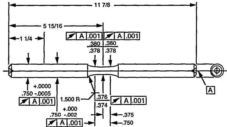
Figure 2. Configuration of fatigue test specimen (all dimensions in inches).
