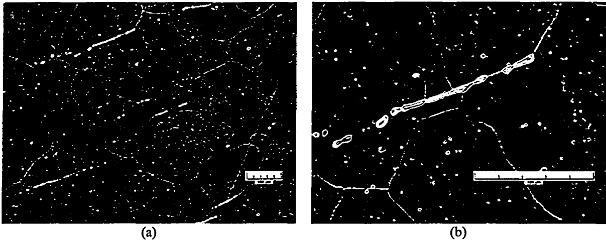
Figure 31. (a) Low- and (b) high-magnification photomicrographs of the structure of the Type 304L base metal from the top shell of the H5 weld of the Grand Gulf core shroud.
