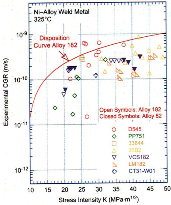
Figure 93. Comparison of the SCC growth rate for the Argonne Alloy 182 weld with the available data for Alloy 182 and 82 welds in simulated PWR environment. All results normalized to 325°C using an activation energy of 130 kJ/mole. Data from Refs. 107–114.
