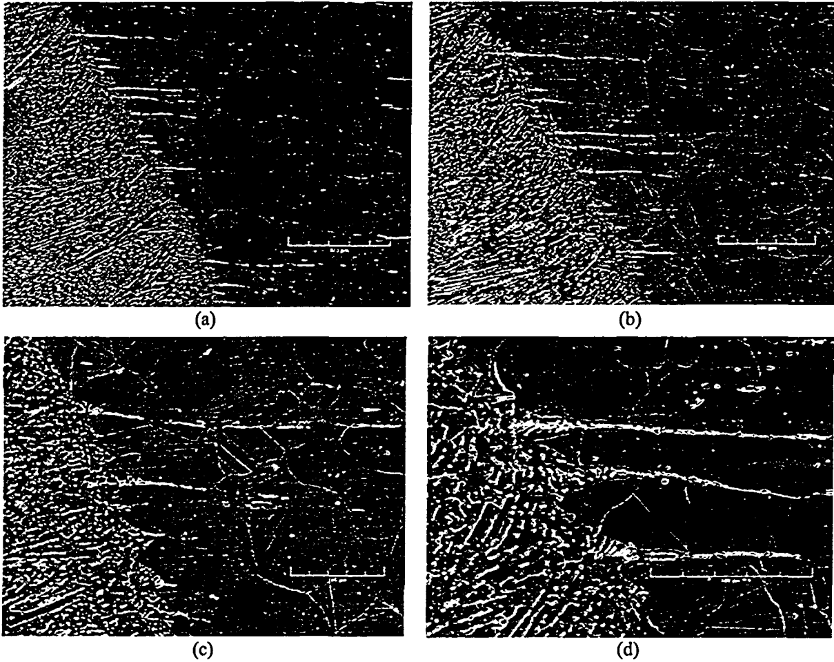
Figure 36. Micrographs of the interface between the weld metal and base metal.
