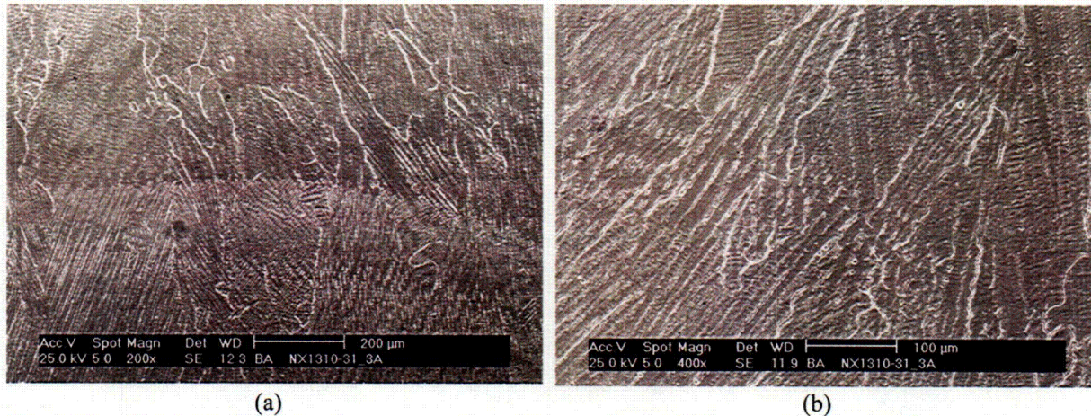
Figure 72. Dendritic microstructure observed on the surface of sample 3A at (a) 100 \times and (b) 200 \times magnifications.
