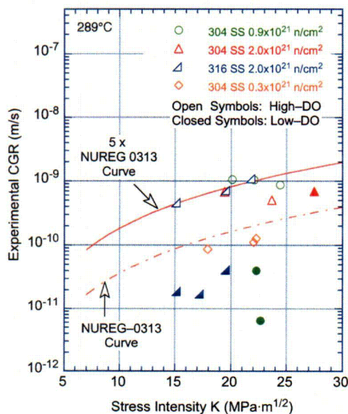
Figure 41. CGR data under constant load with periodic partial unloads for irradiated austenitic SSs in high-purity water at 289°C.
