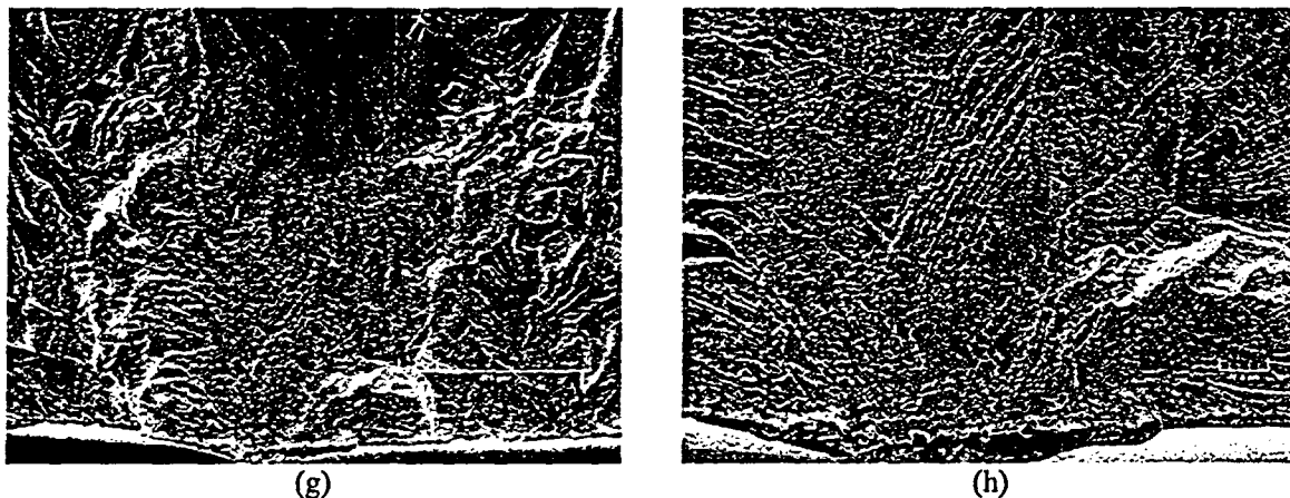
Figure 10. Photomicrographs showing the sites of crack initiation on the fracture surfaces of Type 304 SS specimen tested in simulated PWR environment: (a), (c), (e), (g) low magnification; (b), (d), (f), (h) high magnification.
