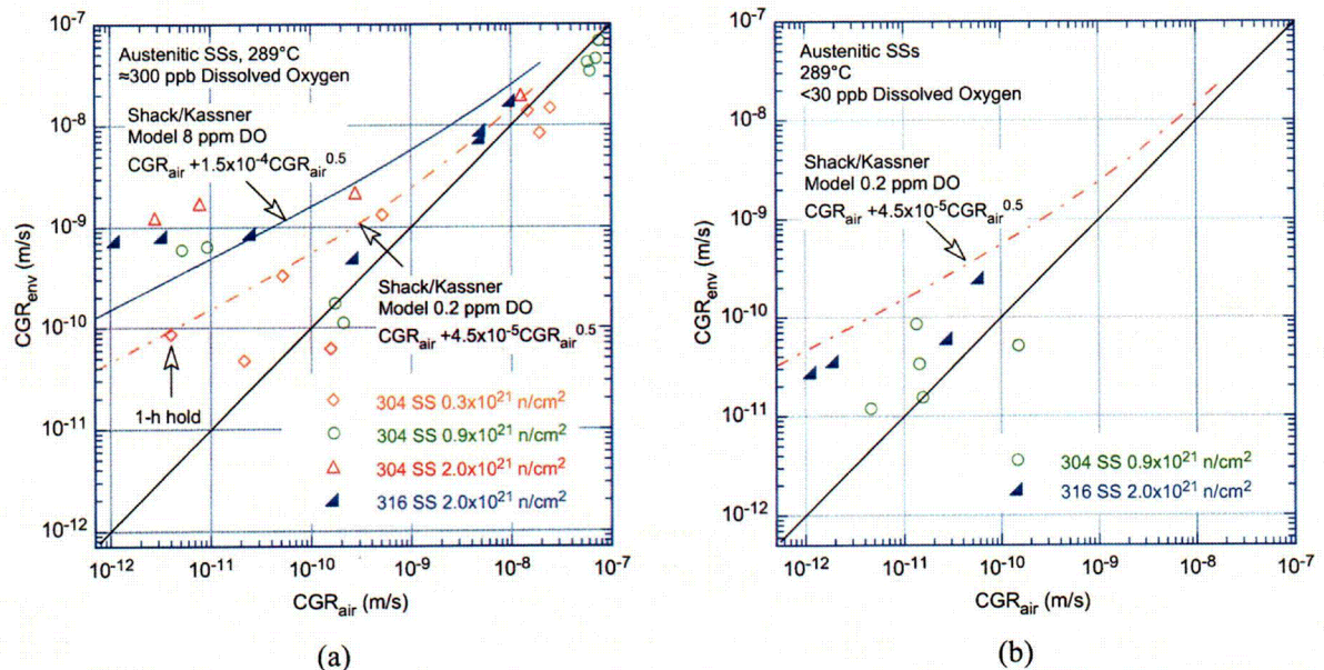
Figure 40. CGR data for irradiated austenitic SSs under continuous cycling at 289°C in high-purity water with (a) \approx 300 ppb and (b) < 30 ppb dissolved oxygen.
