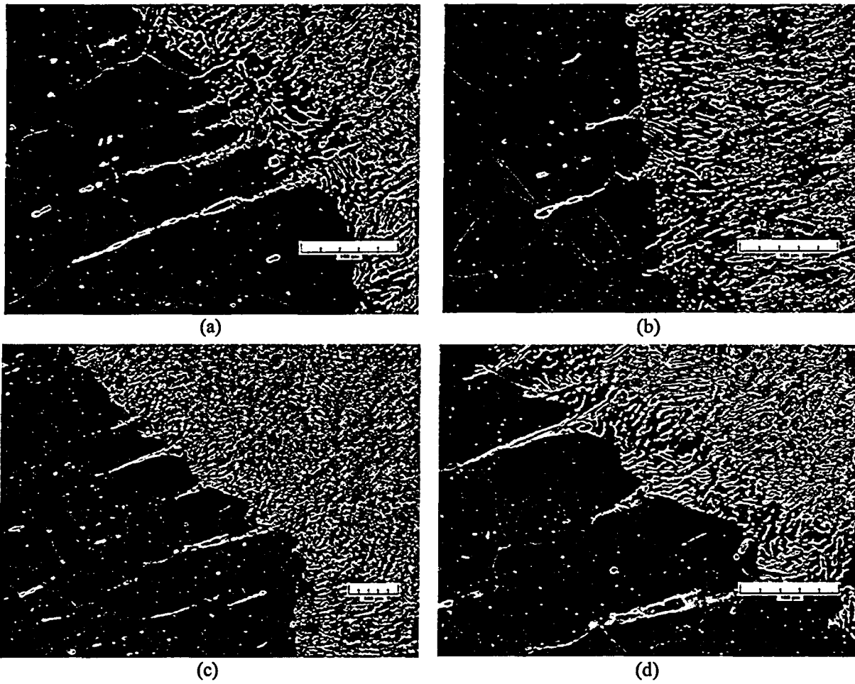
Figure 32. Micrographs of the interface between the weld metal and top shell of the H5 weld of the Grand Gulf core shroud.
