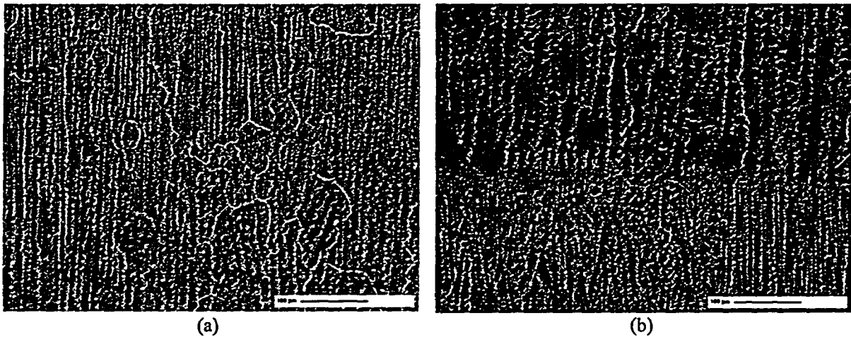
Figure 69. (a) Dendritic microstructure on sample 3A, and (b) at a weld pass.
