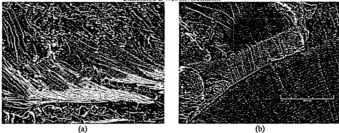
Figure 11. (a) Low- and (b) high-magnification photomicrographs showing striations at select locations on fracture surfaces of MA specimen of Heat 30956 in simulated BWR environment.
