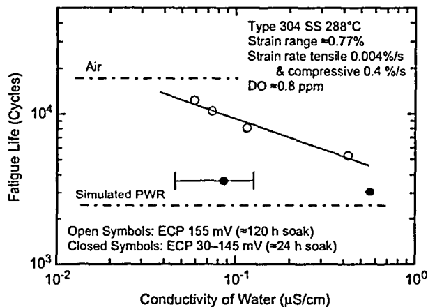
Figure 46. Effects of conductivity of water and soaking period on fatigue life of Type 304 SS in high-DO water (Ref. 7,37).
