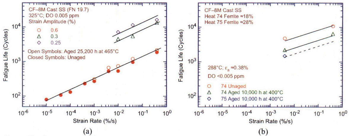
Figure 53. Dependence of fatigue lives of CF-8M cast SSs on strain rate in low-DO water at various strain amplitudes (Refs. 23,28,36,37).
