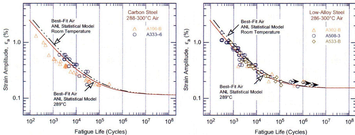
Figure 4. Fatigue strain vs. life data for carbon and low-alloy steels in air at 288°C (JNUFAD database, and Refs. 4,12,13,41-42).
