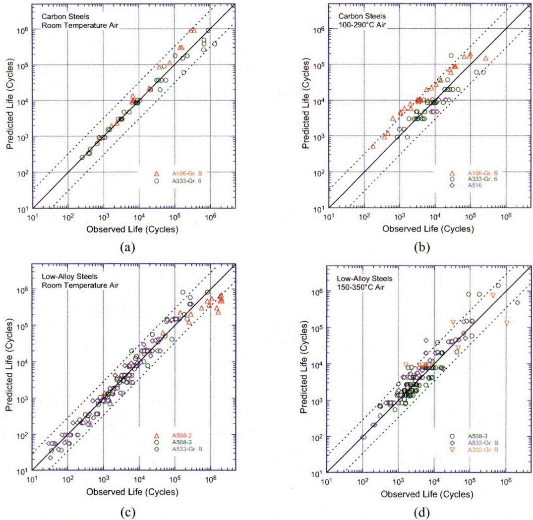
Figure 8. Experimental and predicted fatigue lives of (a, b) carbon steels and (c, d) low-alloy steels in air.
