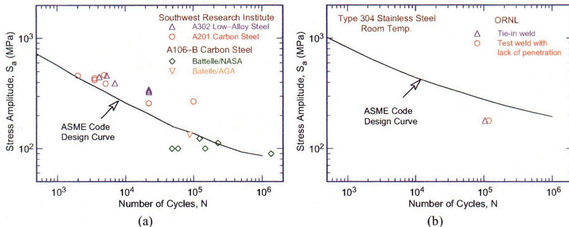
Figure 56. Fatigue data for (a) carbon and low-alloy steel and (b) Type 304 stainless steel components (Refs. 115,116).
