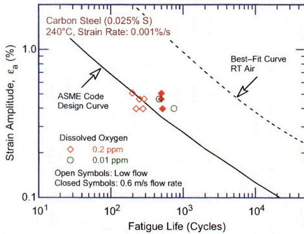
Figure 25. Effect of flow rate on low-cycle fatigue of carbon steel tube bends in high-purity water at 240°C (Ref. 43). RT = room temperature.
