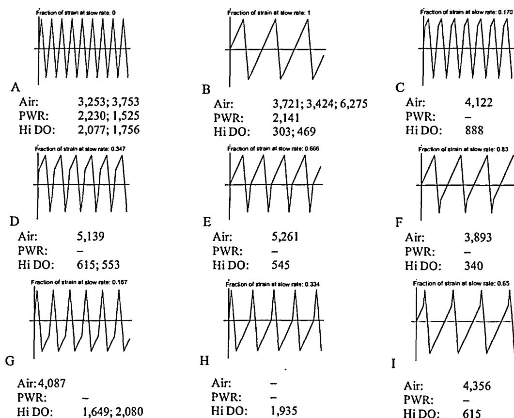
Figure 13. Fatigue life of A106-Gr B carbon steel at 288°C and 0.75% strain range in air and water environments under different loading waveforms (Ref. 4).
