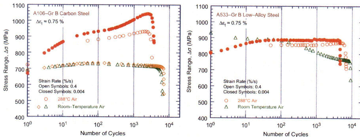
Figure 5. Effect of strain rate and temperature on cyclic stress of carbon and low-alloy steels.
