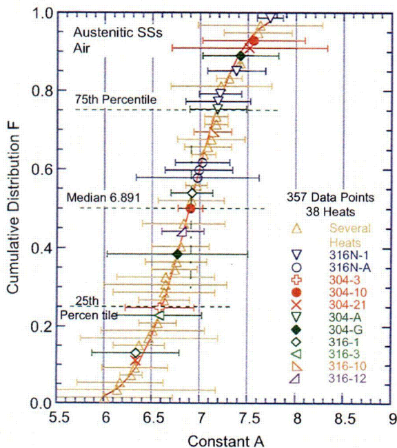
Figure 35. Estimated cumulative distribution of constant A in statistical model for fatigue life for heats of austenitic SS in air.
