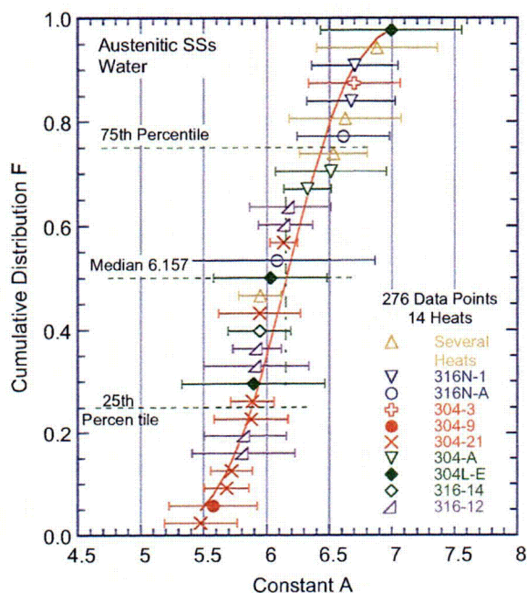
Figure 52. Estimated cumulative distribution of constant A in statistical model for fatigue life for heats of austenitic SSs in water.
