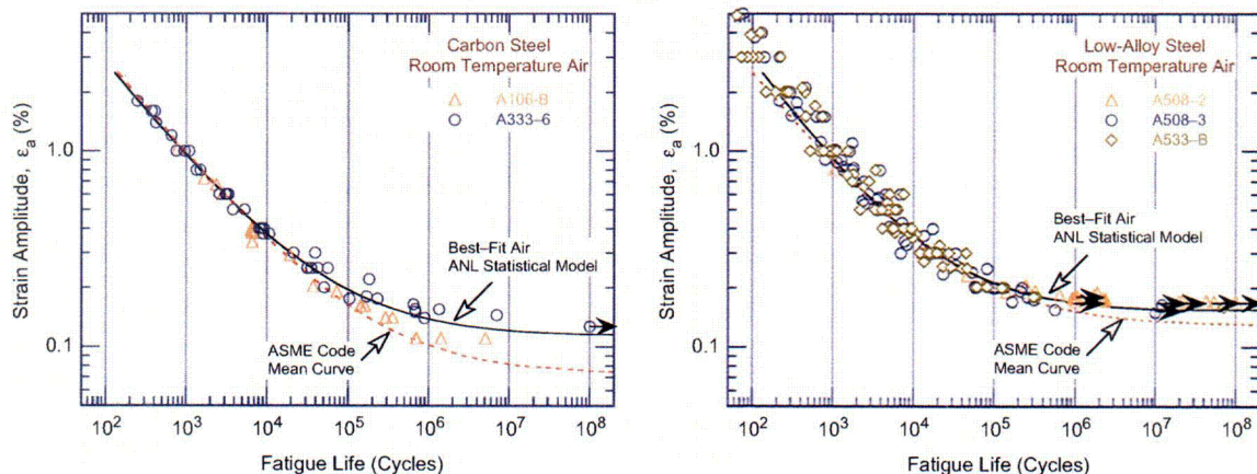
Figure 3. Fatigue strain vs. life data for carbon and low-alloy steels in air at room temperature (JNUFAD database and Refs. 4,12,13,40).
