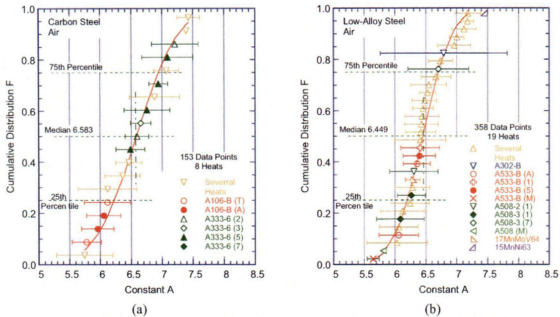
Figure 7. Estimated cumulative distribution of constant A in statistical models for fatigue life with heats of (a) carbon steels and (b) low-alloy steels in air.
