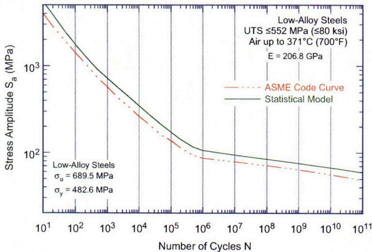
Figure 10. Fatigue design curve for low-alloy steels in air. The curve developed from the statistical model is based on factors of 12 on life and 2 on stress.
