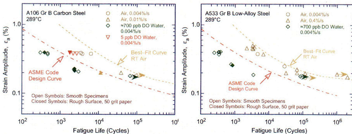
Figure 26. Effect of surface roughness on fatigue life of (a) A106-Gr B carbon steel and (b) A533 low-alloy steel in air and high-purity water at 289°C.
