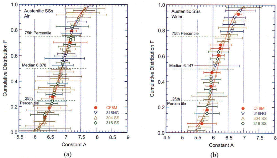
Figure 54. Estimated cumulative distribution of constant A in statistical models for fatigue life of wrought and cast austenitic stainless steels in (a) air and (b) water environments.
