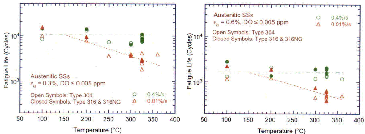
Figure 47. Change in fatigue lives of austenitic stainless steels in low-DO water with temperature (Refs. 7,23–25,28,37–39).
