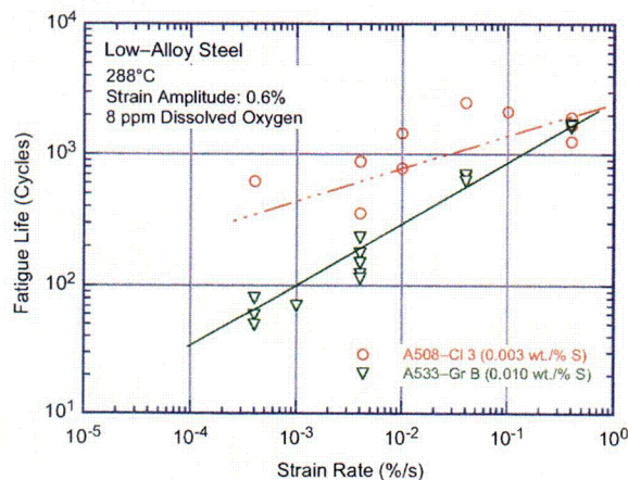
Figure 21. Effect of strain rate on fatigue life of low-alloy steels with different S contents (JNUFAD database and Ref. 4).
