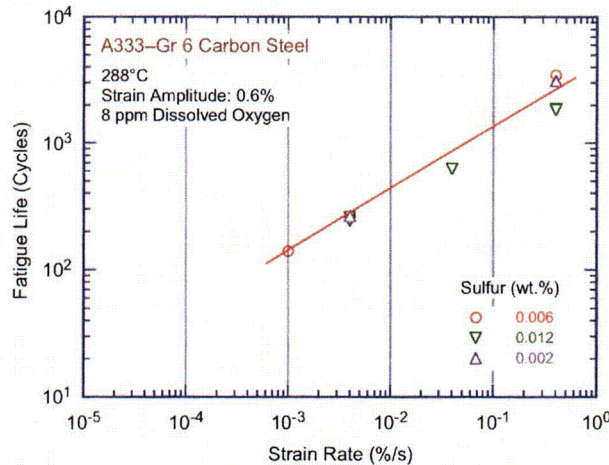
Figure 22. Effect of strain rate on the fatigue life of A333-Gr 6 carbon steels with different S contents.
