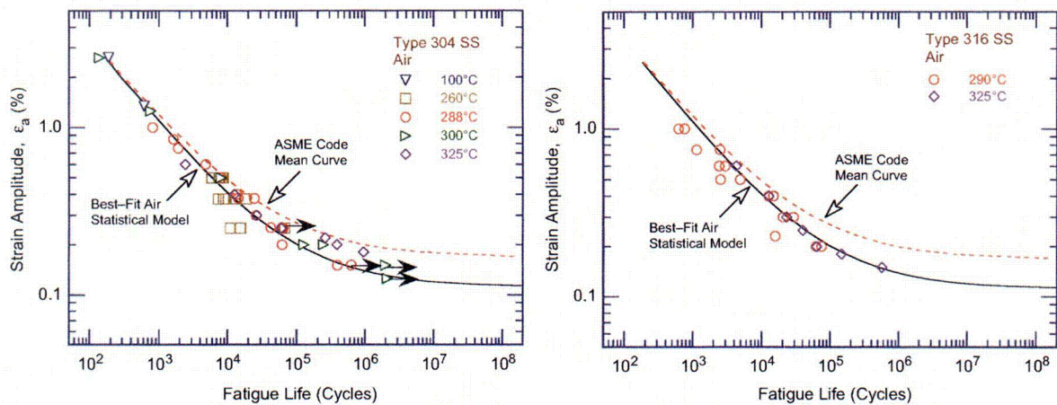
Figure 32. Influence of temperature on fatigue life of Types 304 and 316 stainless steel in air (Ref. 37, JNUFAD database).
