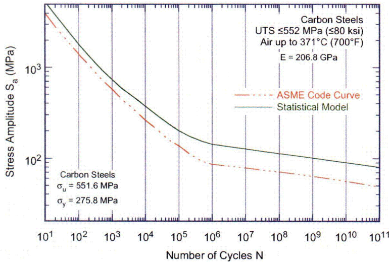
Figure 9. Fatigue design curve for carbon steels in air. The curve developed from the statistical model is based on factors of 12 on life and 2 on stress.
