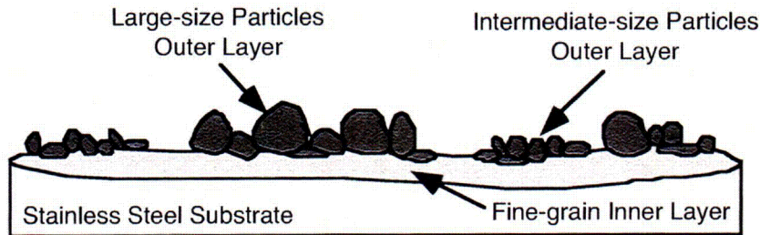
Figure 40. Schematic of the corrosion oxide film formed on austenitic stainless steels in LWR environments.
