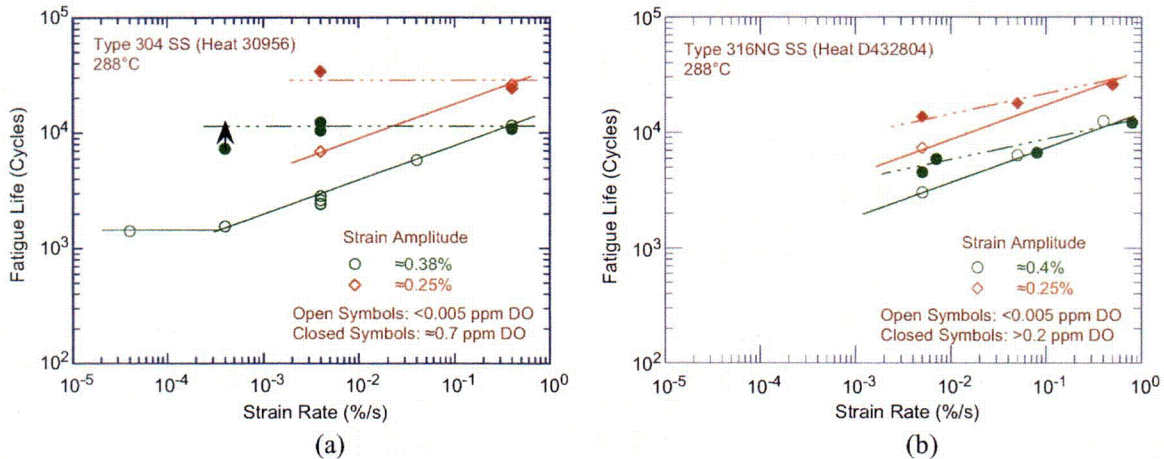
Figure 45. Dependence of fatigue life of Types (a) 304 and (b) 316NG stainless steel on strain rate in high- and low-DO water at 288°C (Ref. 7,37,39).
