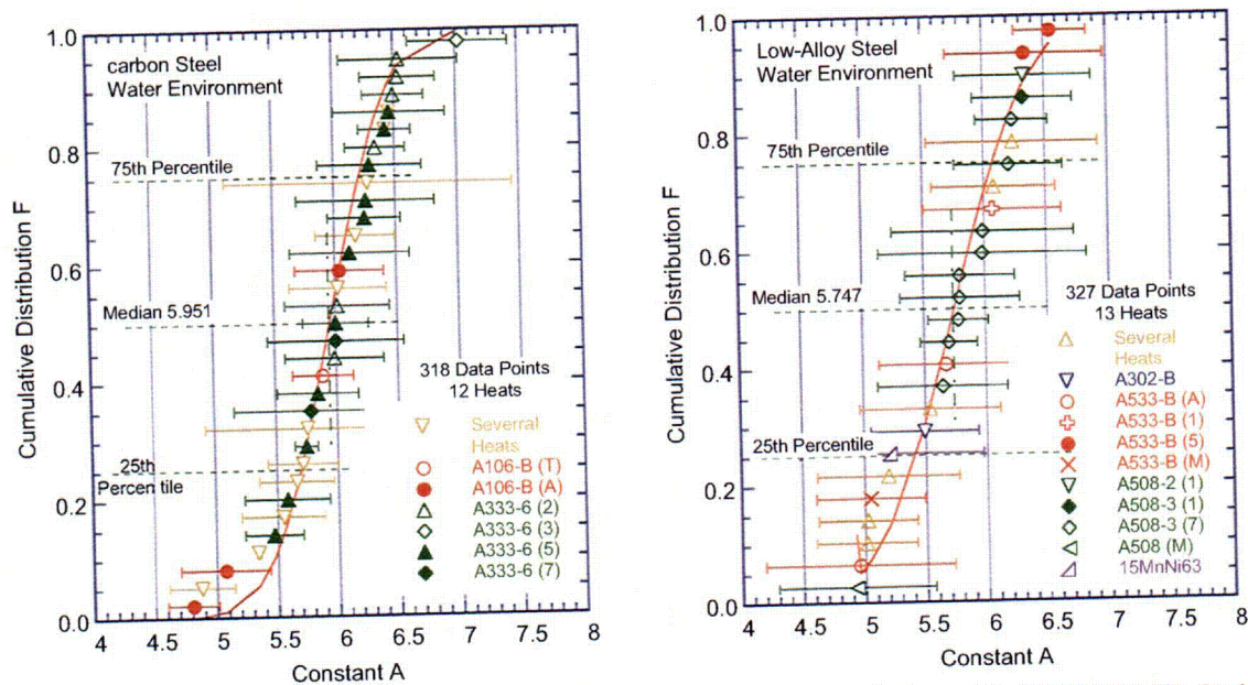
Figure 27. Estimated cumulative distribution of parameter A in statistical models for fatigue life for heats of carbon and low-alloy steels in LWR environments.
