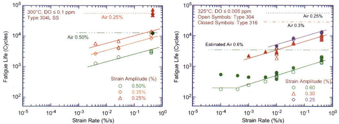
Figure 44. Dependence of fatigue lives of austenitic stainless steels on strain rate in low-DO water (Refs. 7,37,39,69).
