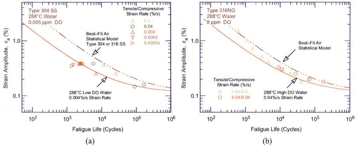
Figure 38. Strain amplitude vs. fatigue life data for (a) Type 304 and (b) Type 316NG SS in water at 288°C (JNUFAD and Refs. 7,37).
