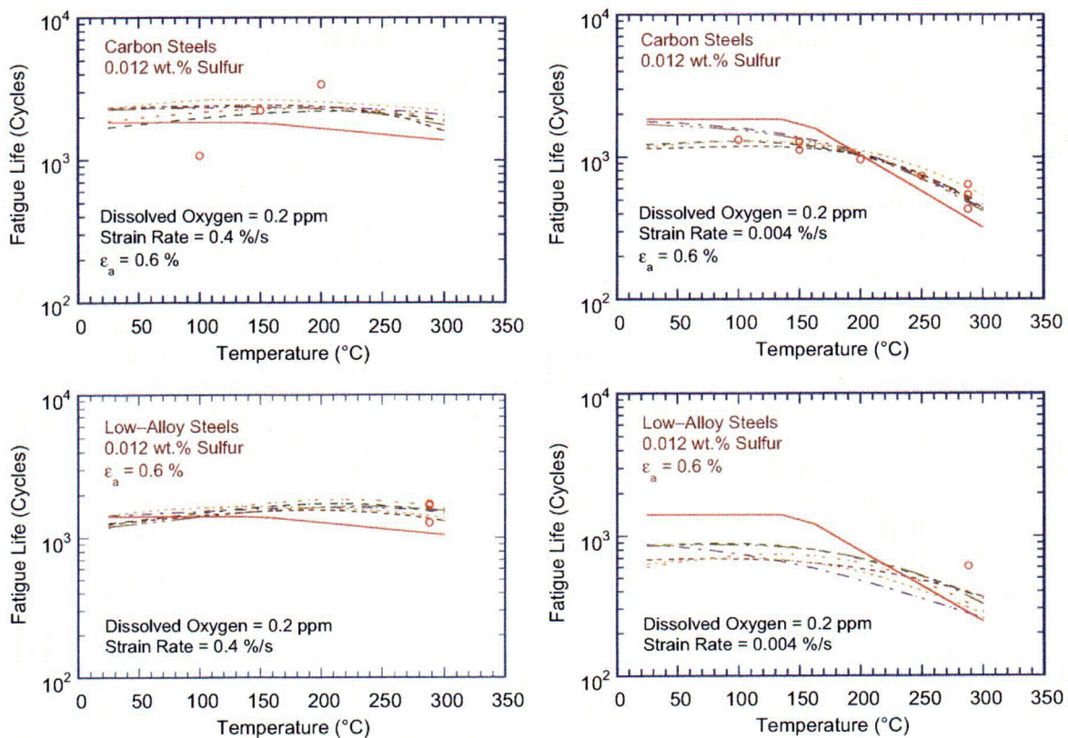
Figure 17. Dependence of fatigue life on temperature for carbon and low-alloy steels in water.
