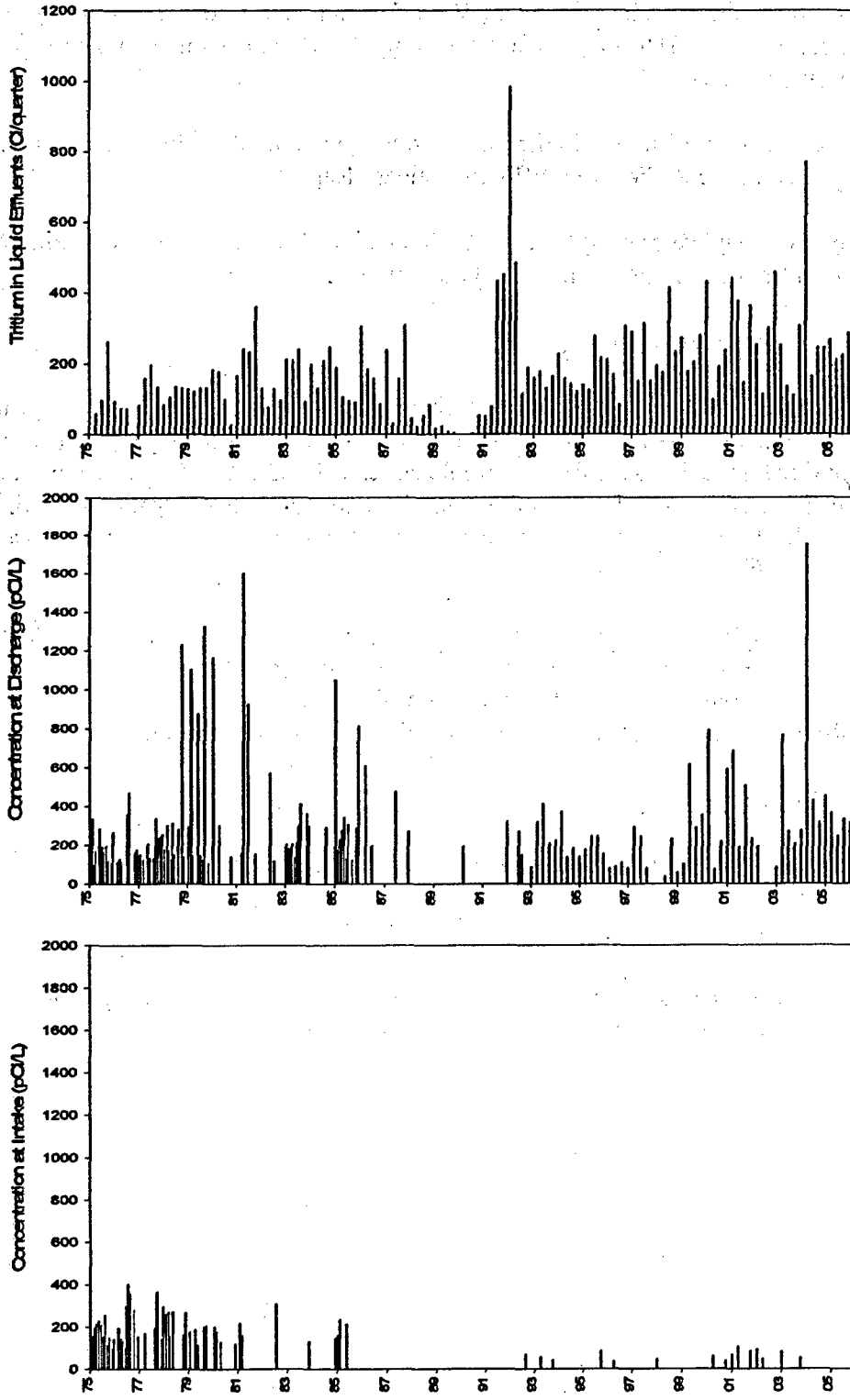
FIGURE 1 Tritium in Chesapeake Bay Water
