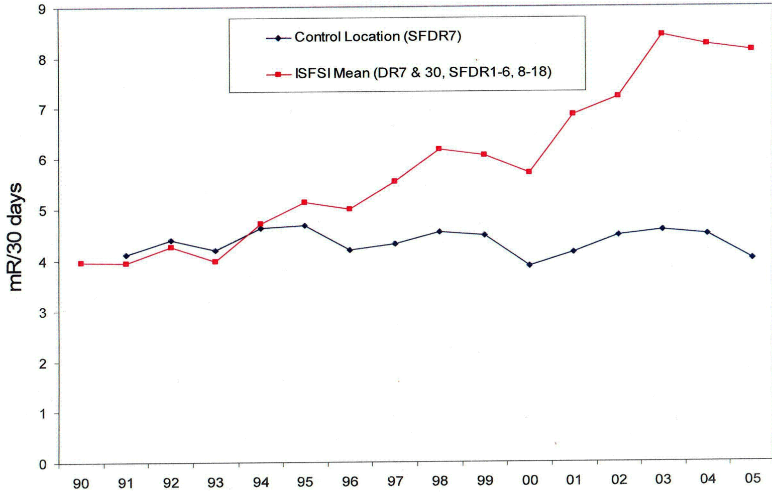
FIGURE 7 Mean TLD Gamma Dose, ISFSI
