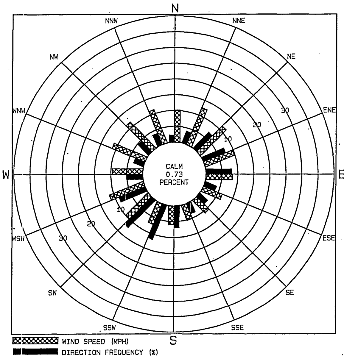
Figure 33 Wind Rose Annual Average 10M
