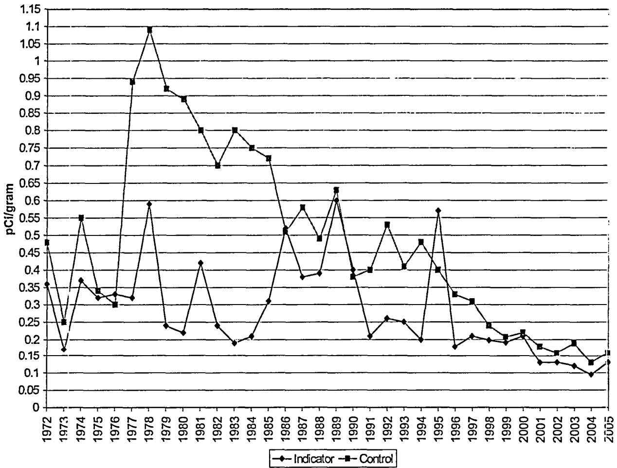
Figure 15: The concentration of Cesium-137 in soil has steadily declined in recent years. The peak seen in 1978 was due to fallout from nuclear weapons testing.
