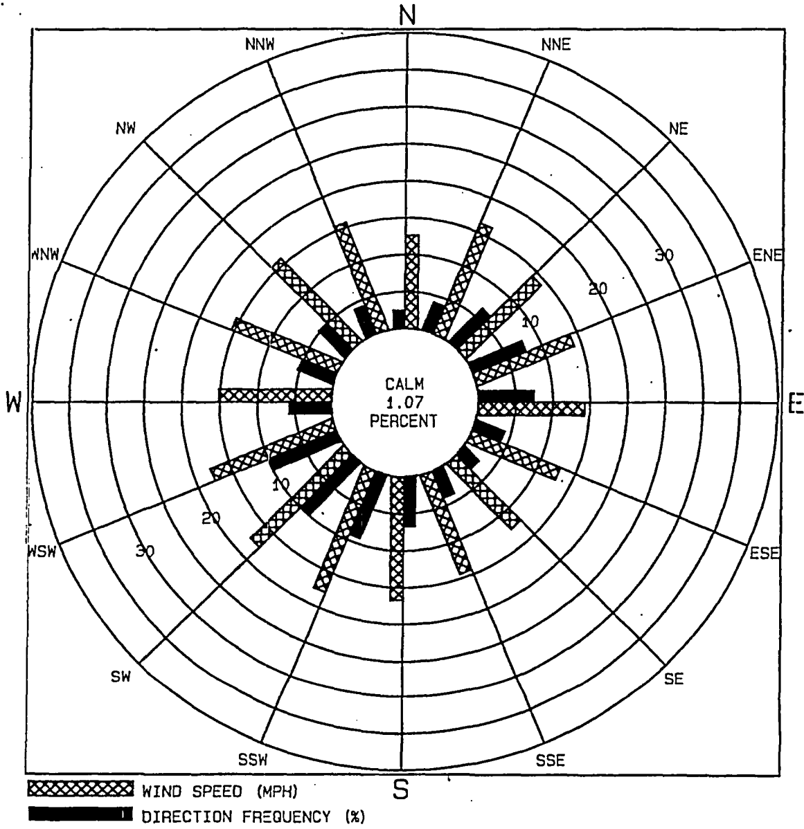
Figure 31 Wind Rose Annual Average 100M
