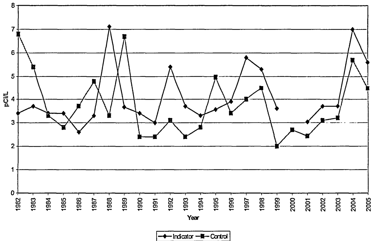
Figure 14: Shown above are the annual averages for gross beta in groundwater from 1982 - 2005. There were no known indicator samples available in 2000.
