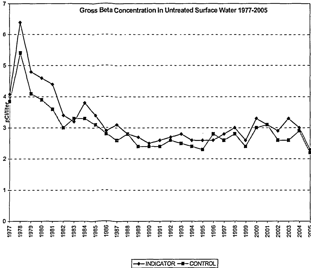
Figure 20: The average concentration of beta-emitting radionuclides in untreated water was similar between control and indicator locations. This demonstrates that Davis-Besse had no significant radiological impact on the surrounding environment.
