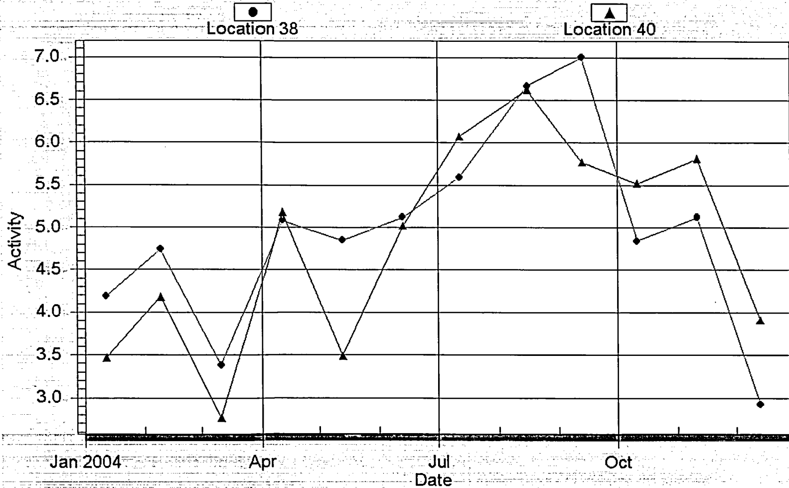
Figure 9 HNP From 1/1/2004 To 12/31/2004 DRINKING WATER for GROSS BETA - Activity (pCi/Liter)
