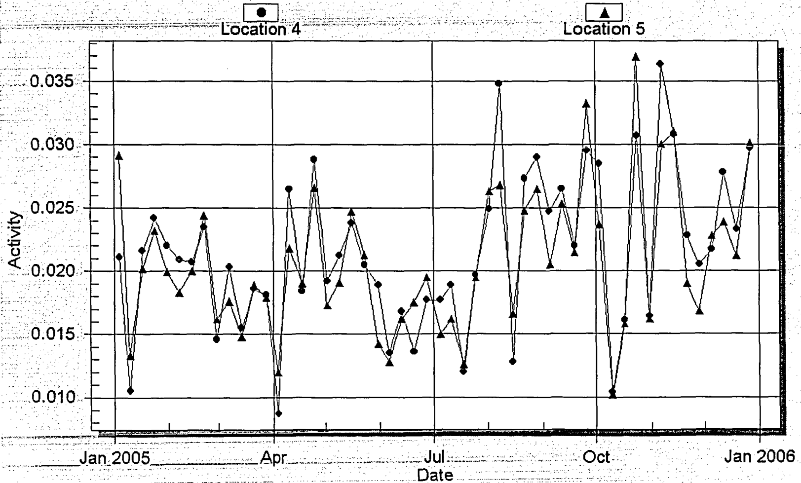
Figure 6 HNP From 1/1/2005 To 12/31/2005 AIR PARTICULATE for GROSS BETA - Activity (pCi/cubic meter)
