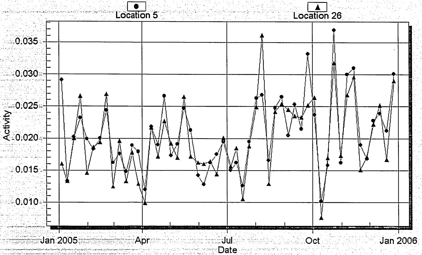
Figure 7 HNP From 1/1/2005 To 12/31/2005 AIR PARTICULATE for GROSS BETA - Activity (pCi/cubic meter)
