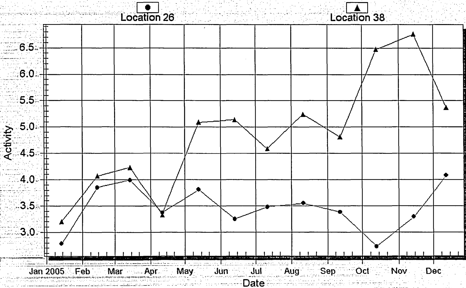
Figure 10 HNP From 1/1/2005 To 12/31/2005 SURFACE WATER for GROSS BETA - Activity (pCi/Liter)
